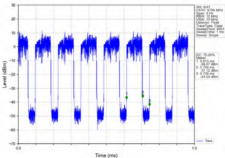
802.11ac(VHT40)_HCH_5795MHz_Ant1_NTNV
