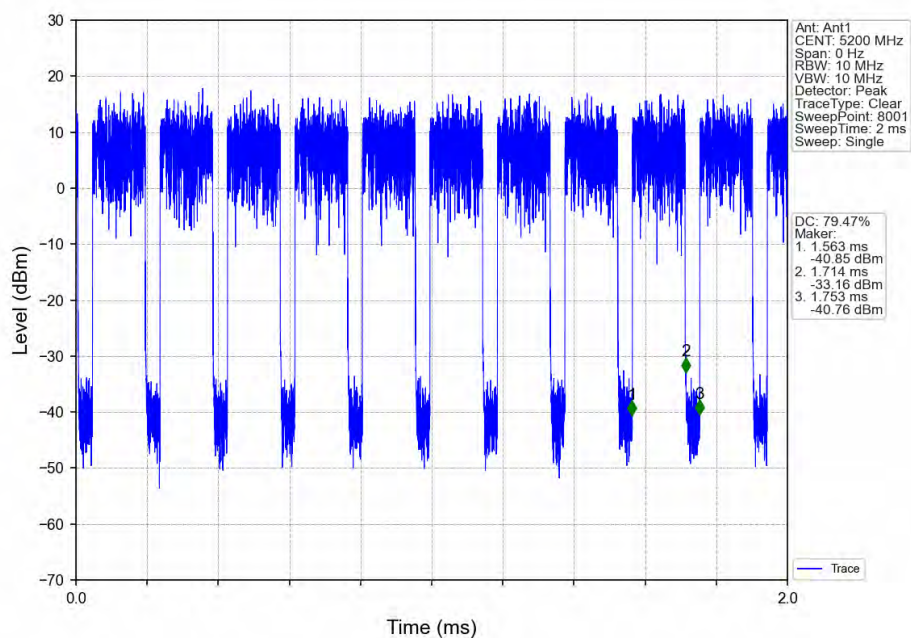
802.11ac(VHT20)_MCH_5200MHz_Ant1_NTNV
