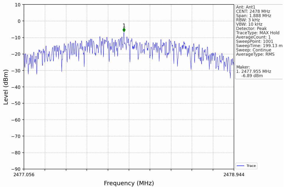
2M_HCH_2478MHz_Ant1_NTNV
