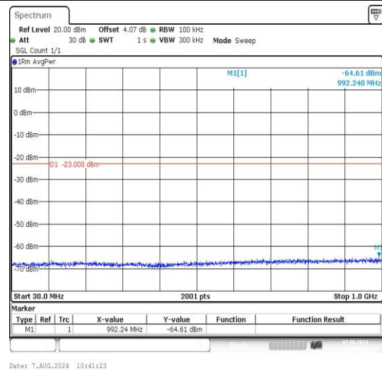
Band2_1.4MHz_16QAM_19193_1RB#0_30~1000_30~1000
