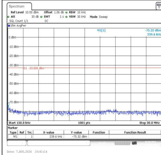
Band2_1.4MHz_16QAM_19193_1RB#0_0.15~30_0.15~30
