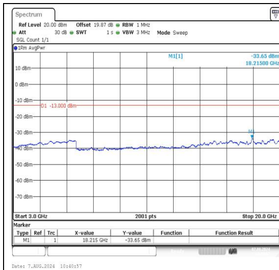
Band2_1.4MHz_QPSK_19193_1RB#0_3000~20000_3000~20000
