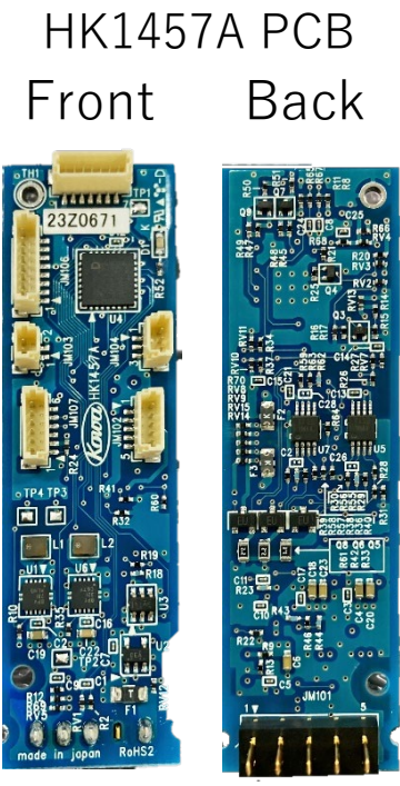
HK1457A PCB
