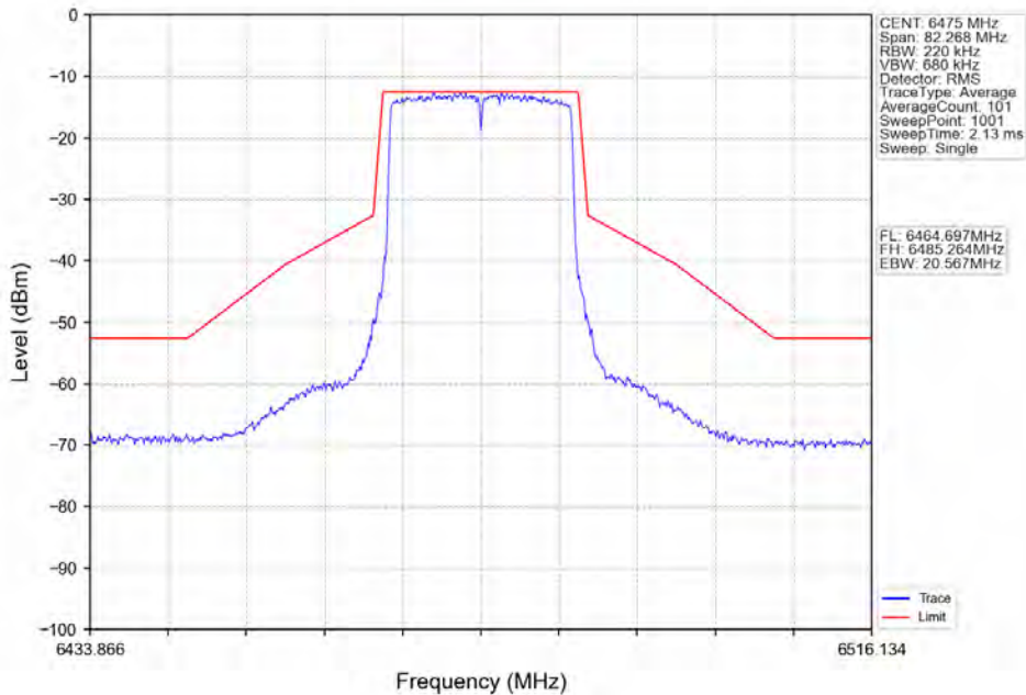
802.11ax(HE20)_MCH_6475MHz_RU242_Left_Ant2_NTNV
