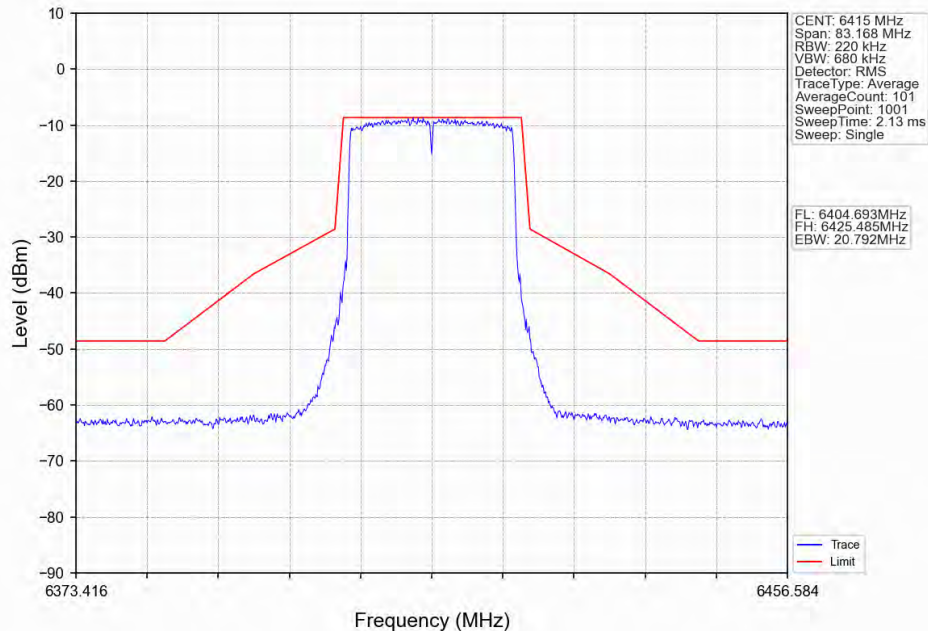
802.11ax(HE20)_HCH_6415MHz_RU242_Left_Ant2_NTNV
