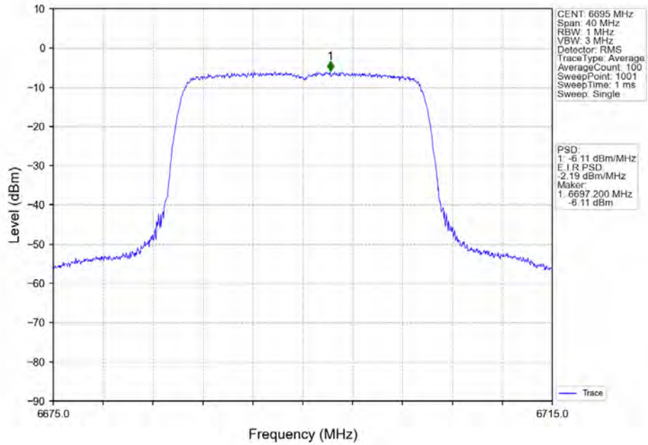
802.11ax(HE20)_MCH_6695MHz_RU242_Left_MIMO_NTNV
