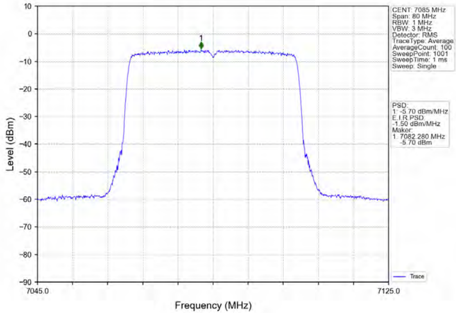
802.11ax(HE40)_HCH_7085MHz_RU484_Left_MIMO_NTNV
