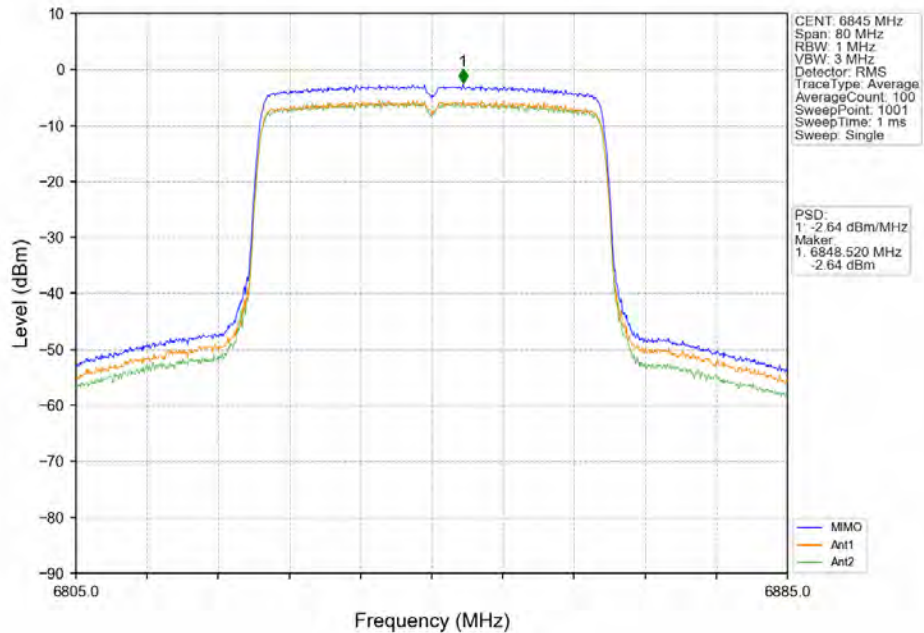
802.11ax(HE40)_HCH_6845MHz_RU484_Left_MIMO_NTNV
