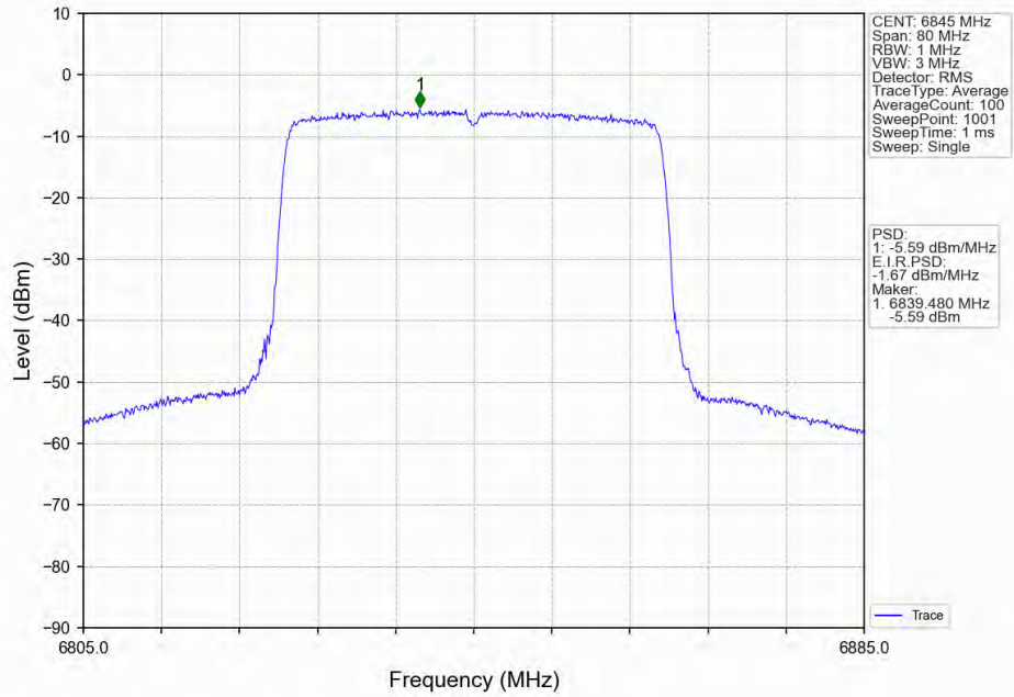
802.11ax(HE40)_HCH_6845MHz_RU484_Left_MIMO_NTNV
