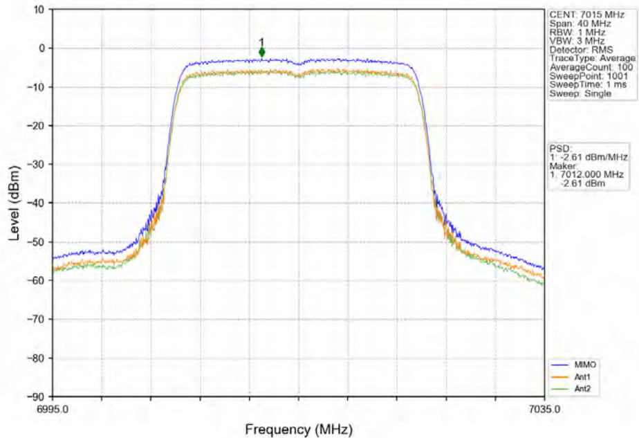
802.11ax(HE20)_MCH_7015MHz_RU242_Left_MIMO_NTNV
