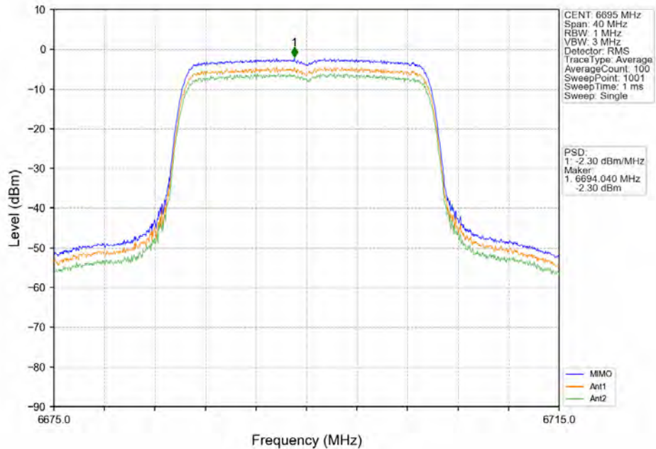
802.11ax(HE20)_MCH_6695MHz_RU242_Left_MIMO_NTNV
