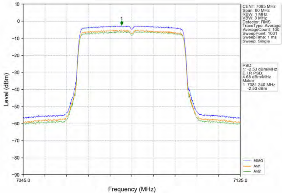
802.11ax(HE40)_HCH_7085MHz_RU484_Left_MIMO_NTNV
