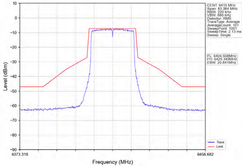
802.11ax(HE20)_HCH_6415MHz_RU242_Left_Ant2_NTNV
