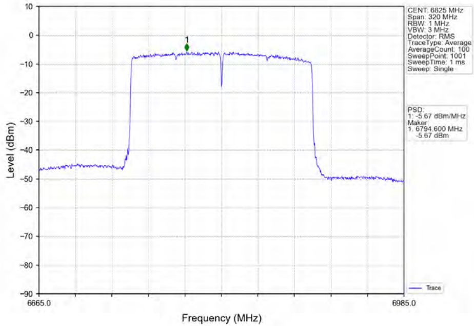
802.11ax(HE160)_HCH_6825MHz_2xRU996_Left_MIMO_NTNV
