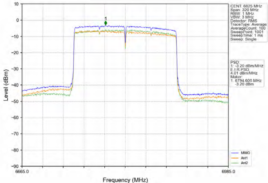
802.11ax(HE160)_HCH_6825MHz_2xRU996_Left_MIMO_NTNV
