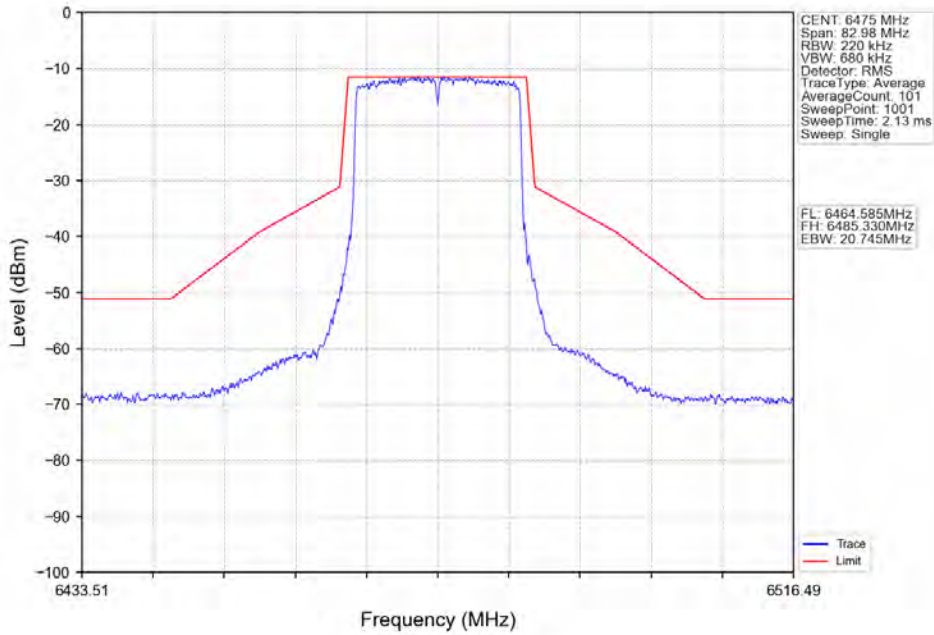
802.11ax(HE20)_MCH_6475MHz_RU242_Left_Ant2_NTNV
