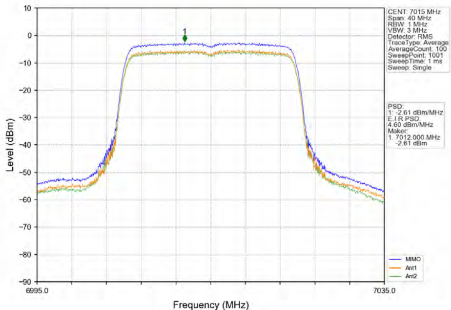
802.11ax(HE20)_MCH_7015MHz_RU242_Left_MIMO_NTNV
