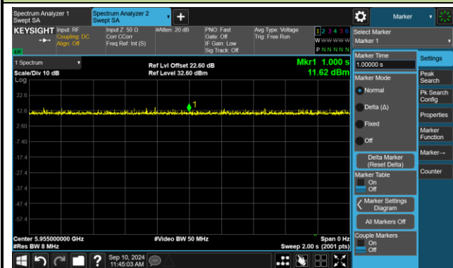
802.11be-EHT80 (T = 1.0s)
