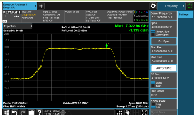
Channel 213 (7015MHz)
