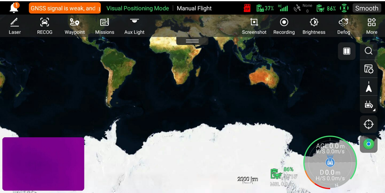
Fig 6-12 "Map" Interface
