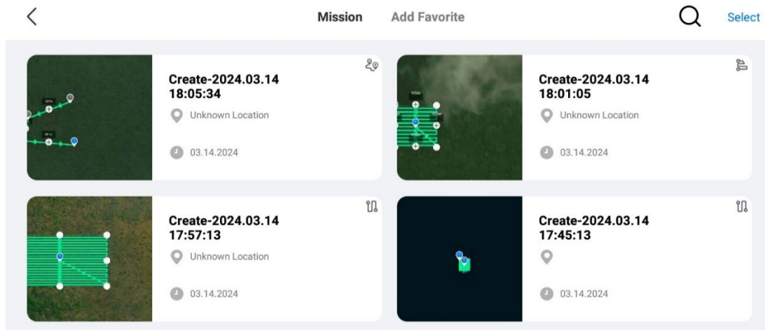
Fig 6-20 Mission/Favorites Interface
