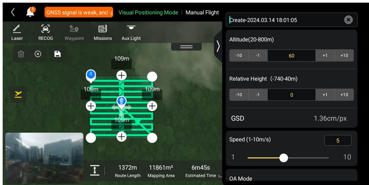
Fig 6-18 Polygon
