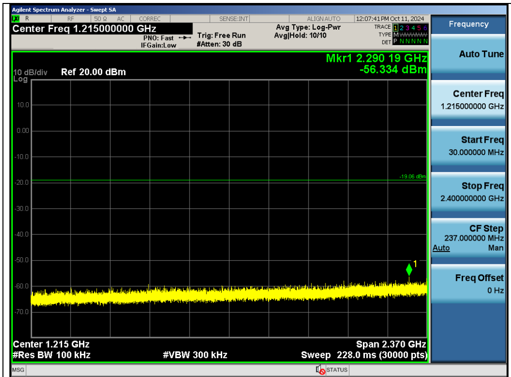
Test_Graph_GFSK_ANT1_2444.5_Lower Band Emissions
