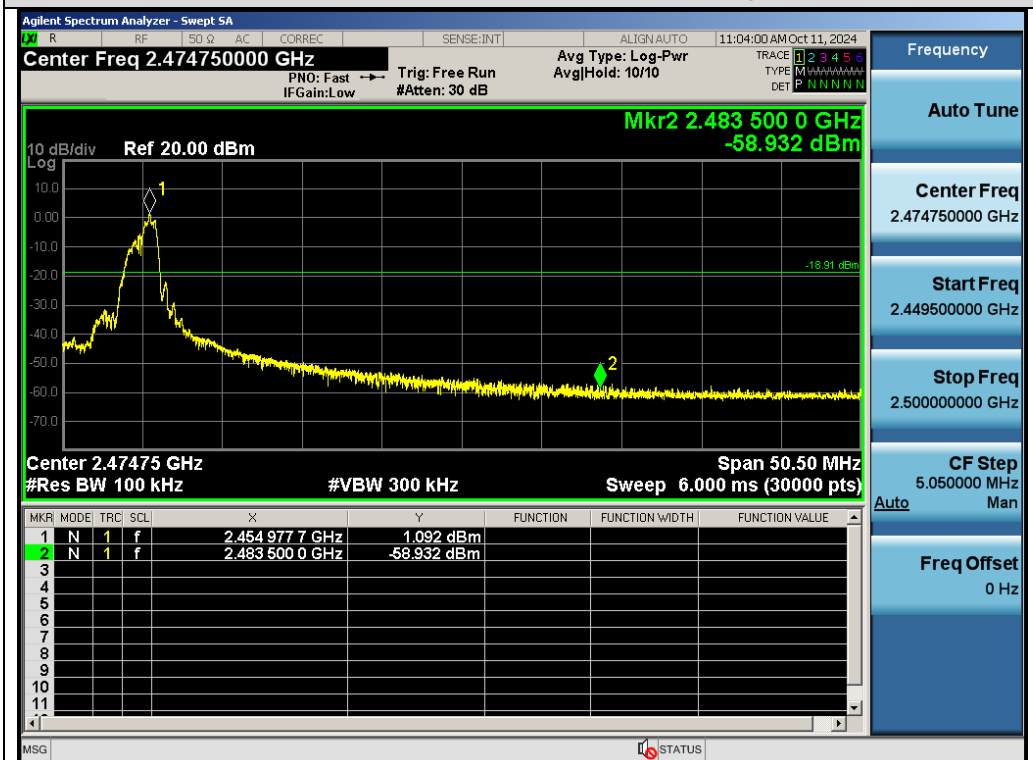
Test_Graph_GFSK_ANT1_2455_Higher Band Edge Emissions
