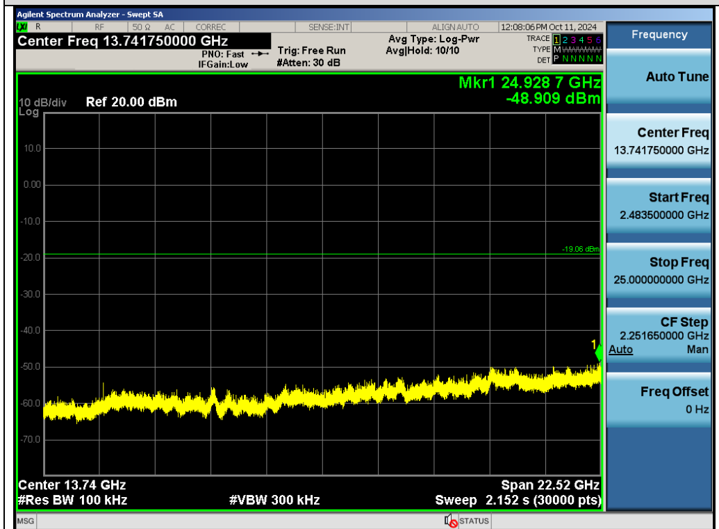
Test_Graph_GFSK_ANT1_2444.5_Higher Band Emissions
