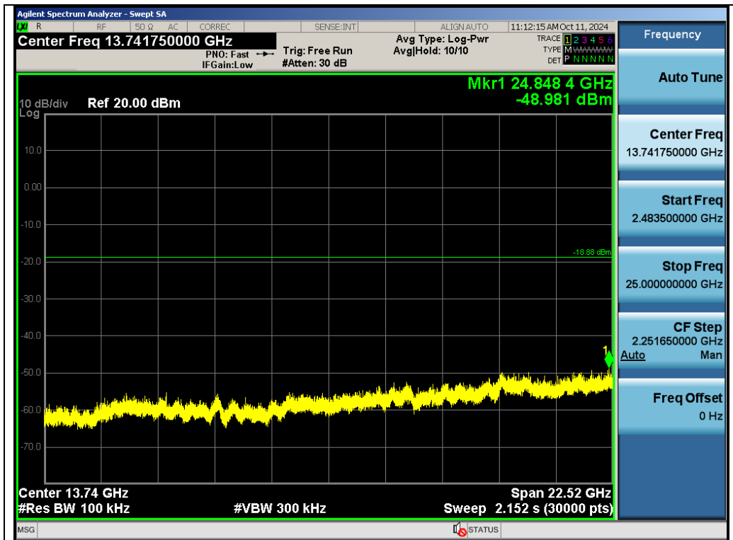
Test_Graph_GFSK_ANT1_2434.5_Higher Band Emissions
