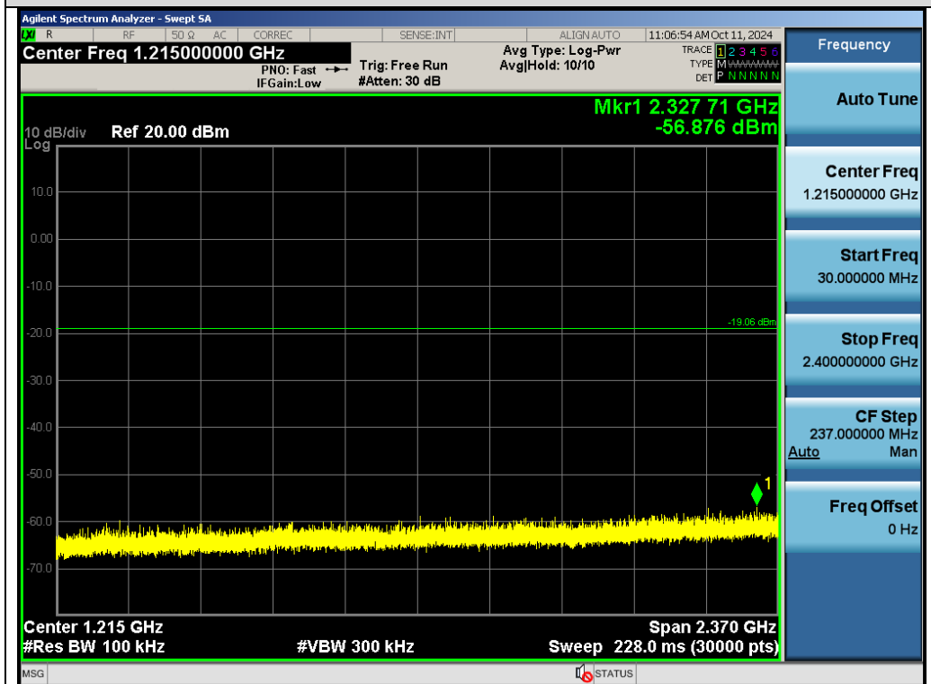
Test_Graph_GFSK_ANT1_2454.5_Lower Band Emissions
