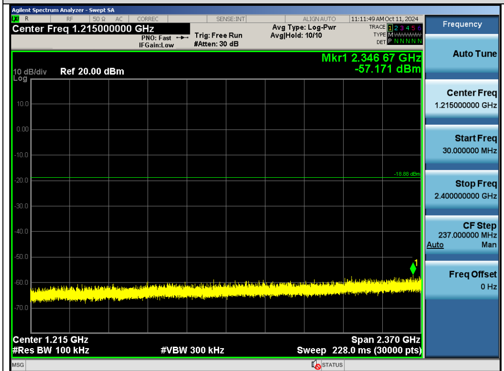
Test_Graph_GFSK_ANT1_2434.5_Lower Band Emissions
