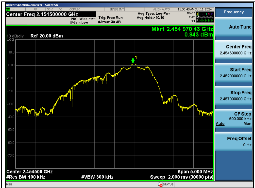
Test_Graph_GFSK_ANT1_2454.5_Reference Level
