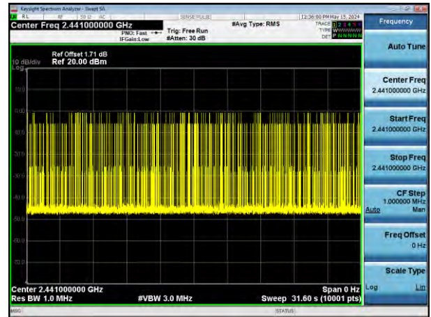
Accumulate(3DH5)
