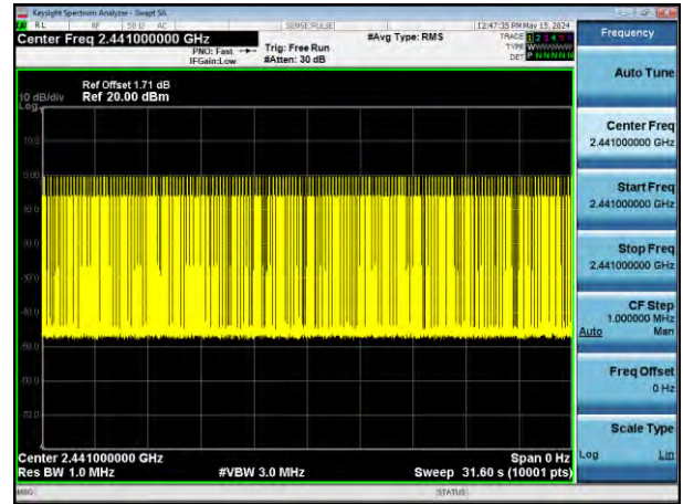
Accumulate(3DH1)
