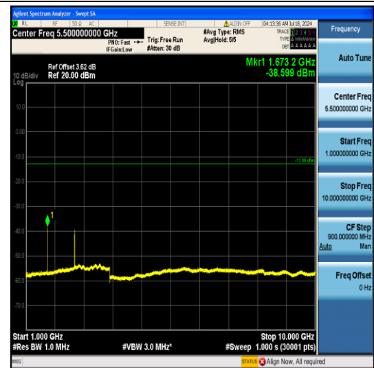
1GHz ~10GHz
