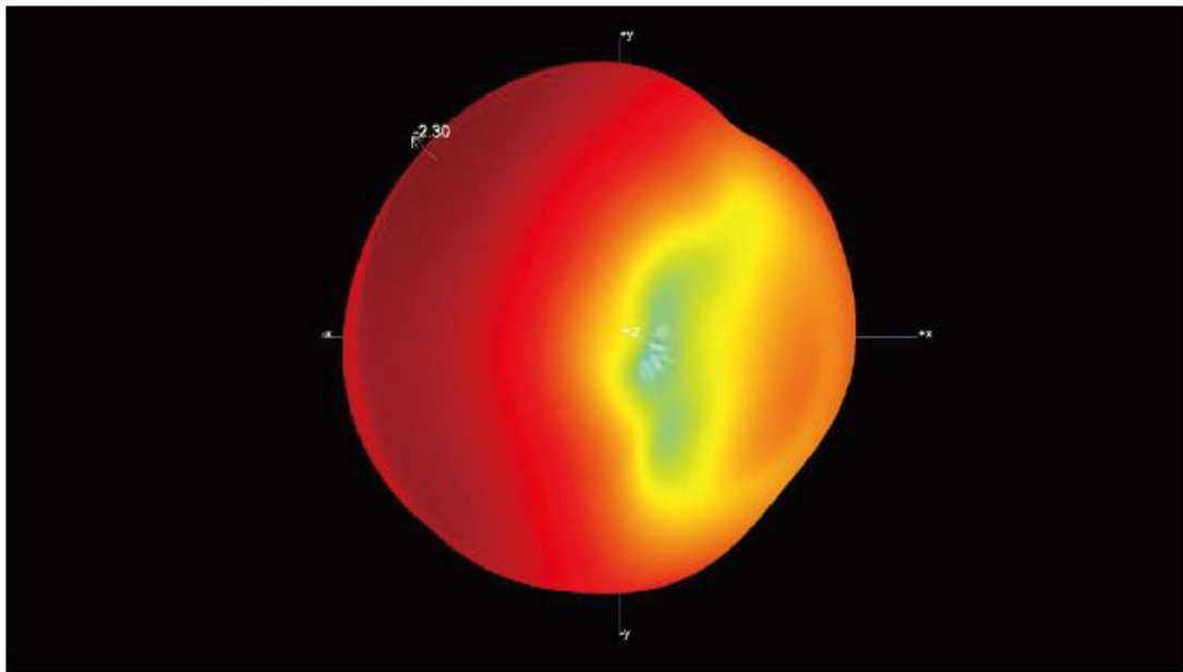
B1.1 3D Pattern for 2400MHz
