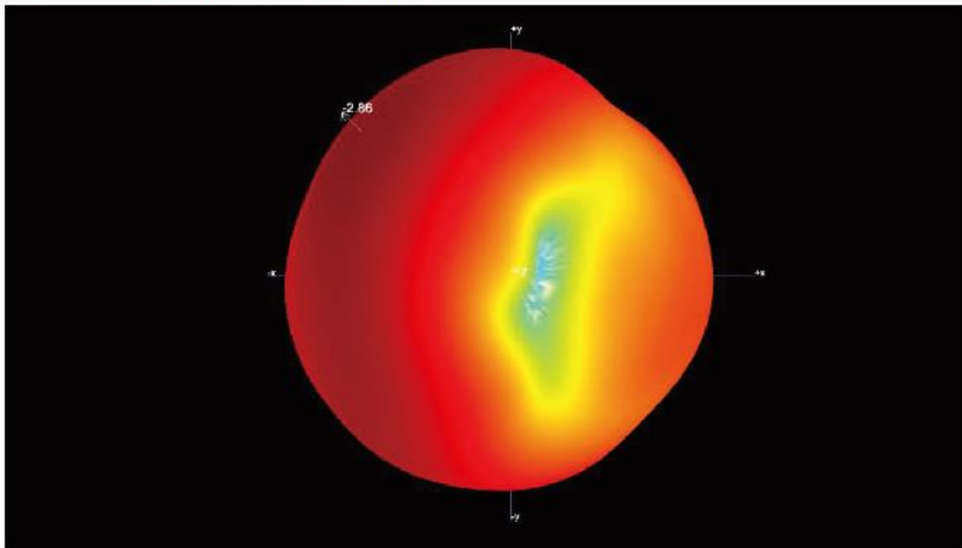
B1.2 3D Pattern for 2450MHz
