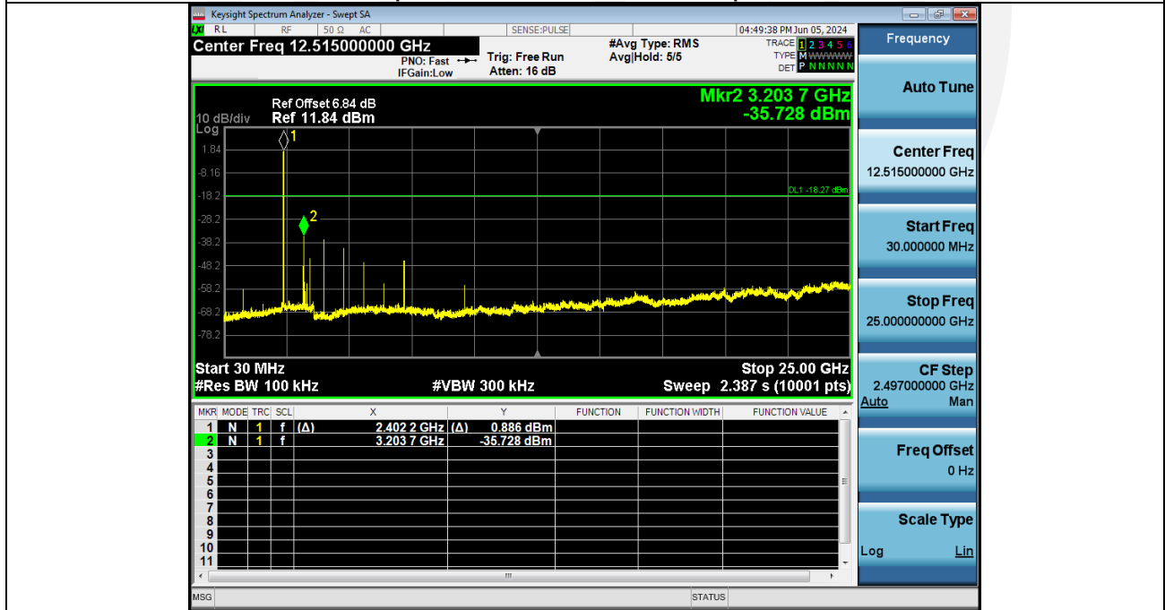
2_Spurious Emission_NVNT_ANT1_1Mbps_2402
