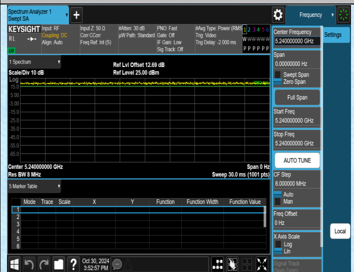
NTNV-11N20SISO-Ant2-5240
