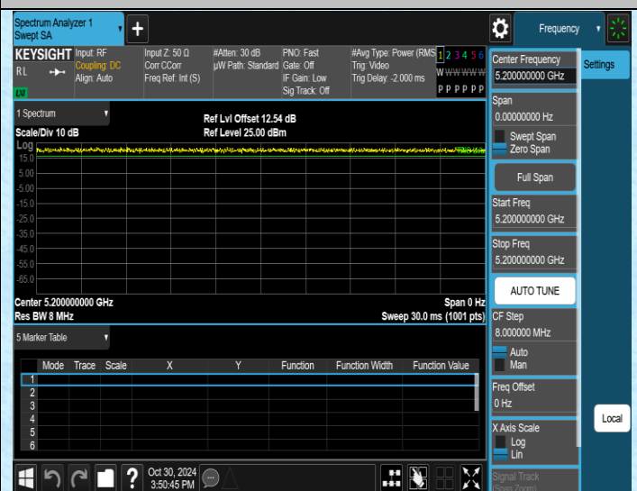
NTNV-11N20SISO-Ant2-5200
