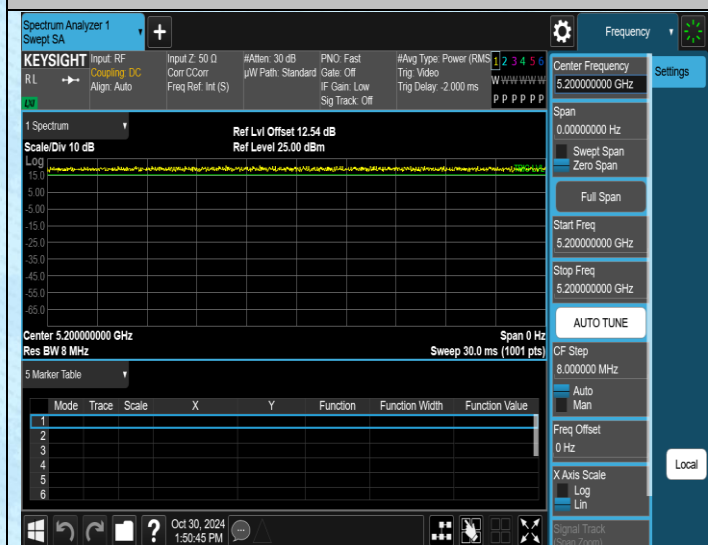
NTNV-11N20SISO-Ant1-5200
