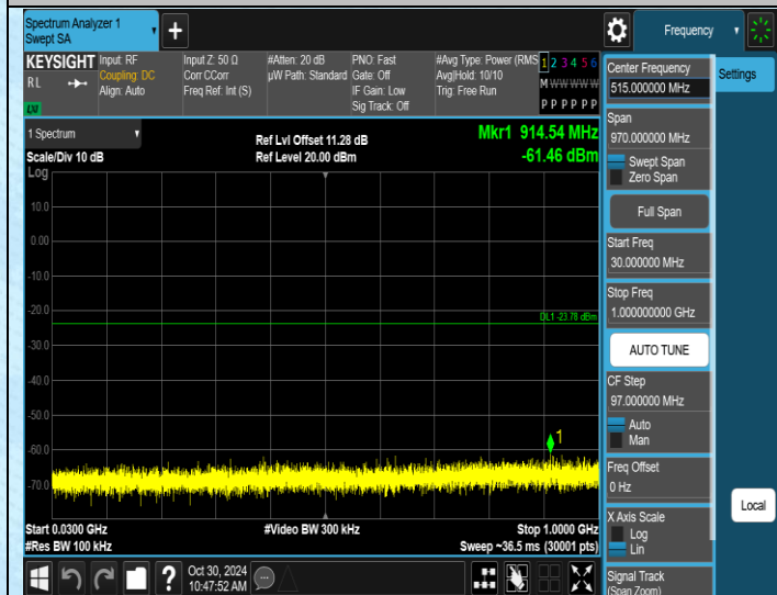
11G-Ant2-2412-30~1000-PASS
