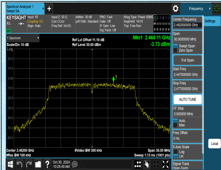
11G-Ant1-2462-0~Reference-PASS
