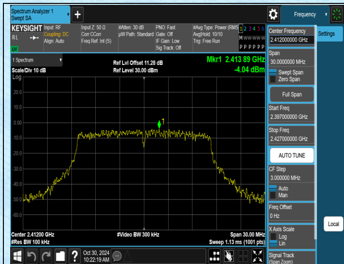
11G-Ant1-2412-0~Reference-PASS
