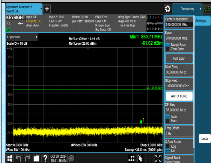
11G-Ant2-2462-30~1000-PASS
