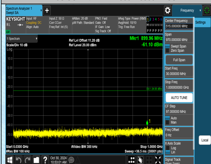
11N20SISO-Ant2-2412-30~1000-PASS
