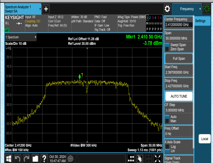
11G-Ant2-2412-0~Reference-PASS
