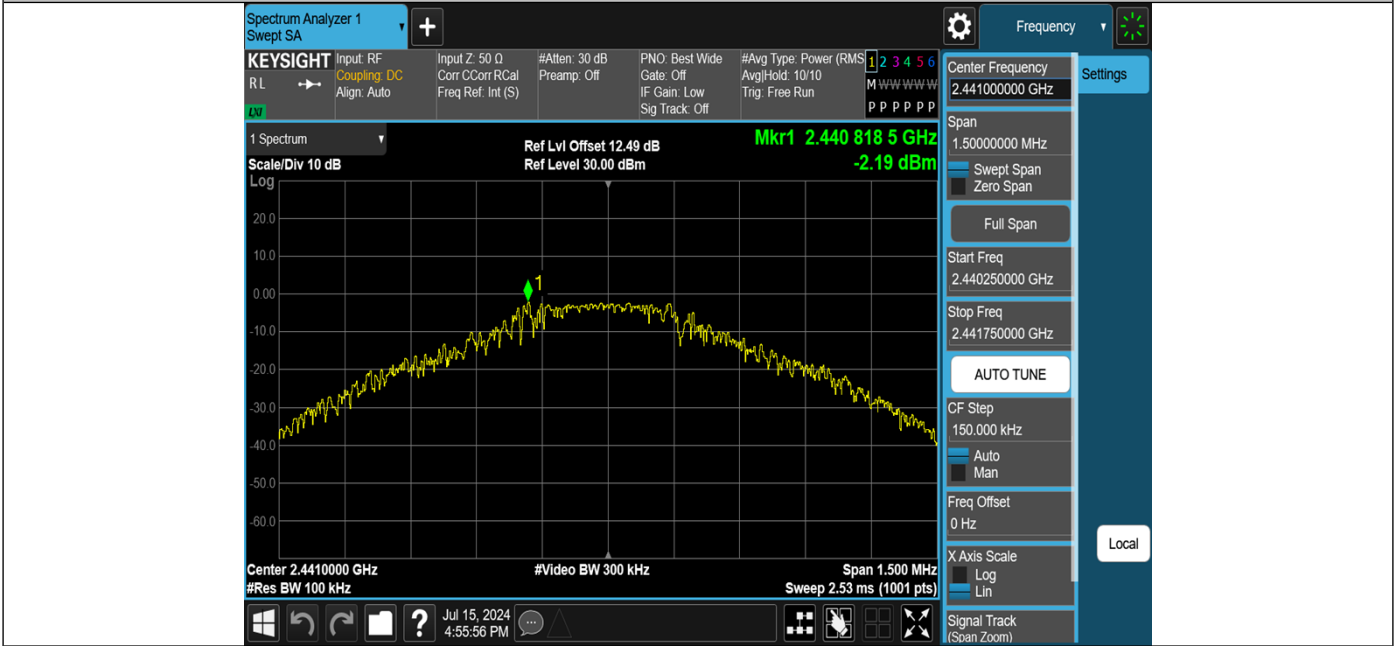
DH5-Ant1-2441-0~Reference-PASS
