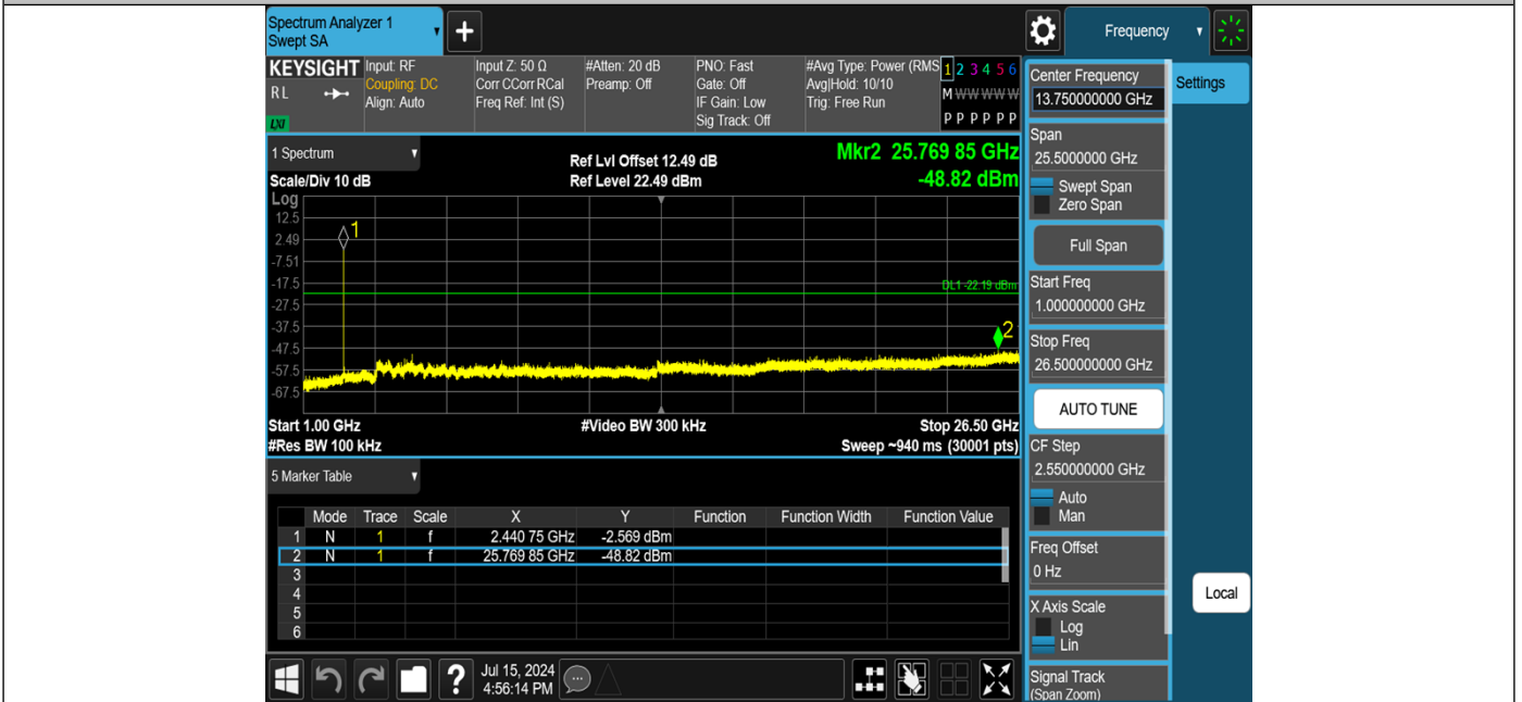
DH5-Ant1-2441-1000~26500-PASS
