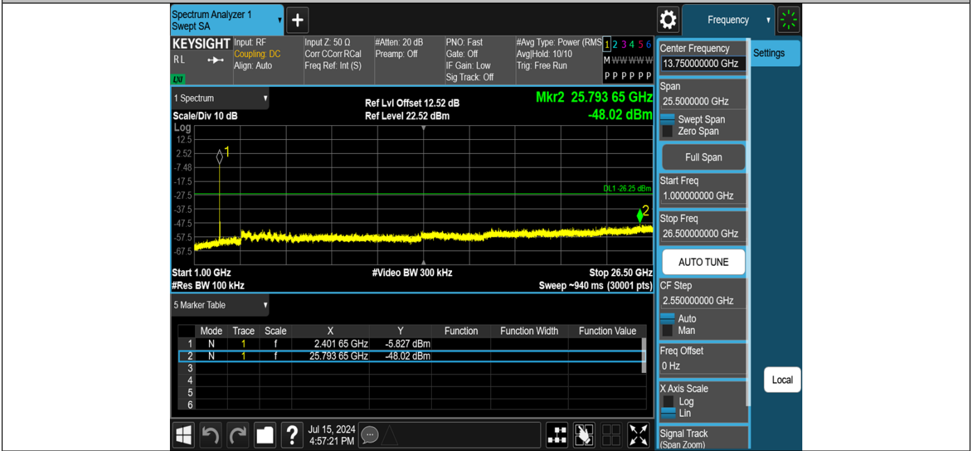
2DH5-Ant1-2402-1000~26500-PASS
