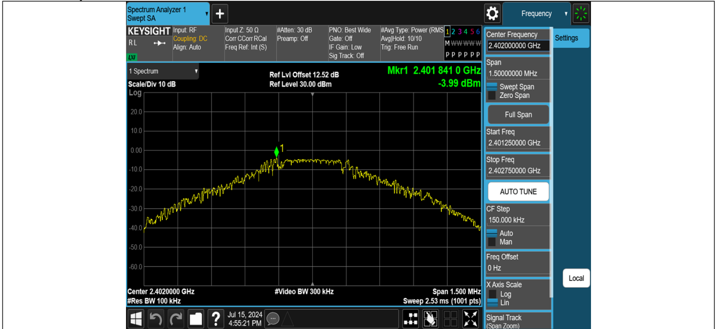
DH5-Ant1-2402-0~Reference-PASS
