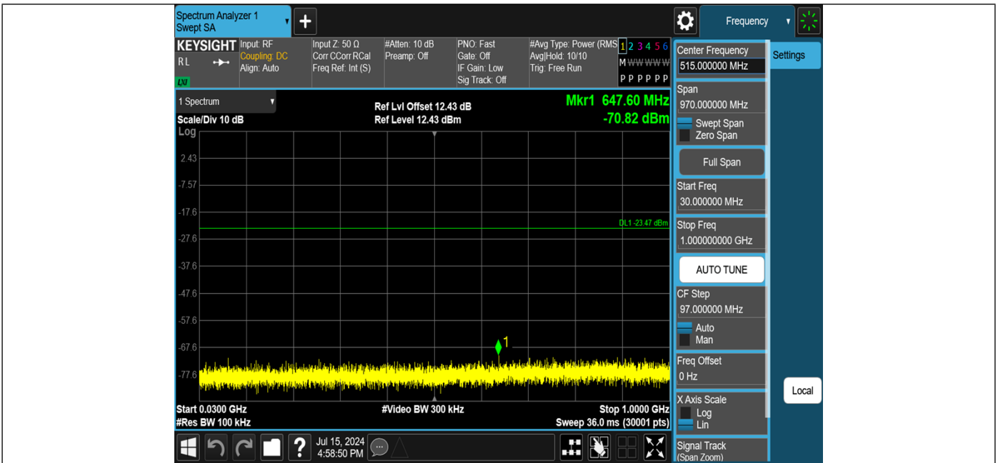
2DH5-Ant1-2480-30~1000-PASS
