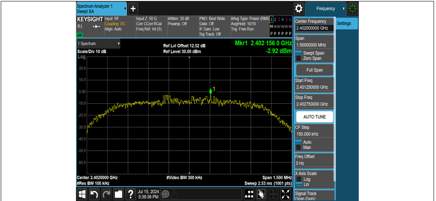
3DH5-Ant1-2402-0~Reference-PASS
