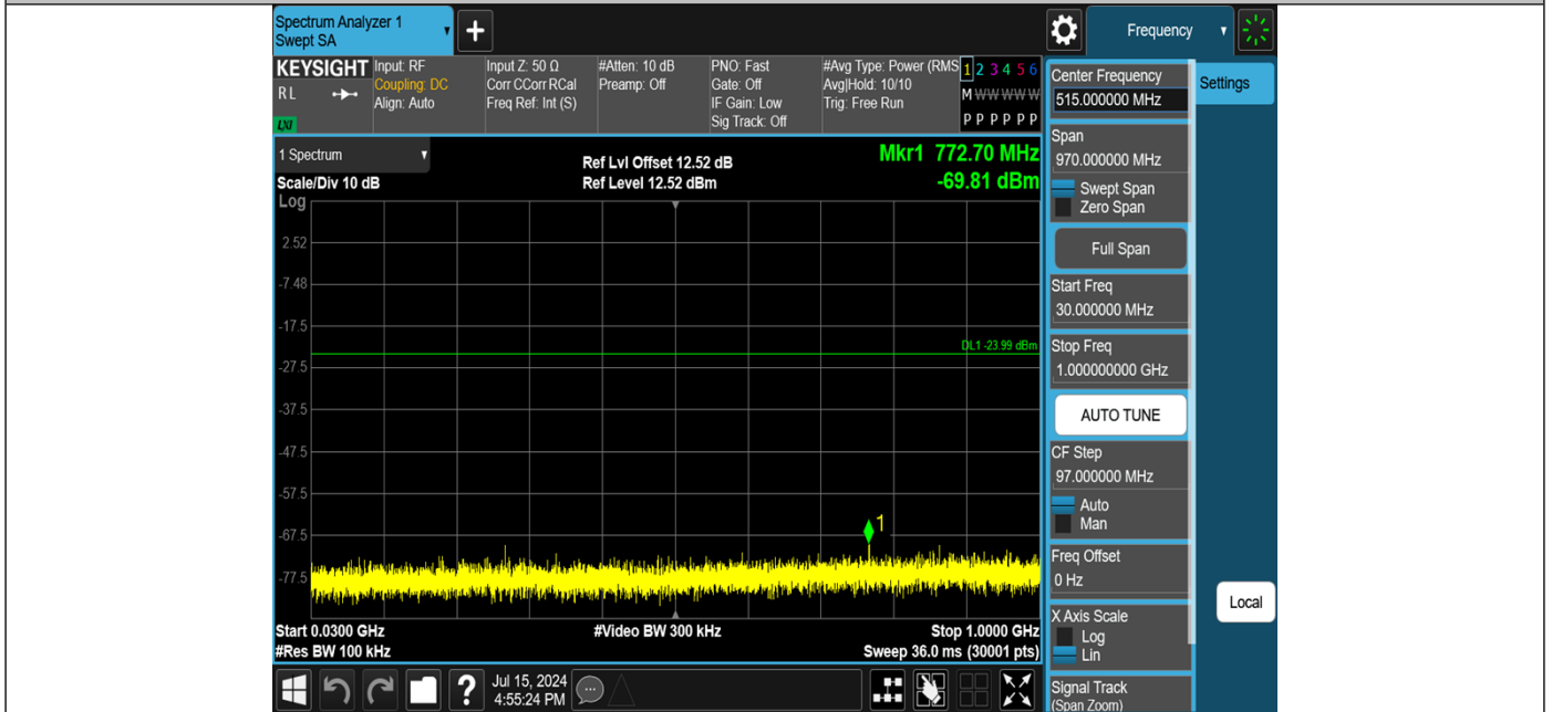
DH5-Ant1-2402-30~1000-PASS
