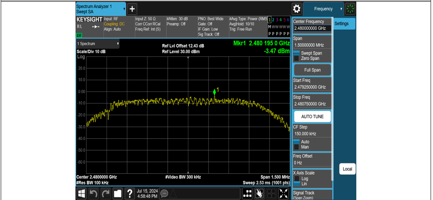
2DH5-Ant1-2480-0~Reference-PASS
