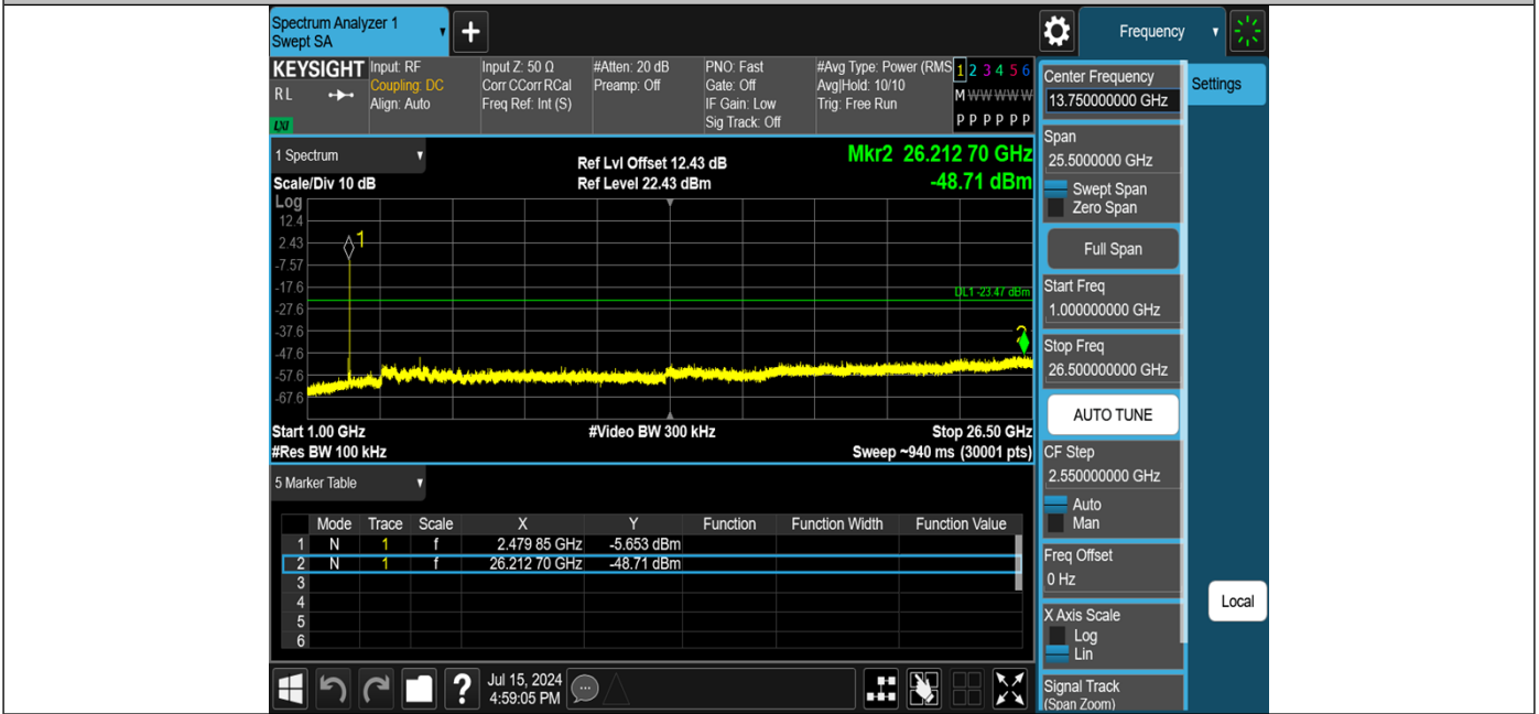
2DH5-Ant1-2480-1000~26500-PASS
