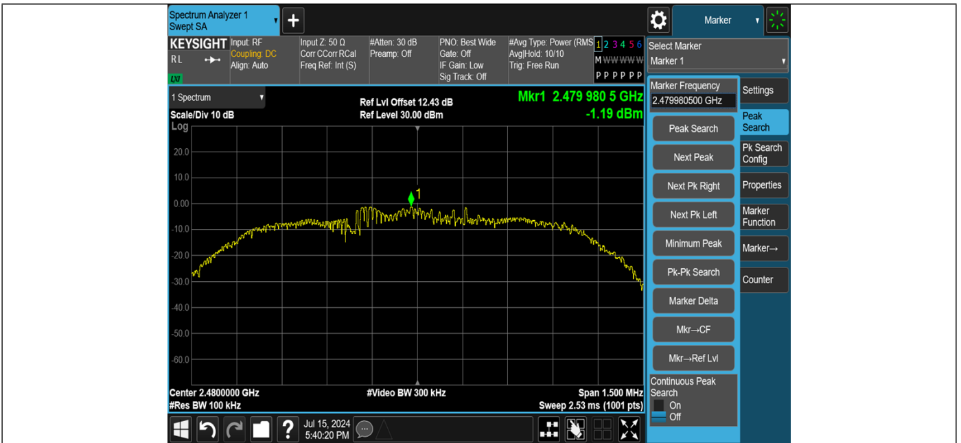
3DH5-Ant1-2480-0~Reference-PASS
