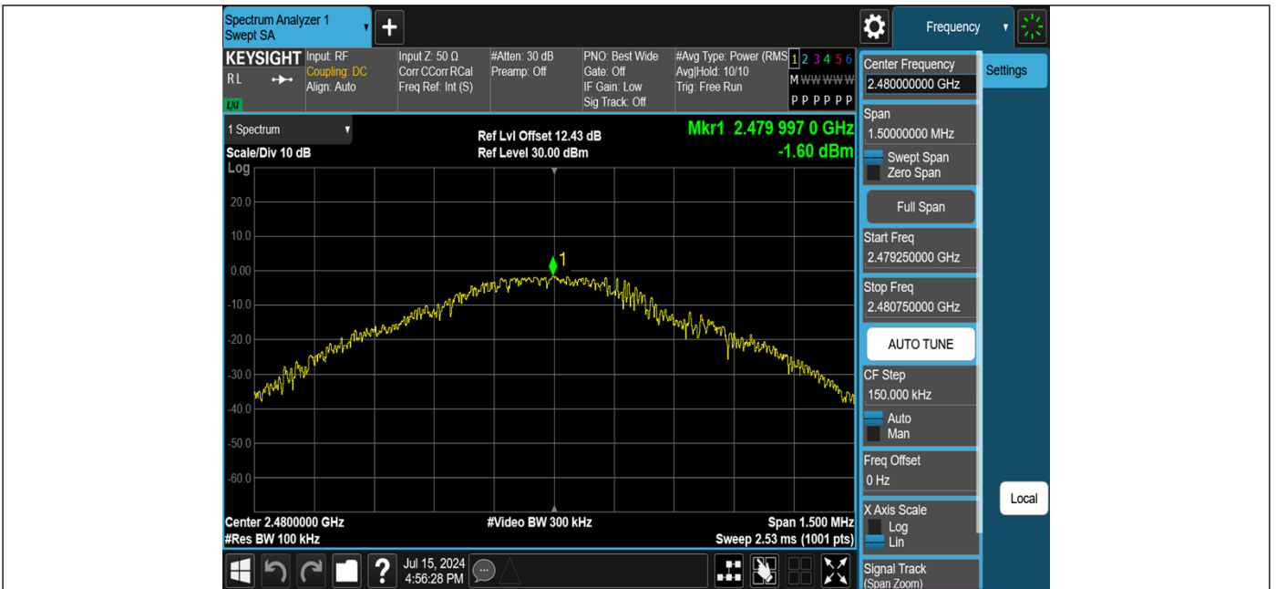
DH5-Ant1-2480-0~Reference-PASS
