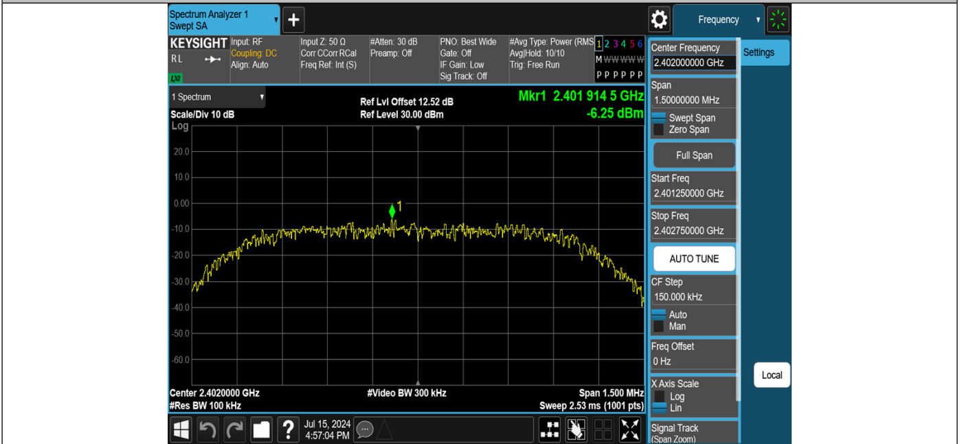
2DH5-Ant1-2402-0~Reference-PASS
