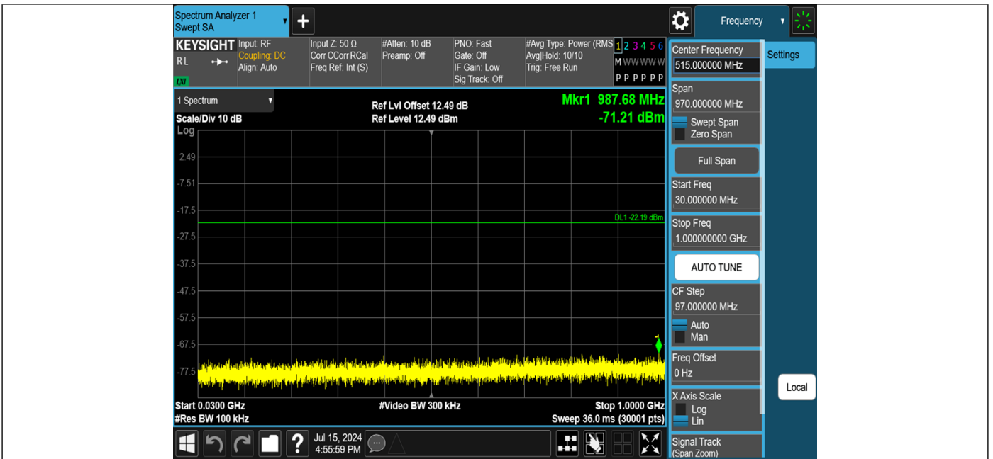
DH5-Ant1-2441-30~1000-PASS
