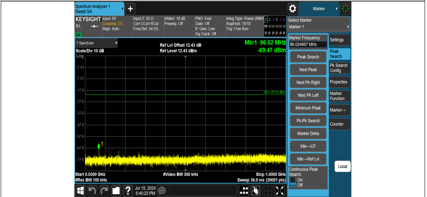
3DH5-Ant1-2480-30~1000-PASS
