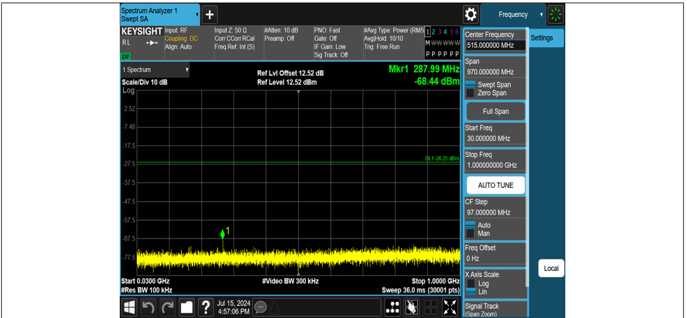
2DH5-Ant1-2402-30~1000-PASS
