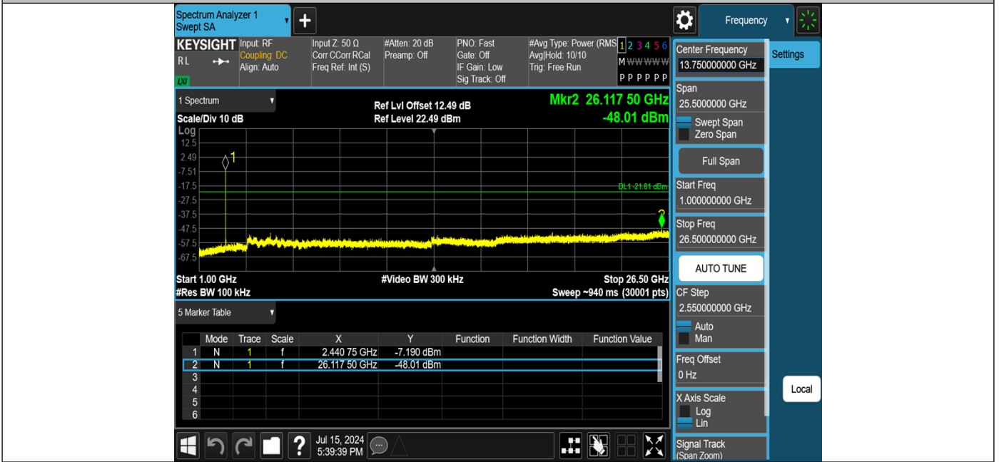
3DH5-Ant1-2441-1000~26500-PASS
