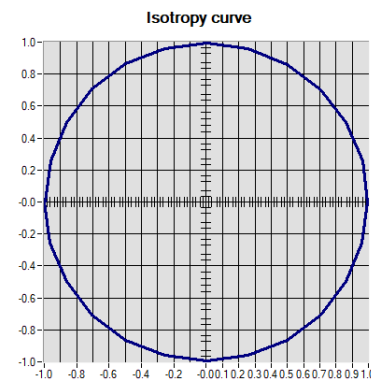
Isotropy: +/-0.26% (+/-0.01dB)
