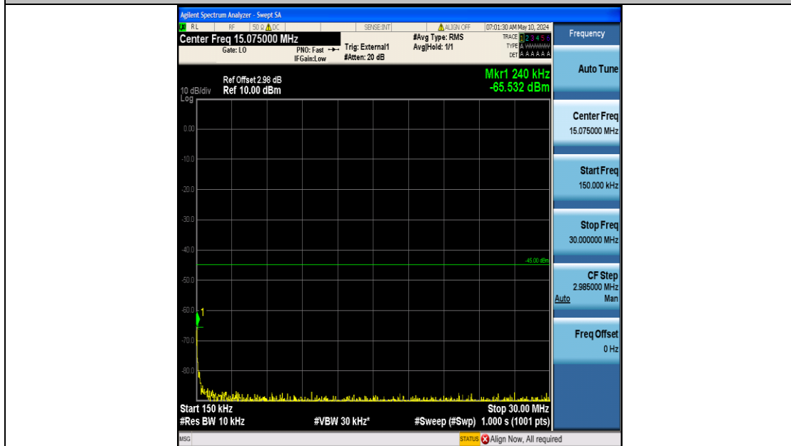
Band41_10MHz_QPSK_39700_50RB#0_0.15~30_0.15~30
