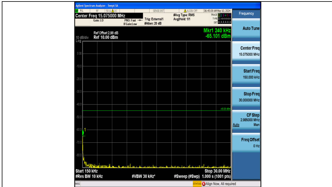
Band41_5MHz_16QAM_39675_25RB#0_0.15~30_0.15~30
