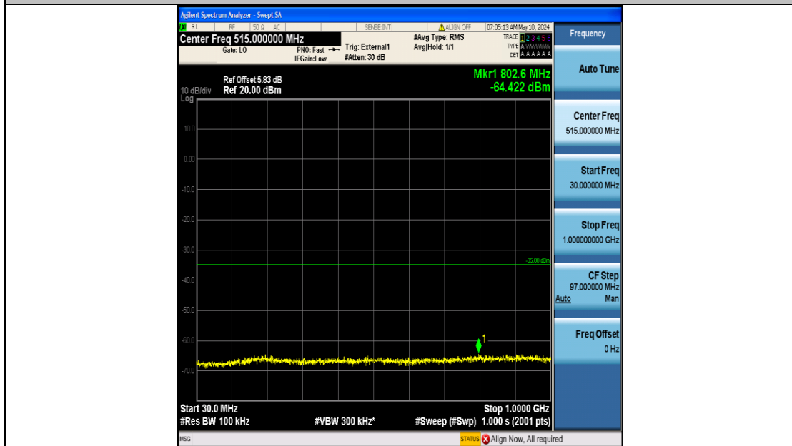
Band41_10MHz_QPSK_40620_50RB#0_30~1000_30~1000
