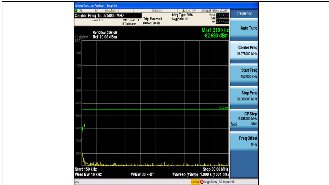
Band41_15MHz_16QAM_39725_75RB#0_0.15~30_0.15~30
