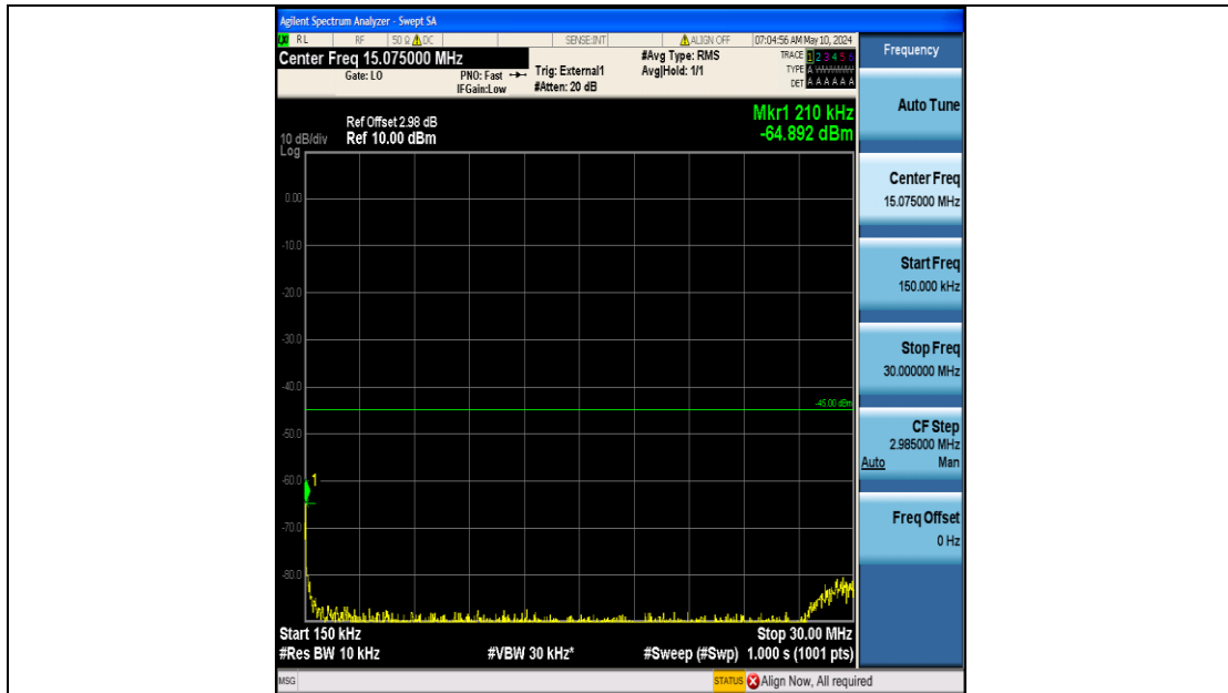
Band41_10MHz_QPSK_40620_50RB#0_0.15~30_0.15~30
