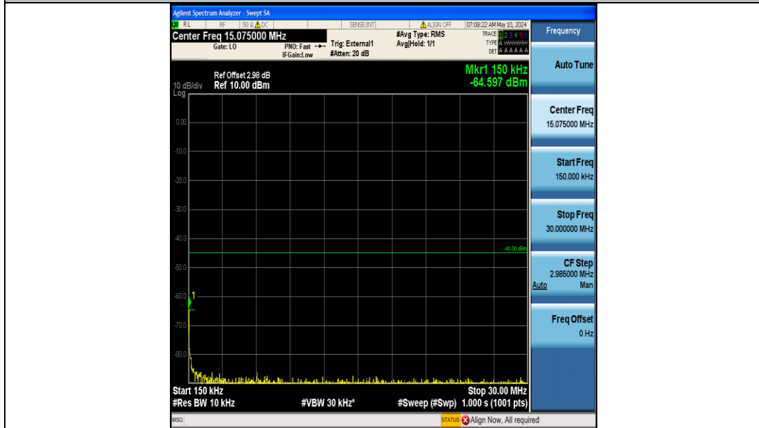
Band41_10MHz_QPSK_41540_50RB#0_0.15~30_0.15~30
