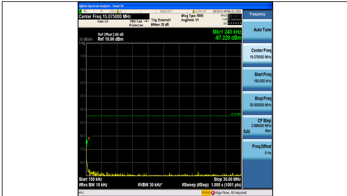
Band41_5MHz_16QAM_41565_25RB#0_0.15~30_0.15~30
