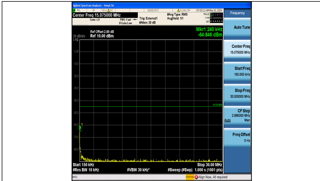
Band41_10MHz_16QAM_39700_50RB#0_0.15~30_0.15~30
