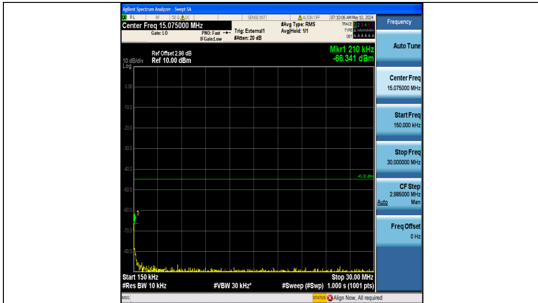
Band41_10MHz_16QAM_41540_50RB#0_0.15~30_0.15~30
