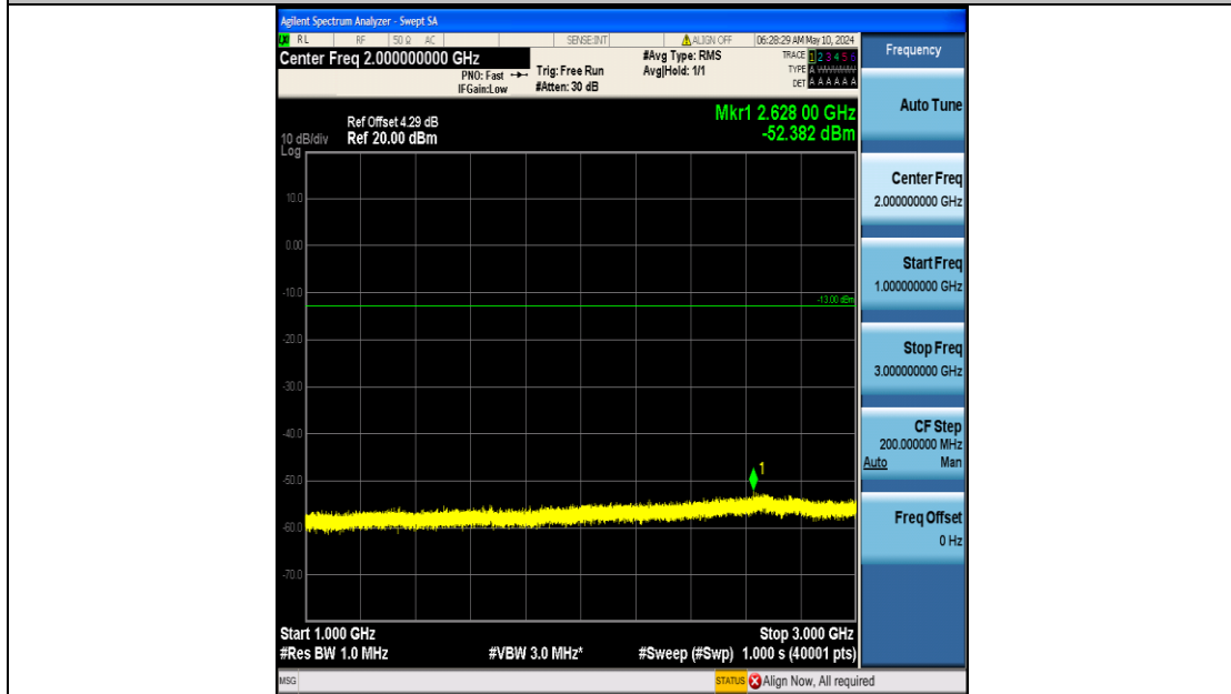
Band26_15MHz_16QAM_26915_75RB#0_1000~3000_1000~3000
