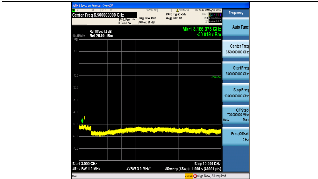
Band26_15MHz_16QAM_26915_75RB#0_3000~10000_3000~10000
