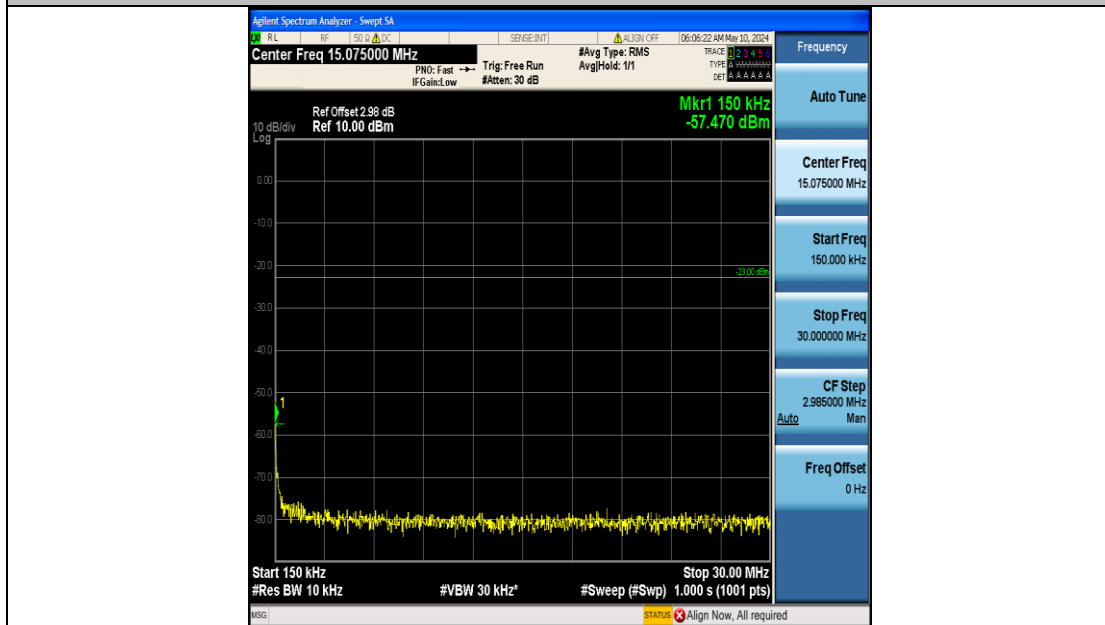
Band26_5MHz_16QAM_26915_25RB#0_0.15~30_0.15~30
