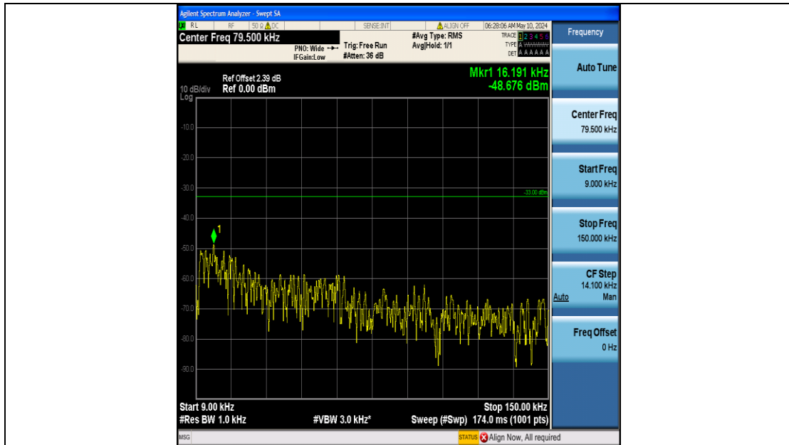
Band26_15MHz_16QAM_26915_75RB#0_0.009~0.15_0.009~0.15
