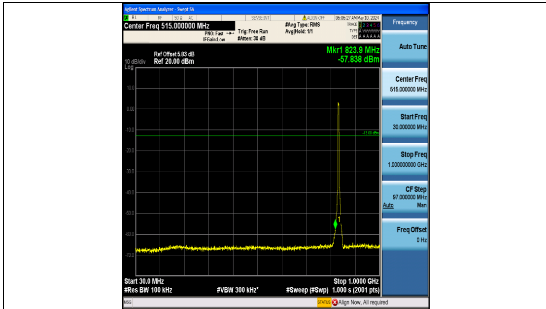
Band26_5MHz_16QAM_26915_25RB#0_30~1000_30~1000
