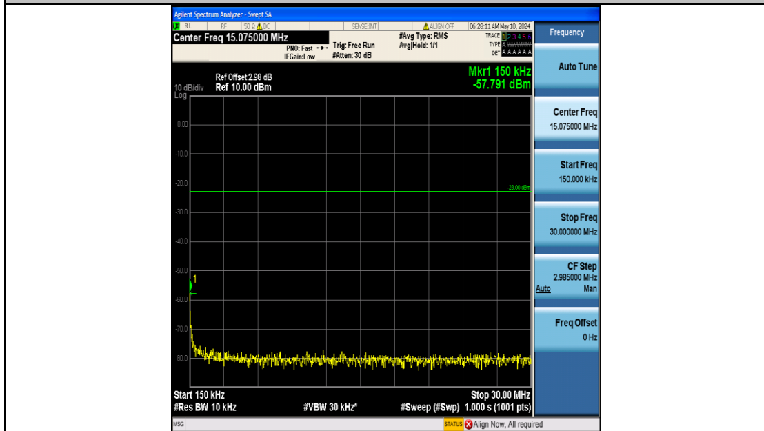
Band26_15MHz_16QAM_26915_75RB#0_0.15~30_0.15~30
