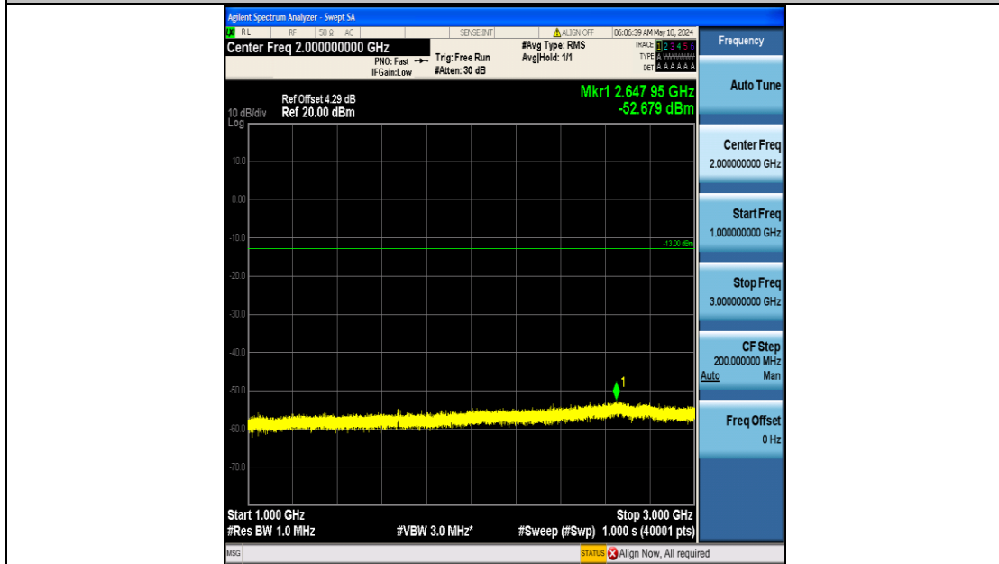
Band26_5MHz_16QAM_26915_25RB#0_1000~3000_1000~3000
