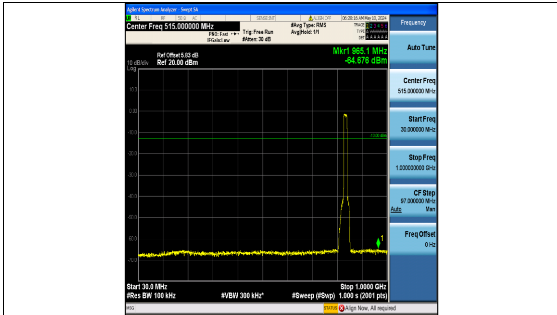
Band26_15MHz_16QAM_26915_75RB#0_30~1000_30~1000
