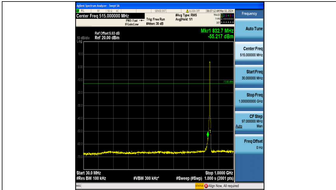
Band26_5MHz_QPSK_27015_25RB#0_30~1000_30~1000
