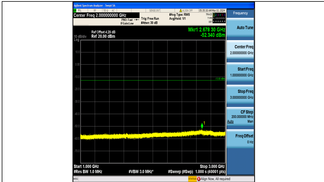
Band26_10MHz_16QAM_26740_50RB#0_1000~3000_1000~3000
