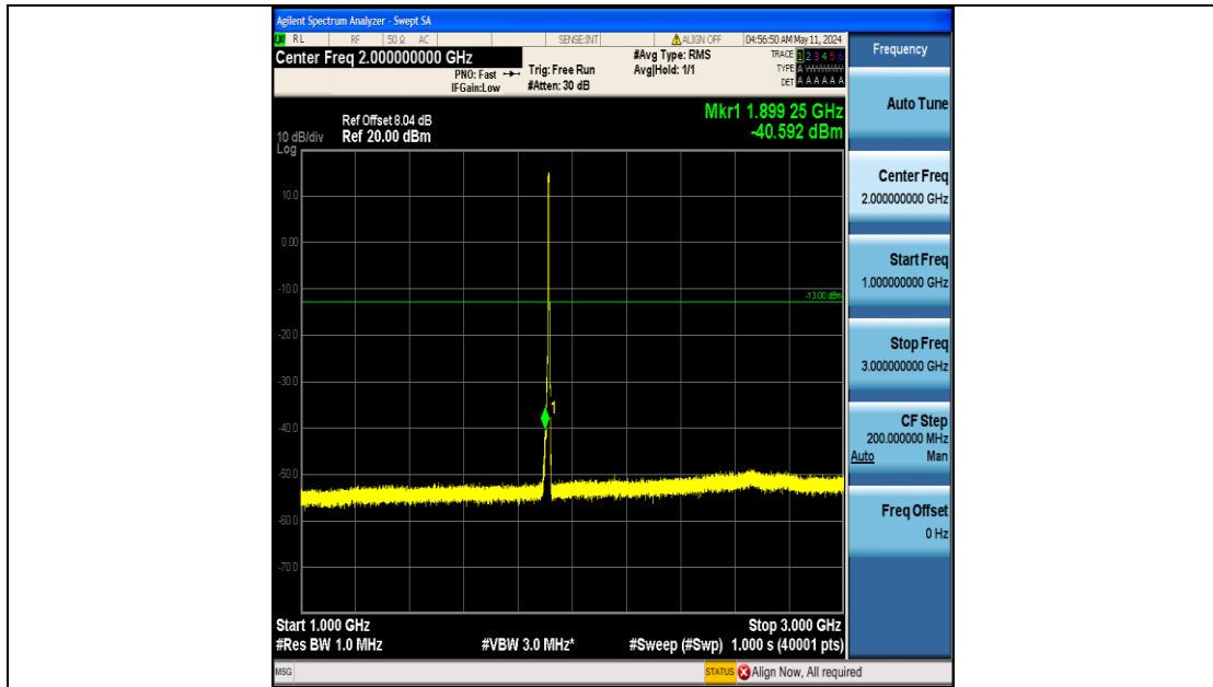
Band25_5MHz_QPSK_26665_25RB#0_1000~3000_1000~3000
