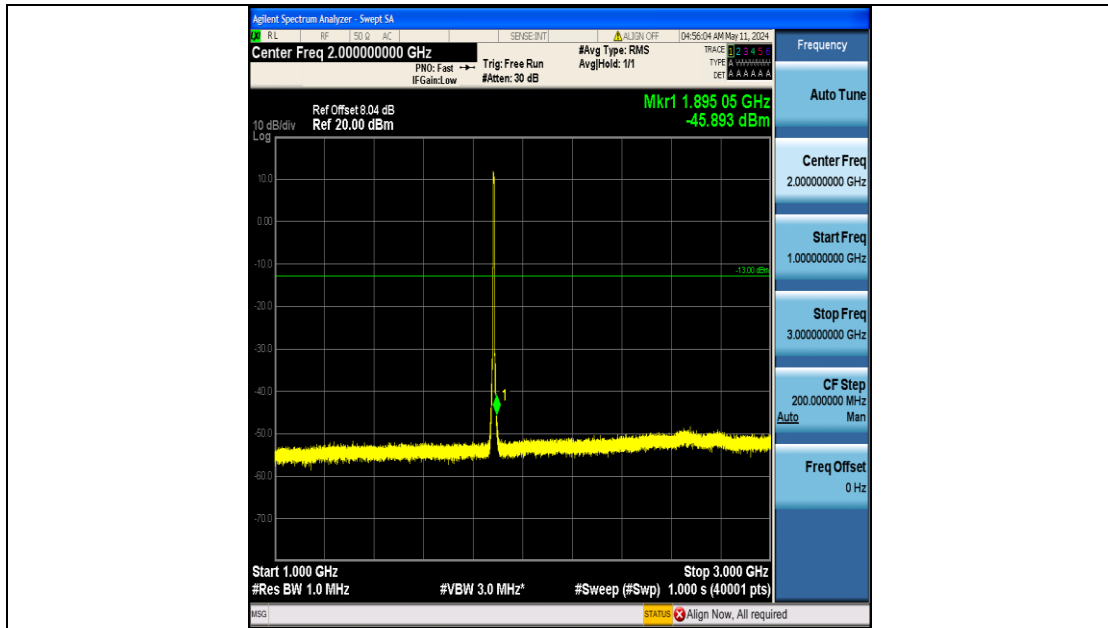
Band25_5MHz_16QAM_26365_25RB#0_1000~3000_1000~3000
