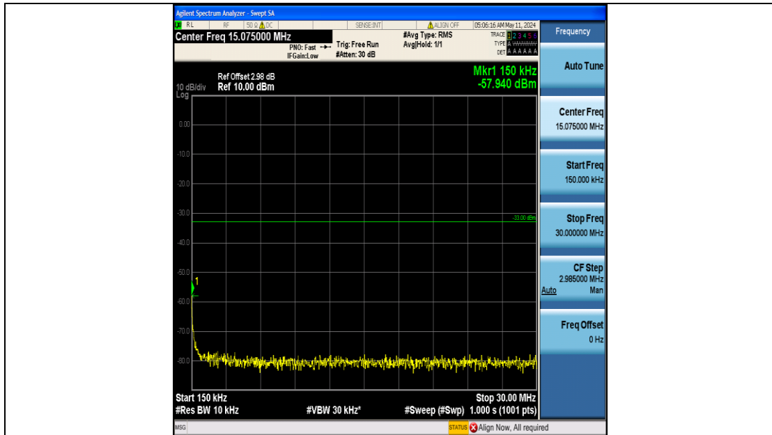
Band25_10MHz_QPSK_26090_50RB#0_0.15~30_0.15~30
