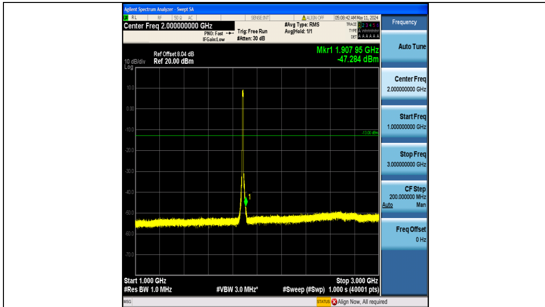
Band25_10MHz_16QAM_26365_50RB#0_1000~3000_1000~3000
