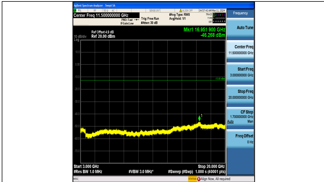
Band25_5MHz_16QAM_26665_25RB#0_3000~20000_3000~20000
