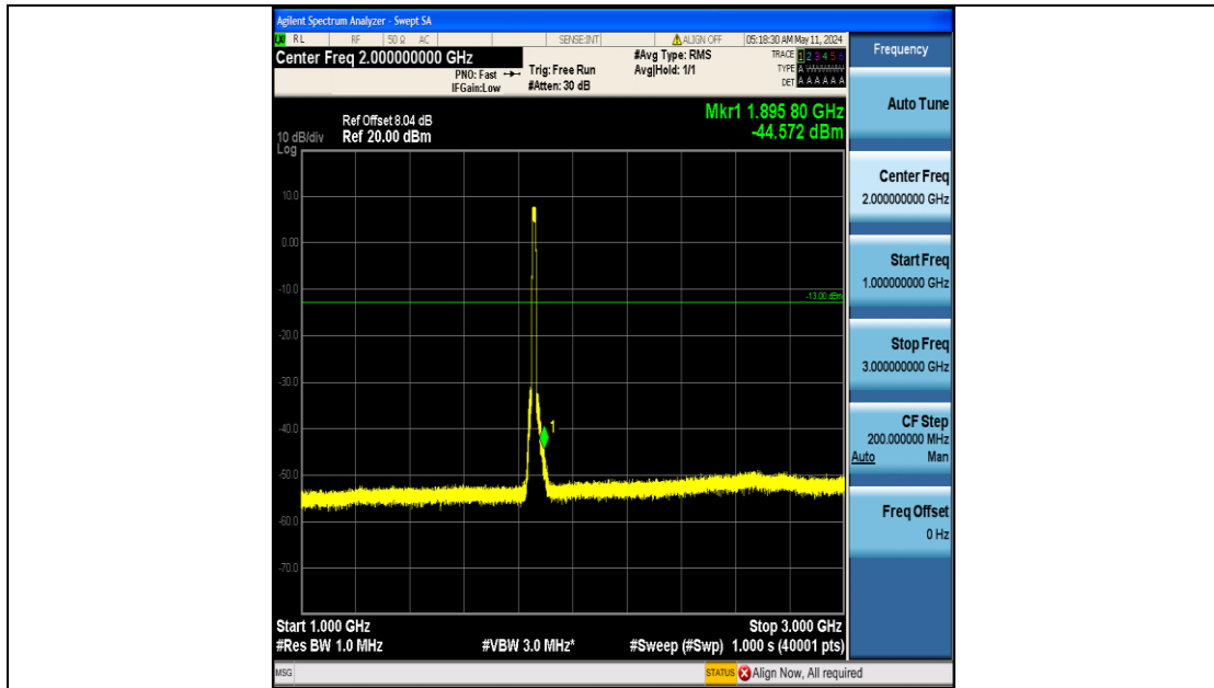
Band25_15MHz_QPSK_26115_75RB#0_1000~3000_1000~3000
