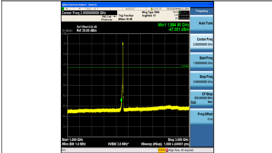
Band25_10MHz_16QAM_26640_50RB#0_1000~3000_1000~3000
