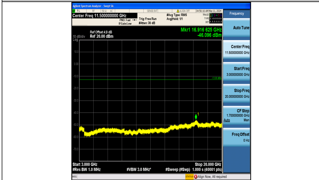
Band25_5MHz_16QAM_26365_25RB#0_3000~20000_3000~20000
