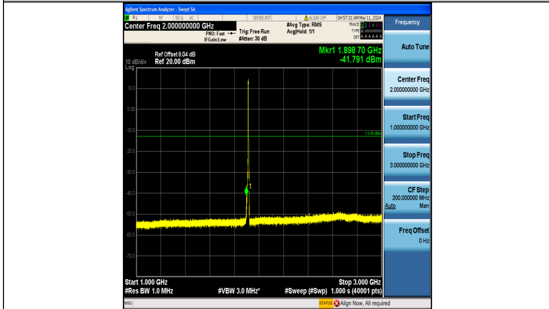
Band25_5MHz_16QAM_26665_25RB#0_1000~3000_1000~3000
