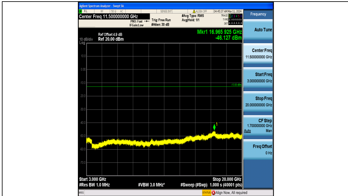
Band25_3MHz_16QAM_26675_15RB#0_3000~20000_3000~20000
