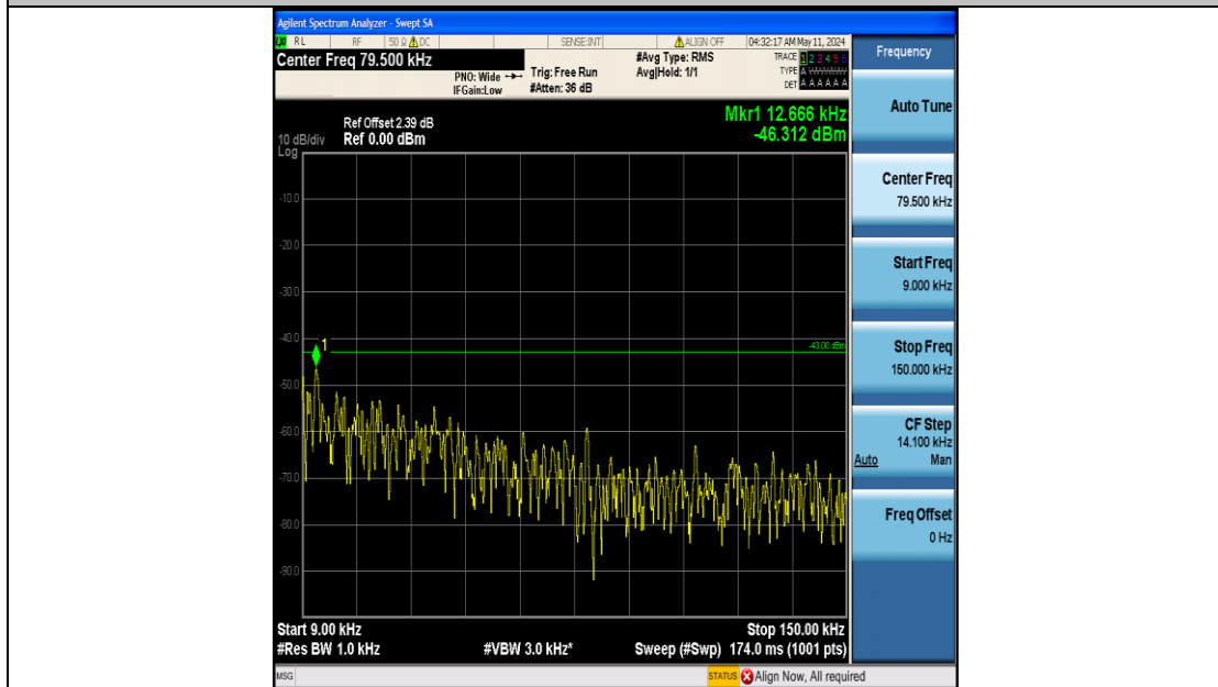
Band25_1.4MHz_16QAM_26365_6RB#0_0.009~0.15_0.009~0.15
