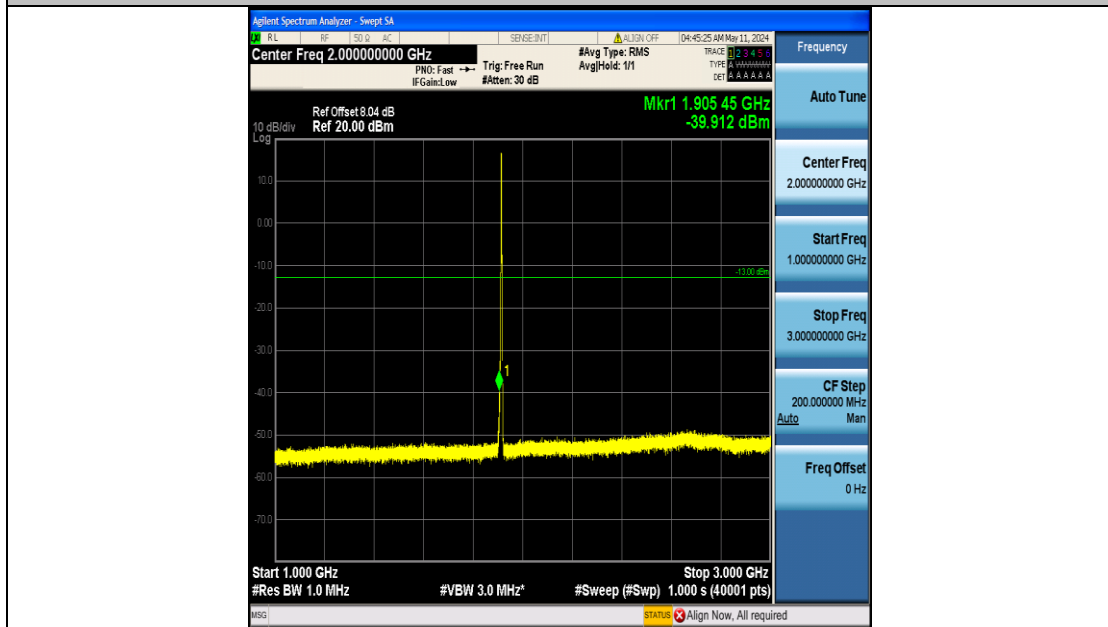
Band25_3MHz_16QAM_26675_15RB#0_1000~3000_1000~3000
