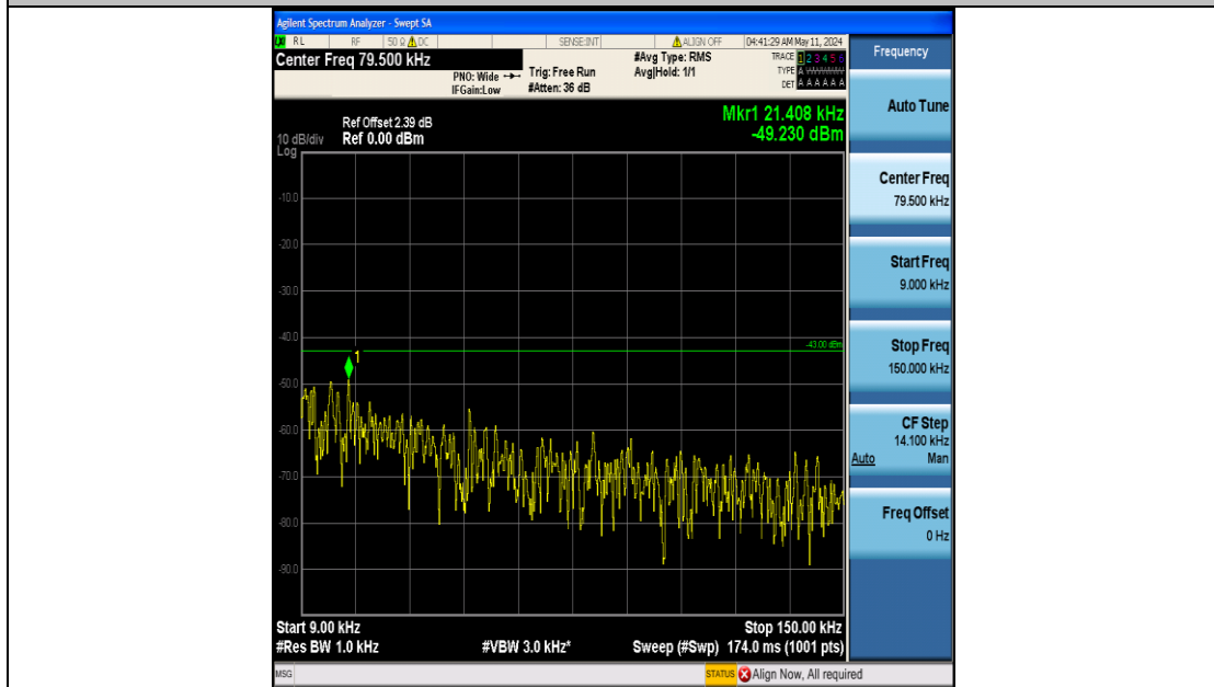
Band25_3MHz_QPSK_26055_15RB#0_0.009~0.15_0.009~0.15
