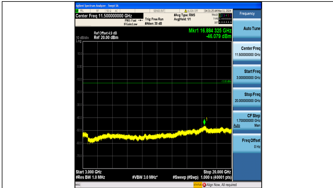
Band25_1.4MHz_16QAM_26047_6RB#0_3000~20000_3000~20000
