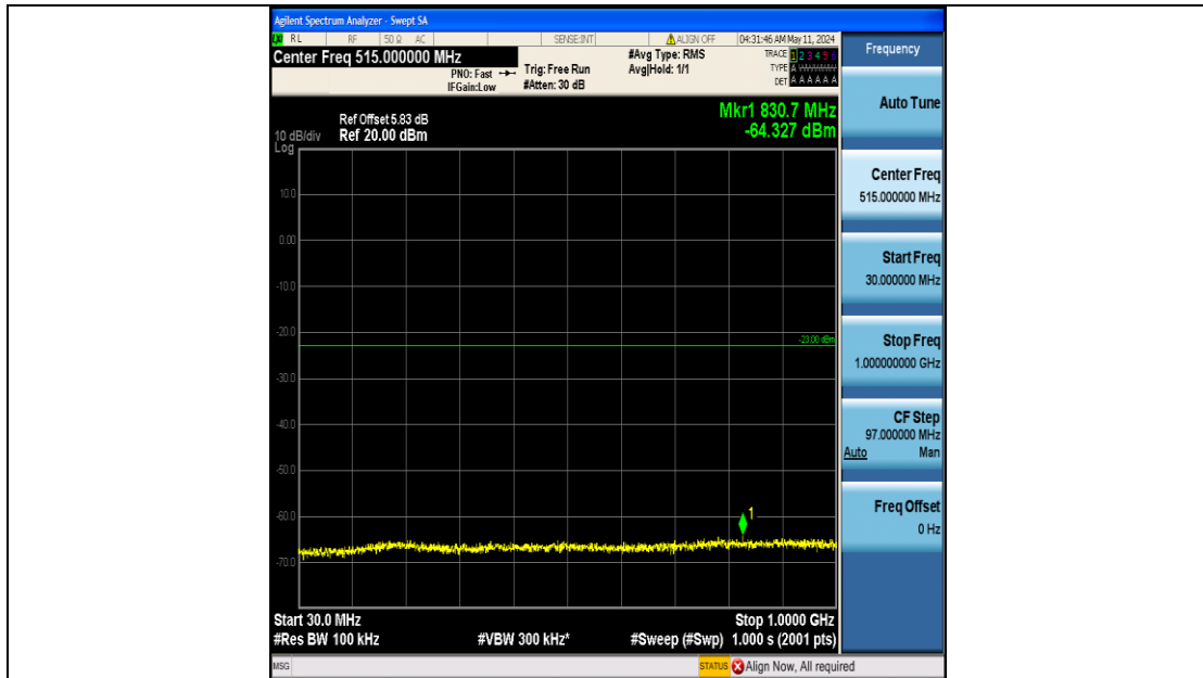
Band25_1.4MHz_QPSK_26365_6RB#0_30~1000_30~1000
