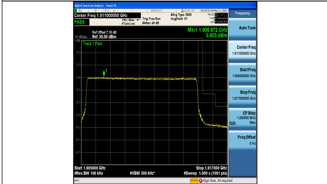
Band25_10MHz_16QAM_26640_50RB#0
