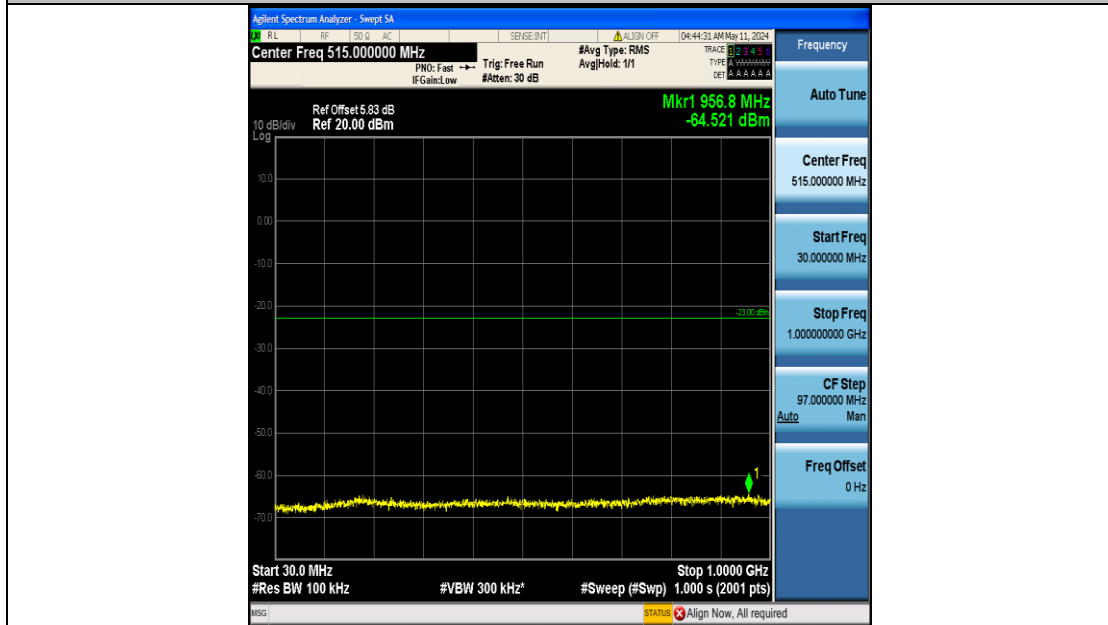
Band25_3MHz_QPSK_26675_15RB#0_30~1000_30~1000
