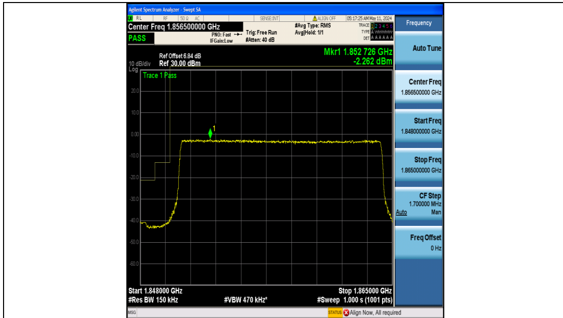
Band25_15MHz_QPSK_26115_75RB#0
