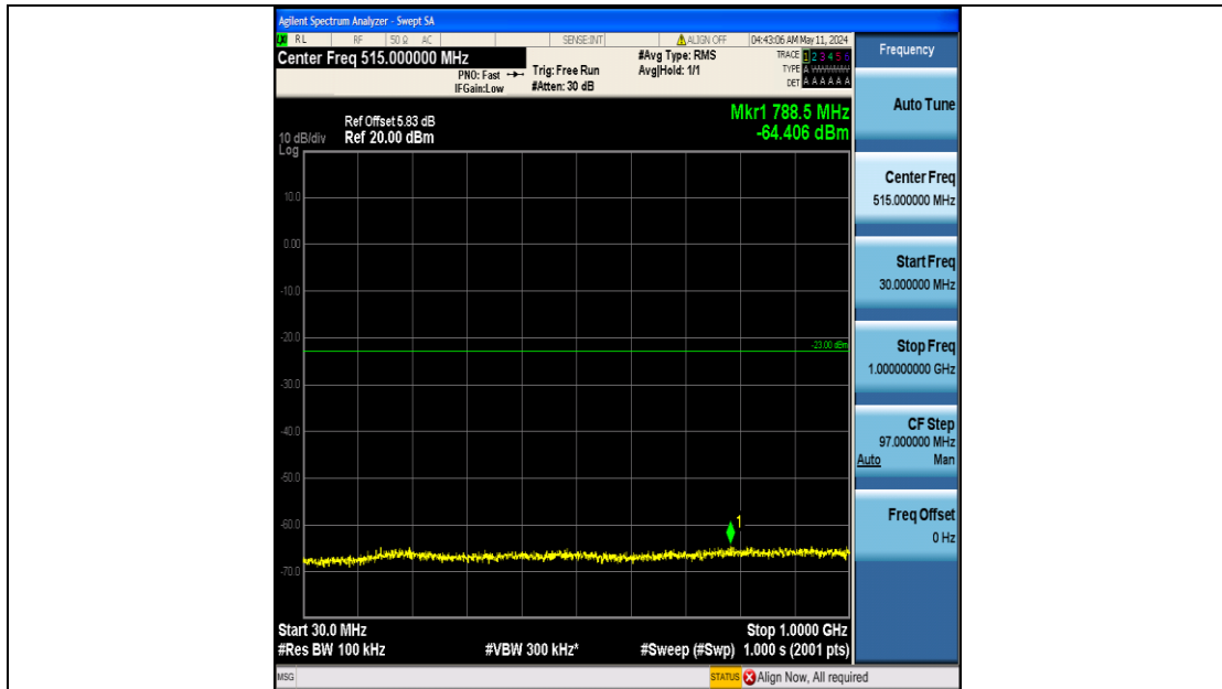
Band25_3MHz_QPSK_26365_15RB#0_30~1000_30~1000
