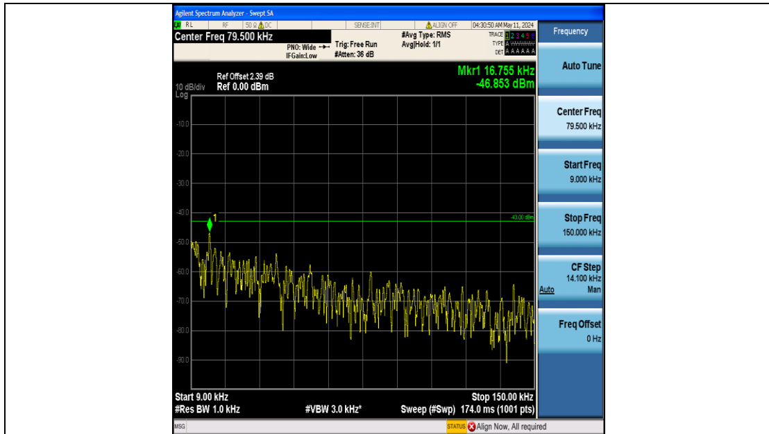
Band25_1.4MHz_16QAM_26047_6RB#0_0.009~0.15_0.009~0.15
