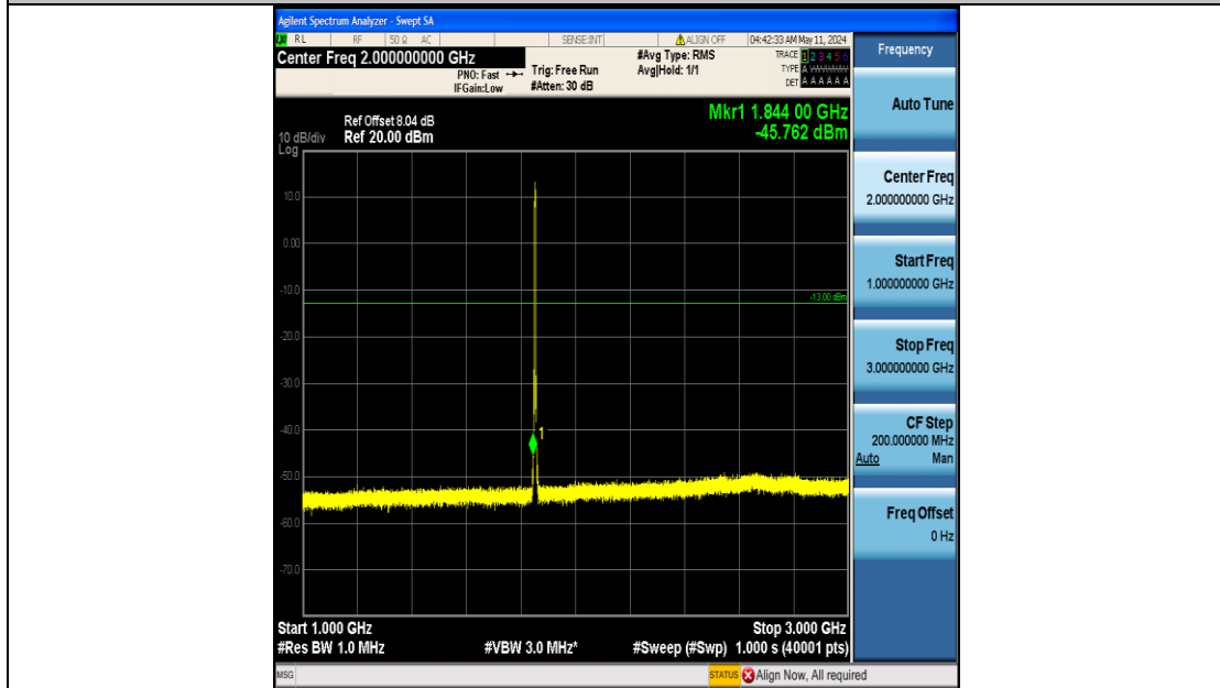
Band25_3MHz_16QAM_26055_15RB#0_1000~3000_1000~3000
