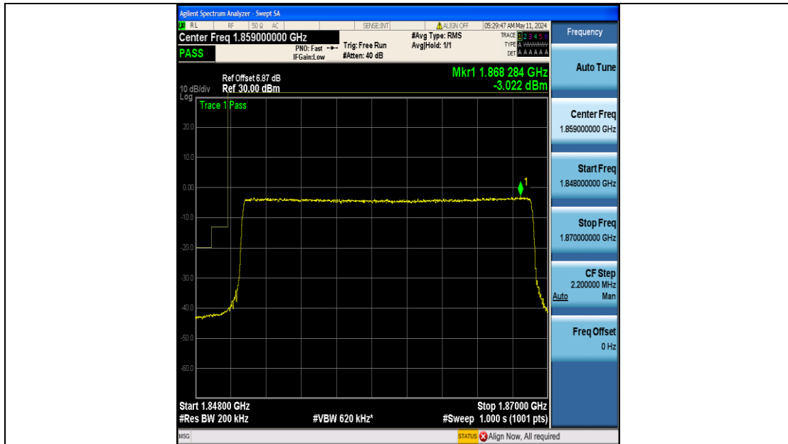
Band25_20MHz_16QAM_26140_100RB#0
