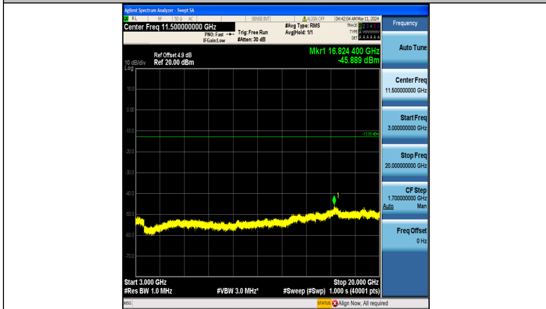
Band25_3MHz_QPSK_26055_15RB#0_3000~20000_3000~20000
