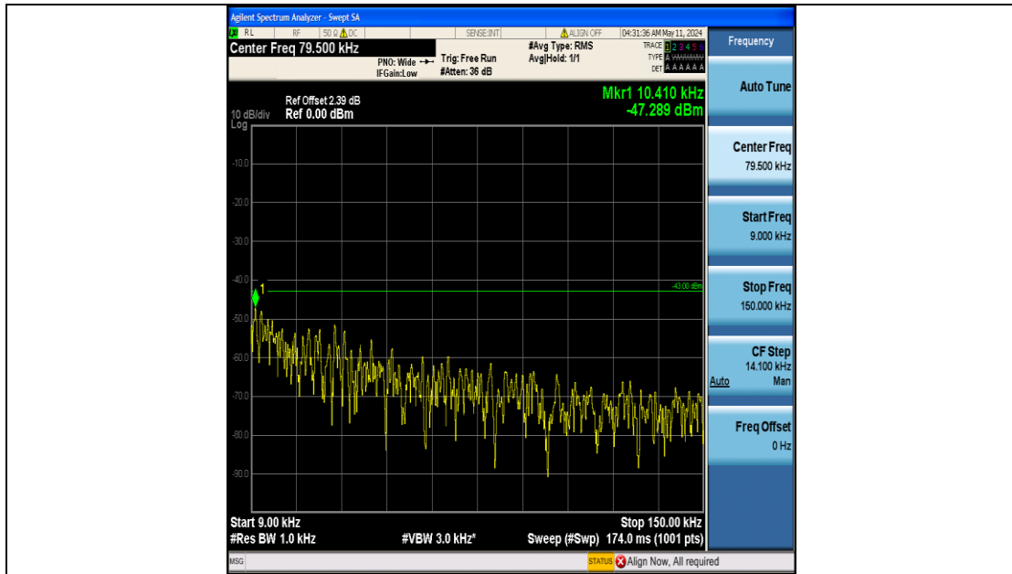
Band25_1.4MHz_QPSK_26365_6RB#0_0.009~0.15_0.009~0.15
