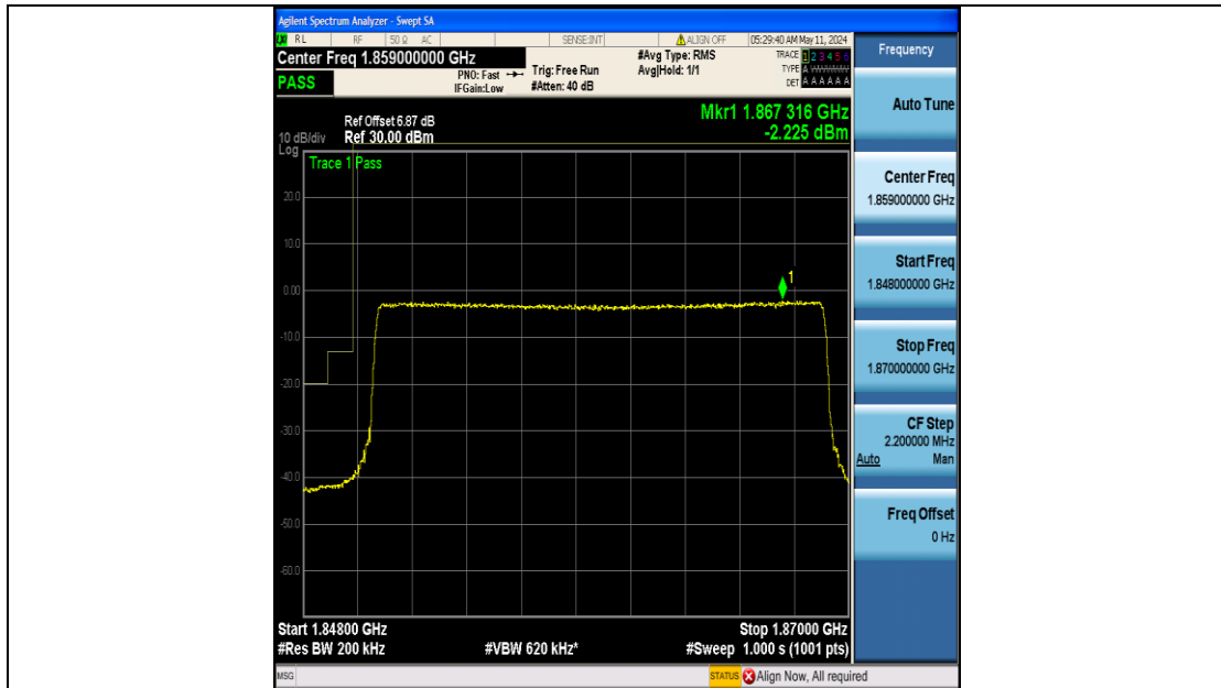
Band25_20MHz_QPSK_26140_100RB#0
