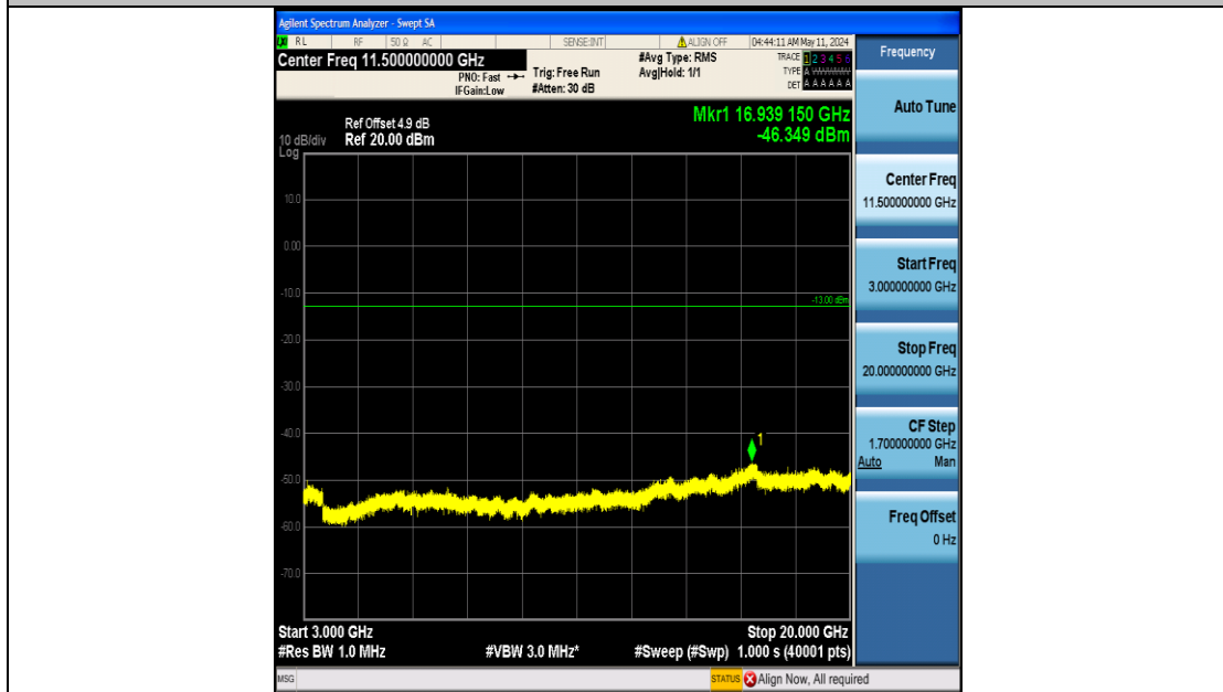
Band25_3MHz_16QAM_26365_15RB#0_3000~20000_3000~20000
