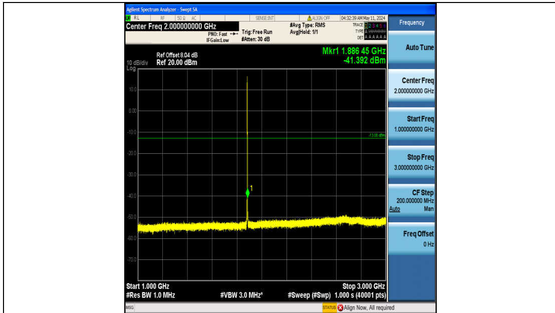
Band25_1.4MHz_16QAM_26365_6RB#0_1000~3000_1000~3000
