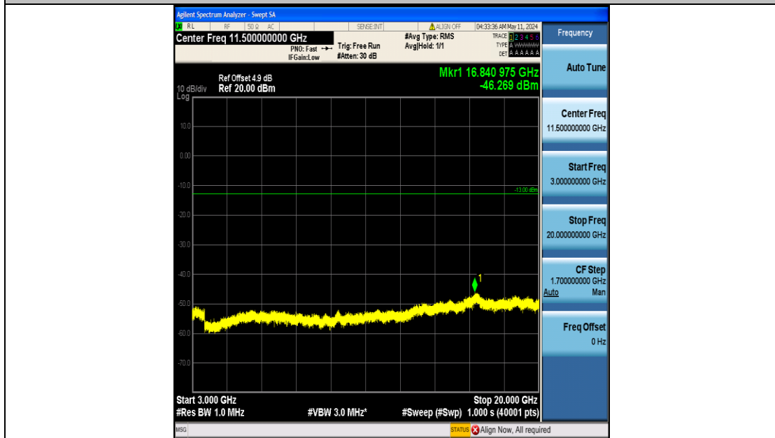
Band25_1.4MHz_QPSK_26683_6RB#0_3000~20000_3000~20000
