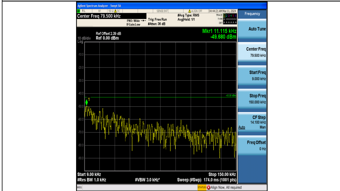
Band25_3MHz_QPSK_26675_15RB#0_0.009~0.15_0.009~0.15
