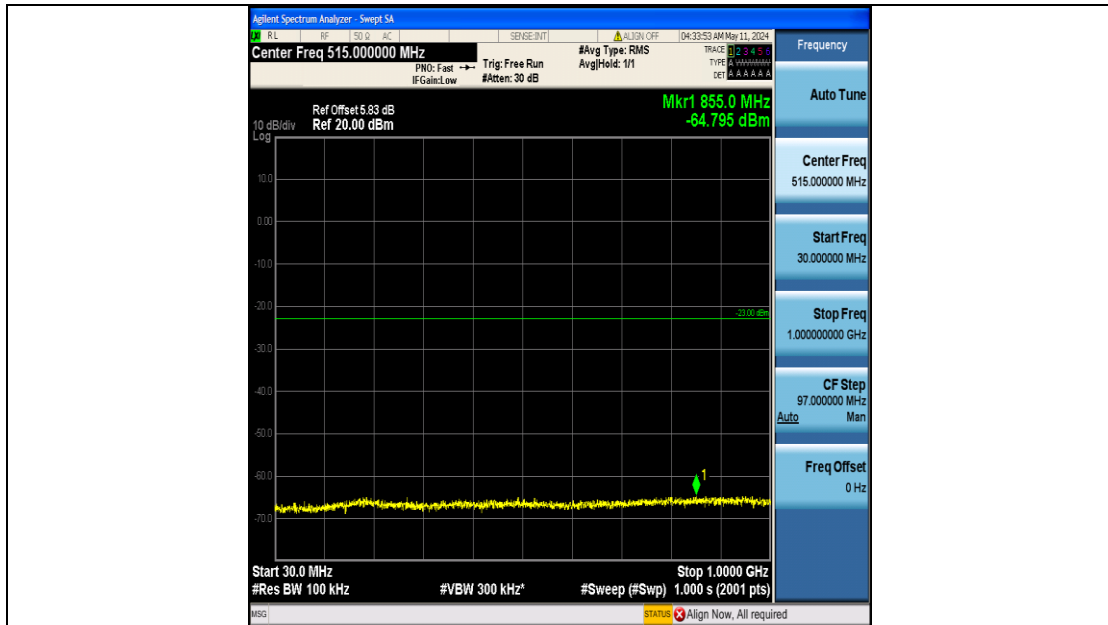
Band25_1.4MHz_16QAM_26683_6RB#0_30~1000_30~1000
