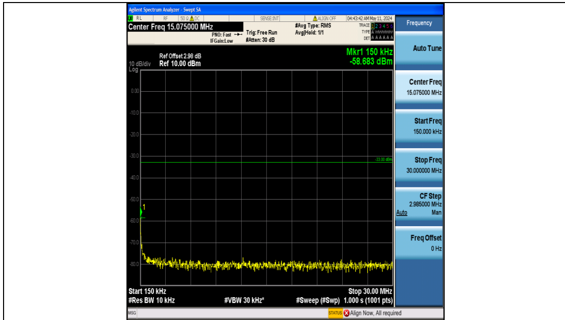
Band25_3MHz_16QAM_26365_15RB#0_0.15~30_0.15~30
