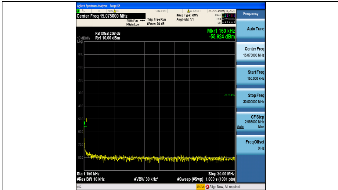
Band25_1.4MHz_16QAM_26365_6RB#0_0.15~30_0.15~30
