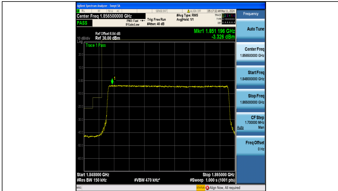
Band25_15MHz_16QAM_26115_75RB#0
