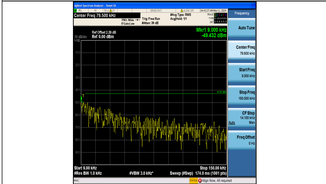
Band25_3MHz_16QAM_26365_15RB#0_0.009~0.15_0.009~0.15
