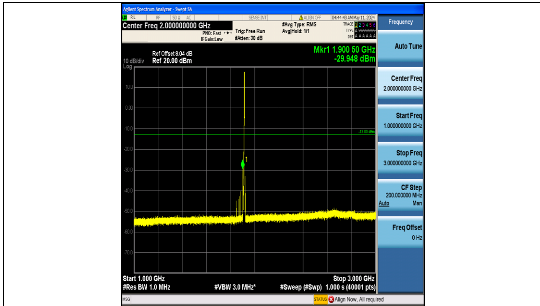
Band25_3MHz_QPSK_26675_15RB#0_1000~3000_1000~3000
