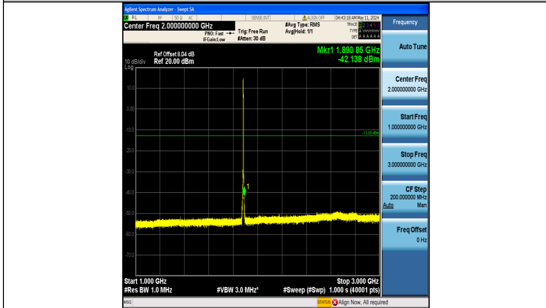
Band25_3MHz_QPSK_26365_15RB#0_1000~3000_1000~3000
