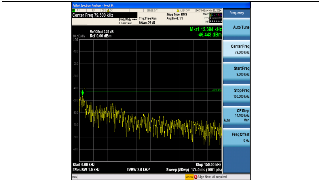
Band25_1.4MHz_16QAM_26683_6RB#0_0.009~0.15_0.009~0.15
