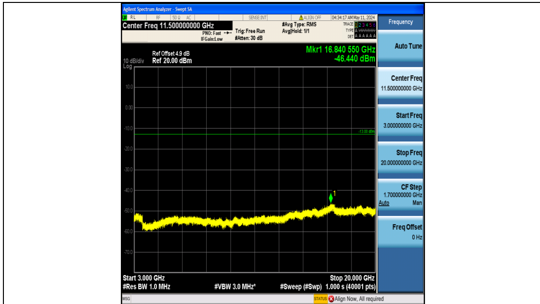
Band25_1.4MHz_16QAM_26683_6RB#0_3000~20000_3000~20000
