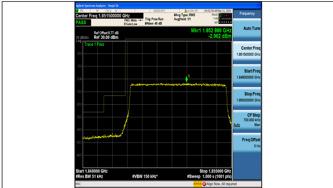
Band25_5MHz_16QAM_26065_25RB#0
