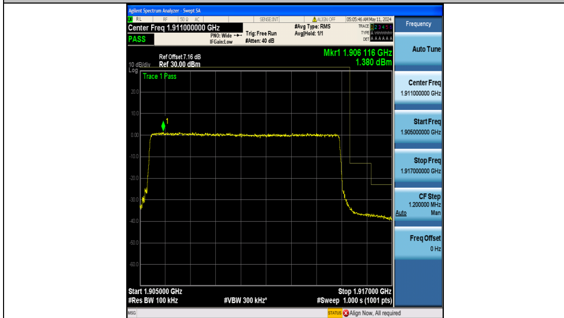
Band25_10MHz_QPSK_26640_50RB#0
