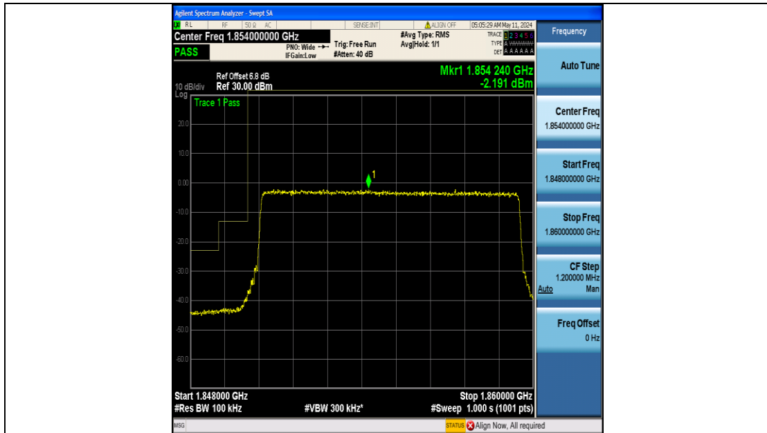
Band25_10MHz_QPSK_26090_50RB#0
