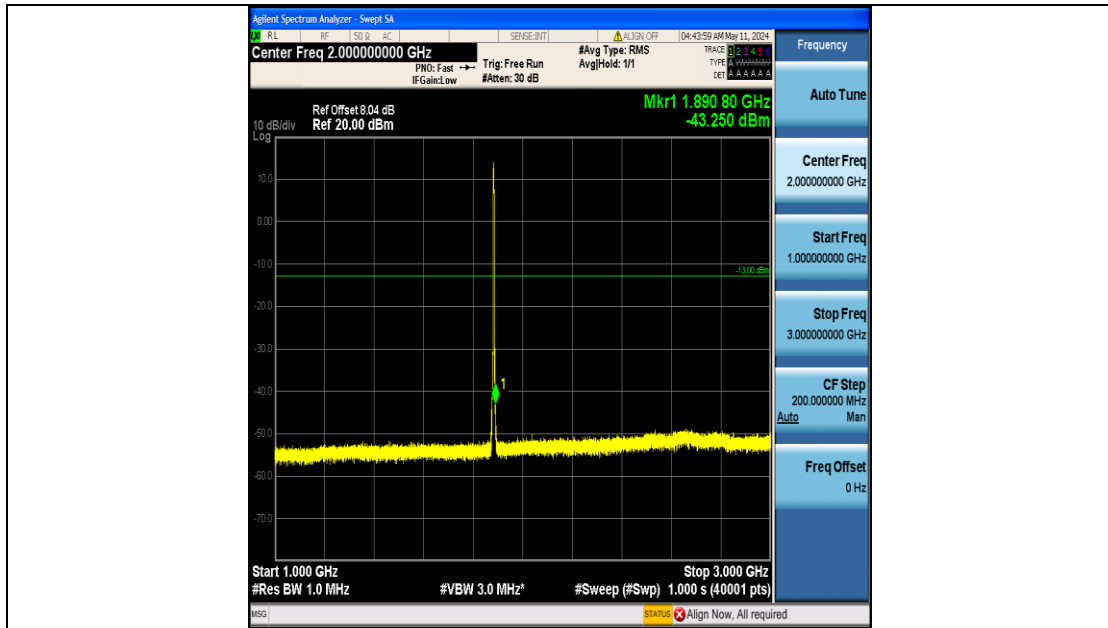
Band25_3MHz_16QAM_26365_15RB#0_1000~3000_1000~3000
