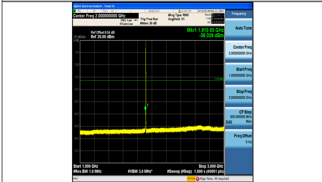
Band25_1.4MHz_16QAM_26683_6RB#0_1000~3000_1000~3000
