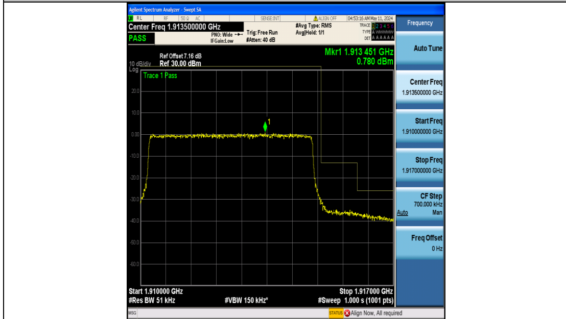
Band25_5MHz_16QAM_26665_25RB#0
