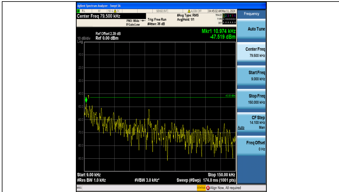
Band25_3MHz_16QAM_26675_15RB#0_0.009~0.15_0.009~0.15
