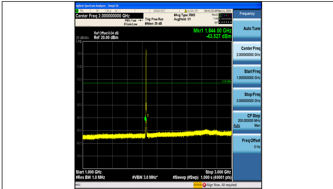
Band25_3MHz_QPSK_26055_15RB#0_1000~3000_1000~3000
