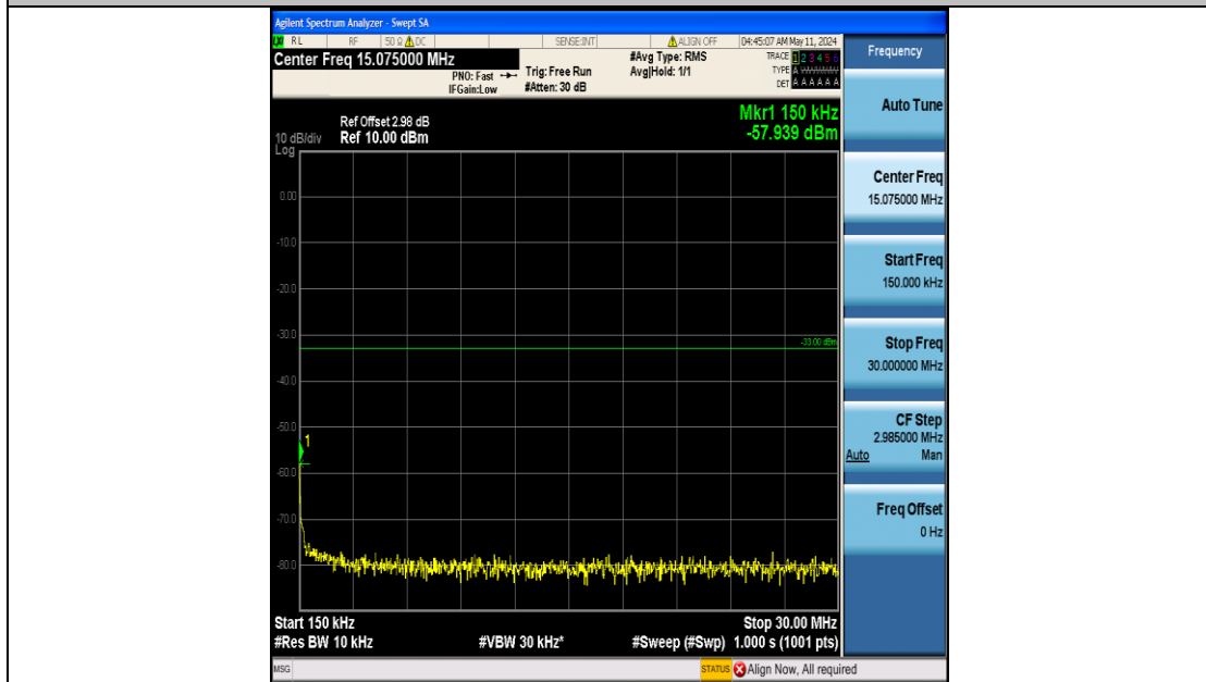
Band25_3MHz_16QAM_26675_15RB#0_0.15~30_0.15~30
