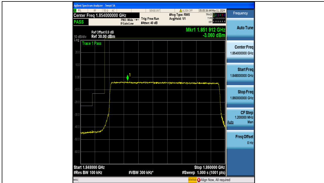
Band25_10MHz_16QAM_26090_50RB#0
