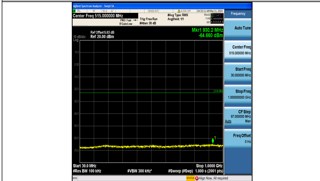
Band25_1.4MHz_QPSK_26683_6RB#0_30~1000_30~1000
