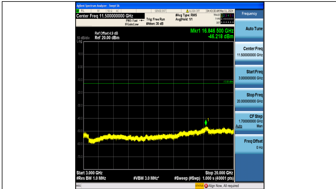
Band25_3MHz_QPSK_26365_15RB#0_3000~20000_3000~20000
