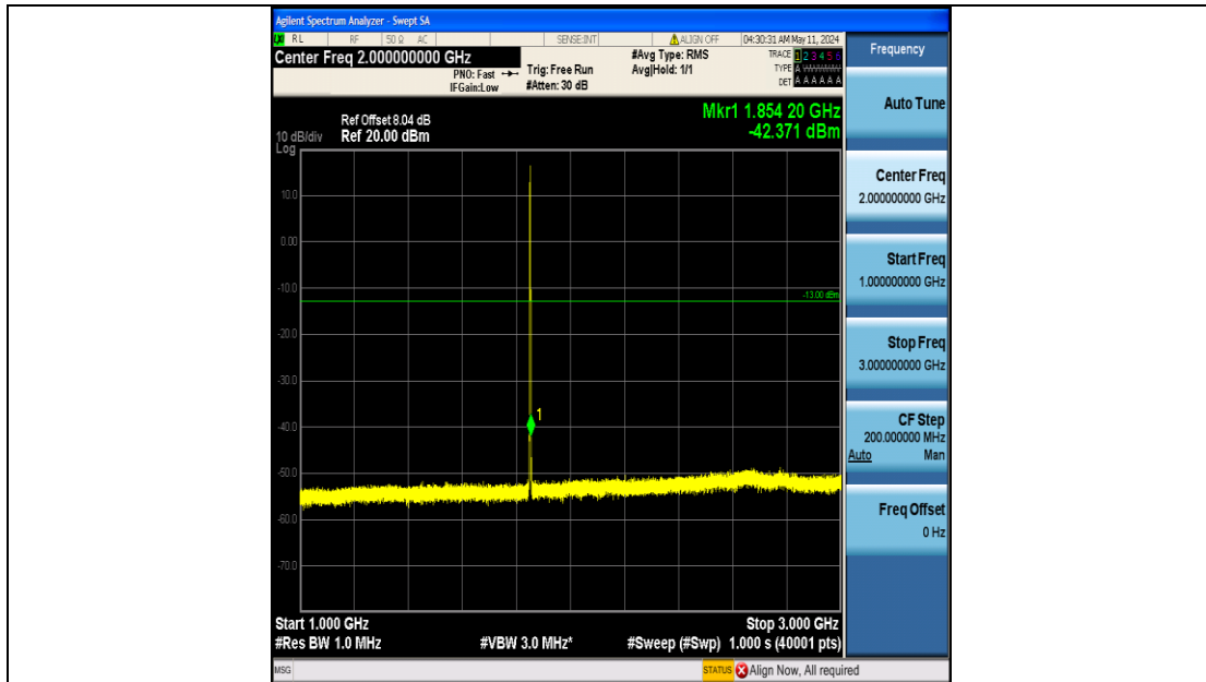
Band25_1.4MHz_QPSK_26047_6RB#0_1000~3000_1000~3000
