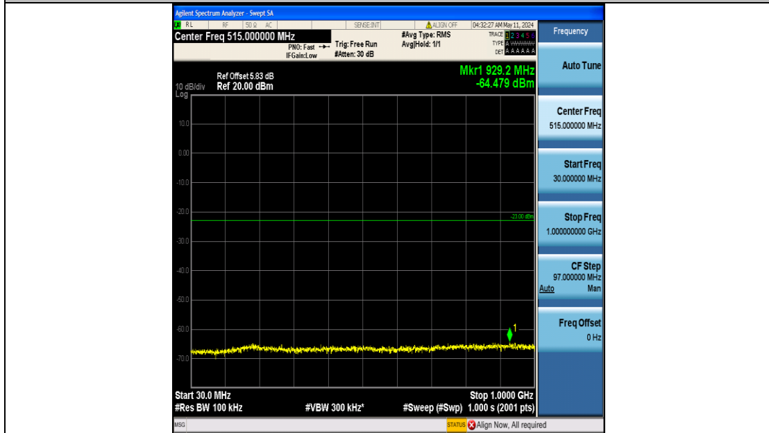
Band25_1.4MHz_16QAM_26365_6RB#0_30~1000_30~1000
