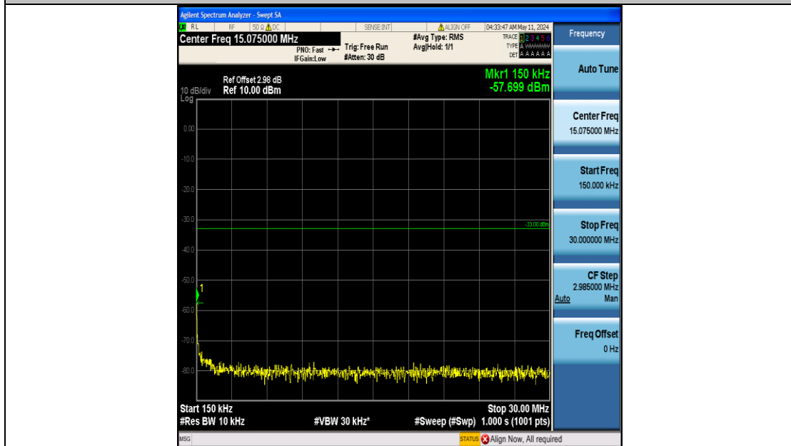
Band25_1.4MHz_16QAM_26683_6RB#0_0.15~30_0.15~30
