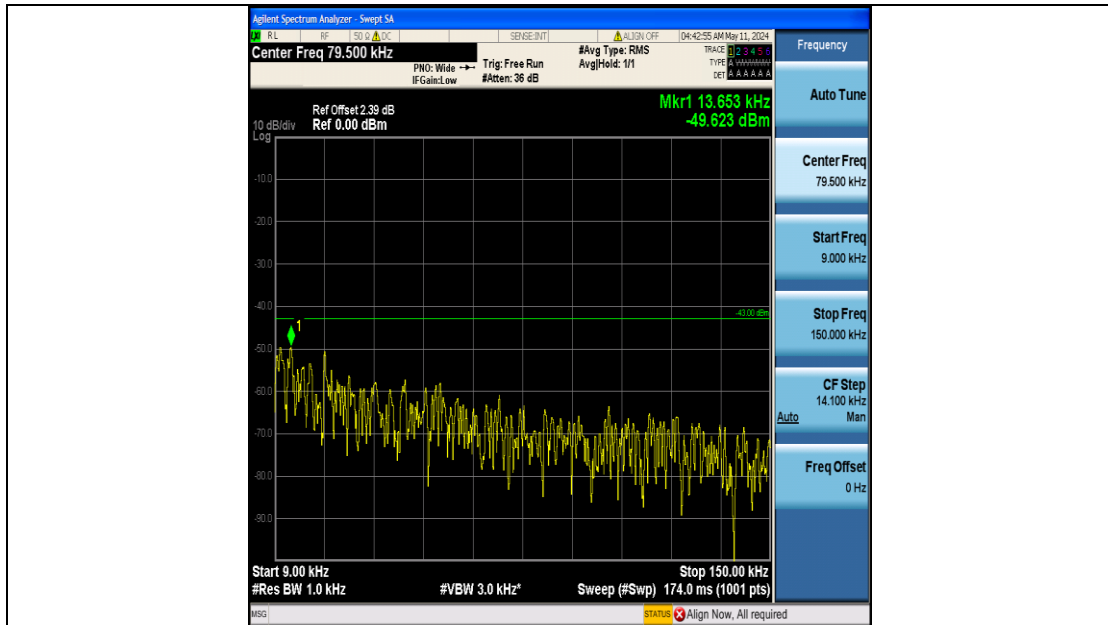
Band25_3MHz_QPSK_26365_15RB#0_0.009~0.15_0.009~0.15
