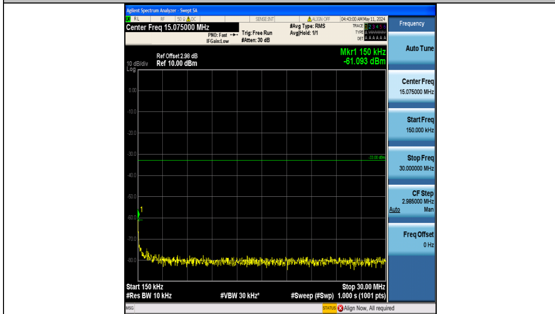
Band25_3MHz_QPSK_26365_15RB#0_0.15~30_0.15~30
