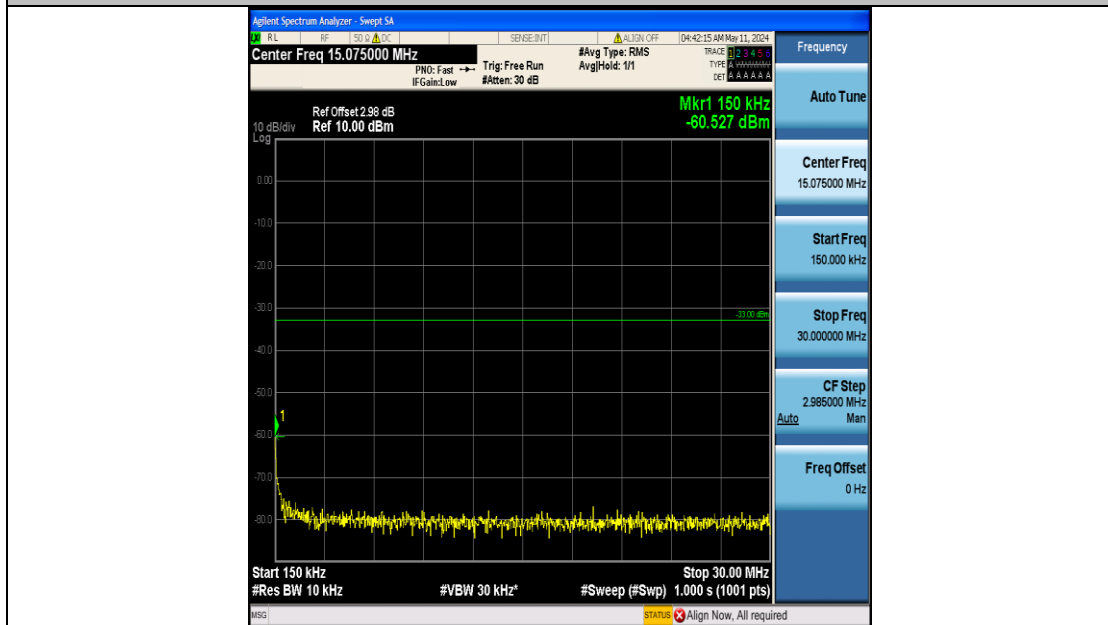
Band25_3MHz_16QAM_26055_15RB#0_0.15~30_0.15~30
