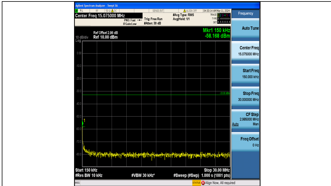
Band25_1.4MHz_QPSK_26047_6RB#0_0.15~30_0.15~30
