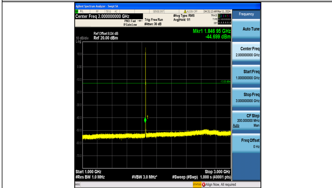
Band25_1.4MHz_16QAM_26047_6RB#0_1000~3000_1000~3000
