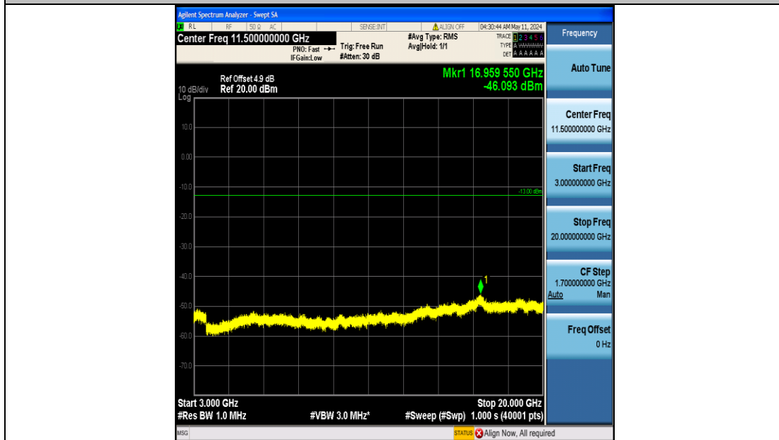
Band25_1.4MHz_QPSK_26047_6RB#0_3000~20000_3000~20000
