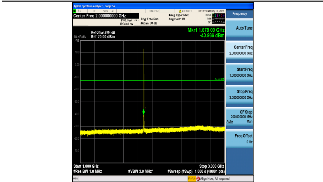
Band25_1.4MHz_QPSK_26365_6RB#0_1000~3000_1000~3000
