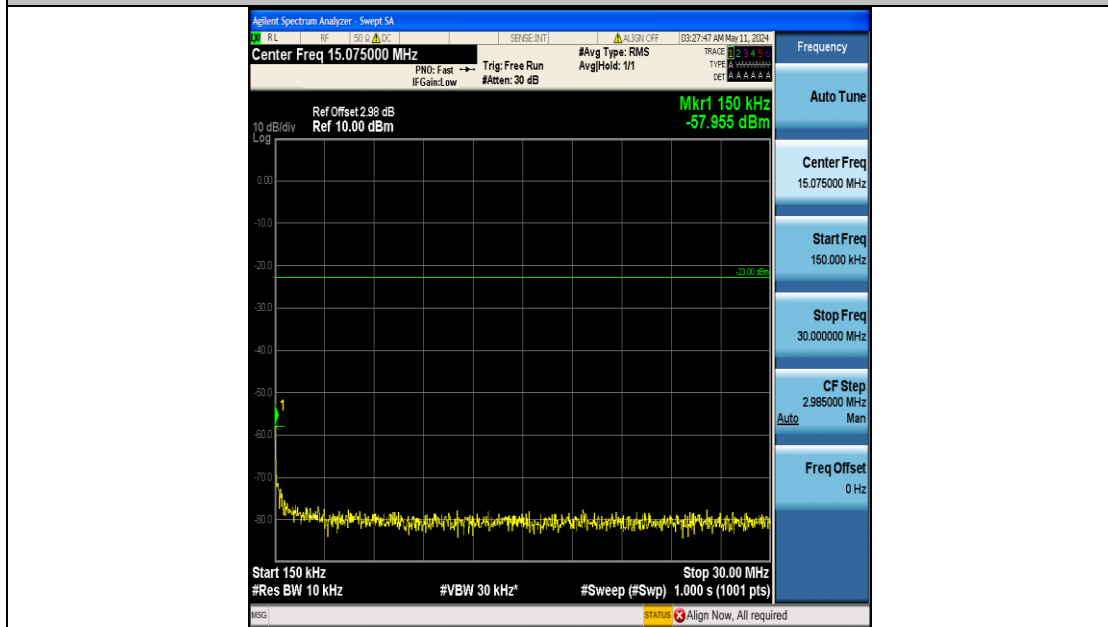
Band12_3MHz_QPSK_23025_15RB#0_0.15~30_0.15~30
