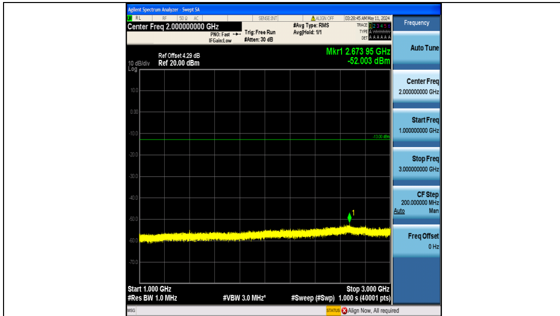
Band12_3MHz_16QAM_23025_15RB#0_1000~3000_1000~3000
