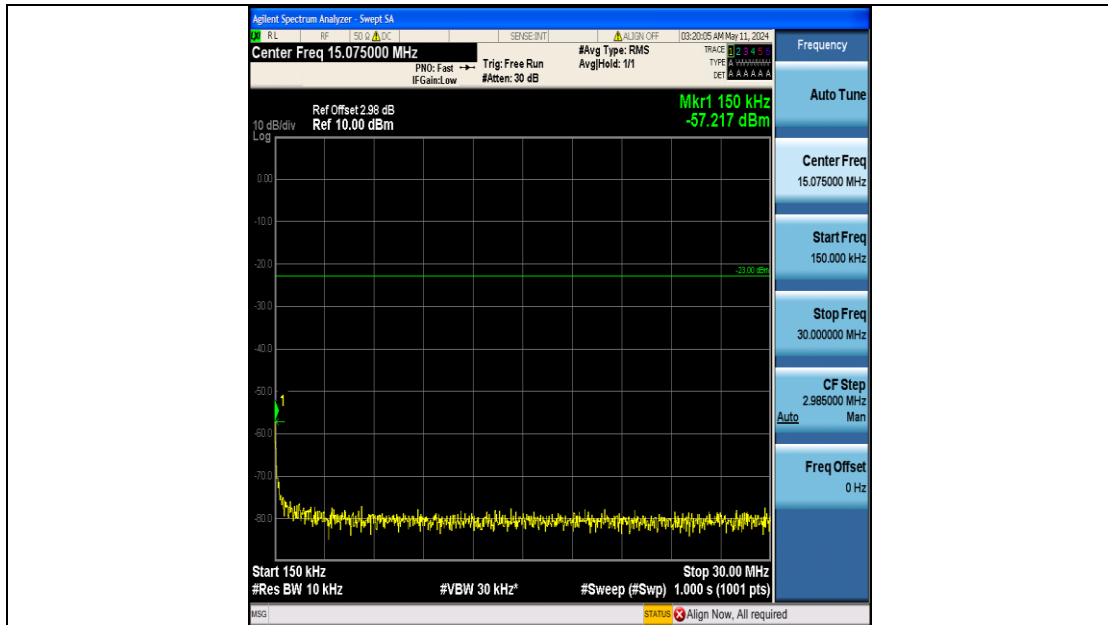
Band12_1.4MHz_16QAM_23173_6RB#0_0.15~30_0.15~30
