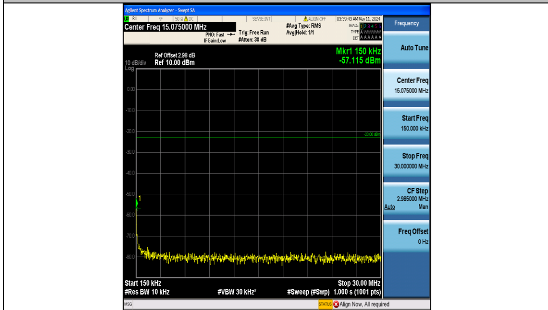
Band12_5MHz_QPSK_23035_25RB#0_0.15~30_0.15~30
