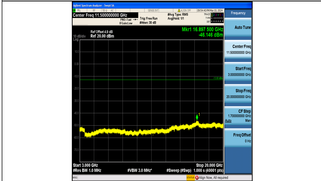
Band2_5MHz_QPSK_18625_25RB#0_3000~20000_3000~20000
