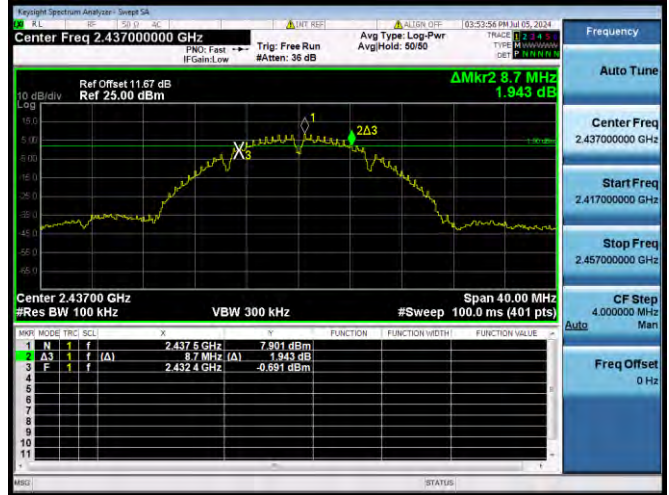
802.11b CHANNEL 6
