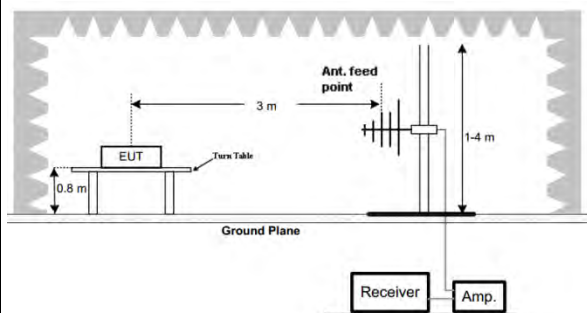
Above 1GHz
