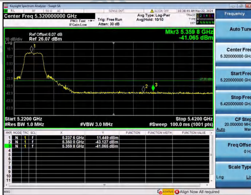
Bandedge_NVNT_ANT1_802_11n(HT20)_5240
