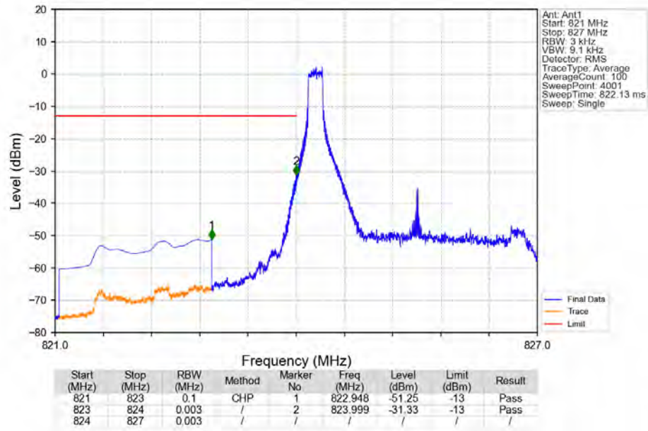
Band5_3MHz_QPSK_LCH_825.5MHz_RB_1_0_NTNV
