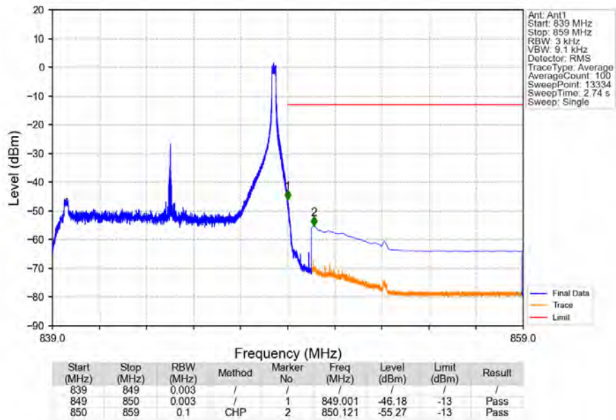
Band5 10MHz 16QAM HCH 844MHz RB 1 49 NTNV
