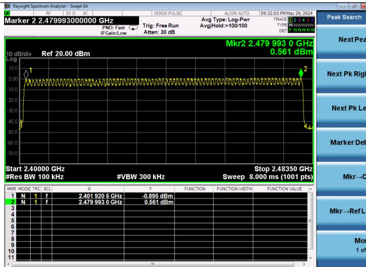
π/4DQPSK Modulation
