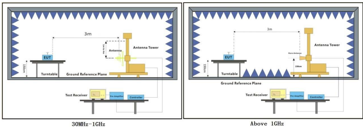
30MHz-1GHz
