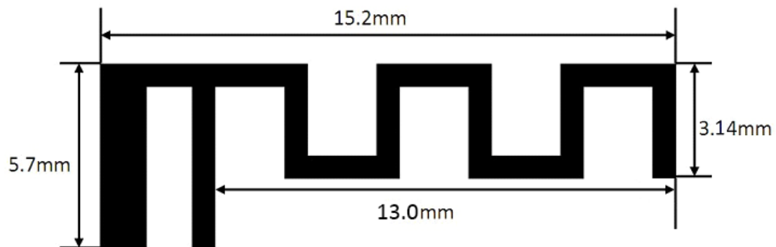
PCB antenna Antenna Photo & Length (mm)
