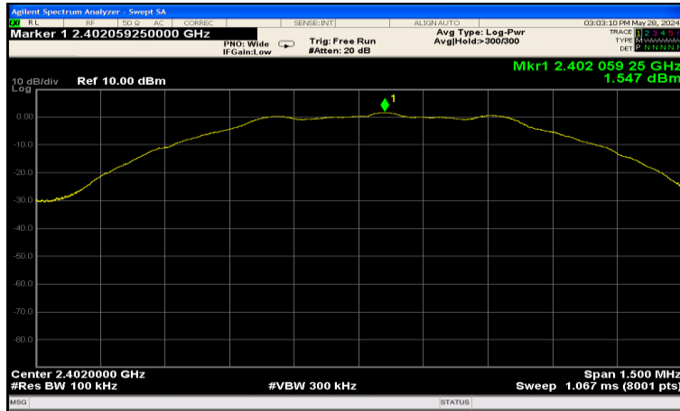
Reference Level, Lowest Channel (2 402 MHz)
