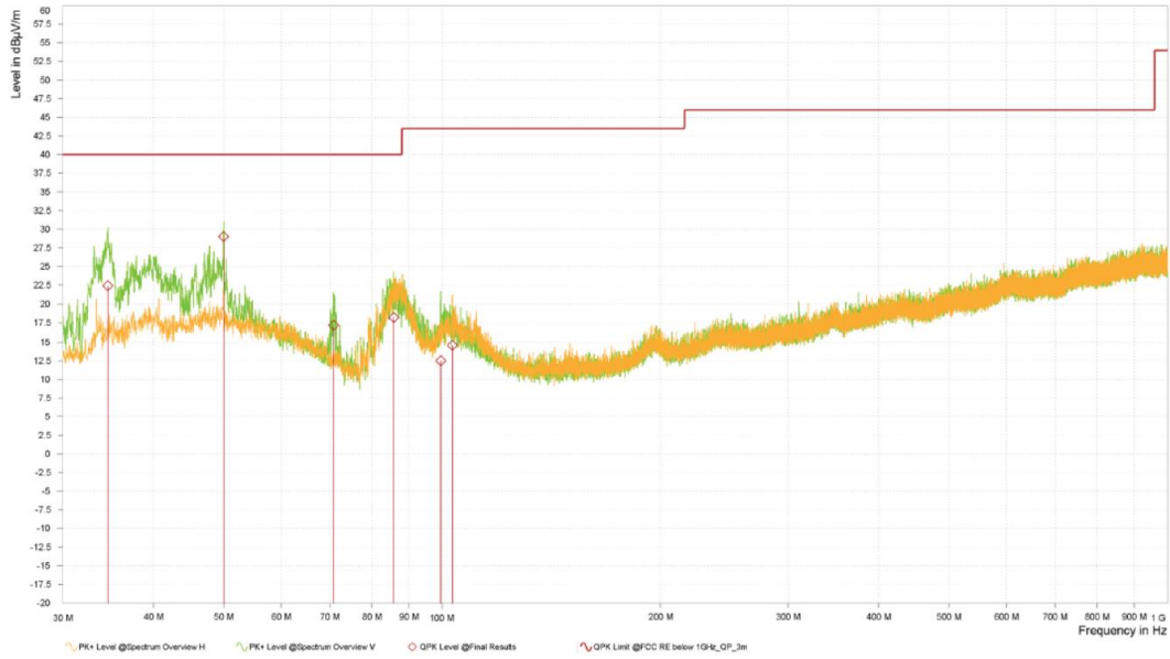
Radiated emission below 1GHz, Highest Channel (2 480 MHz)
