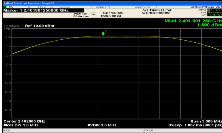
Peak Output Power, Lowest Channel (2 402 MHz)
