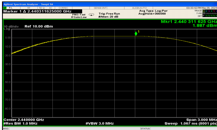
Peak Output Power, Middle Channel (2 440 MHz)
