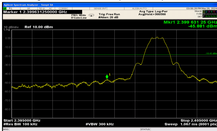
Band Edge, Lowest Channel (2 402 MHz)
