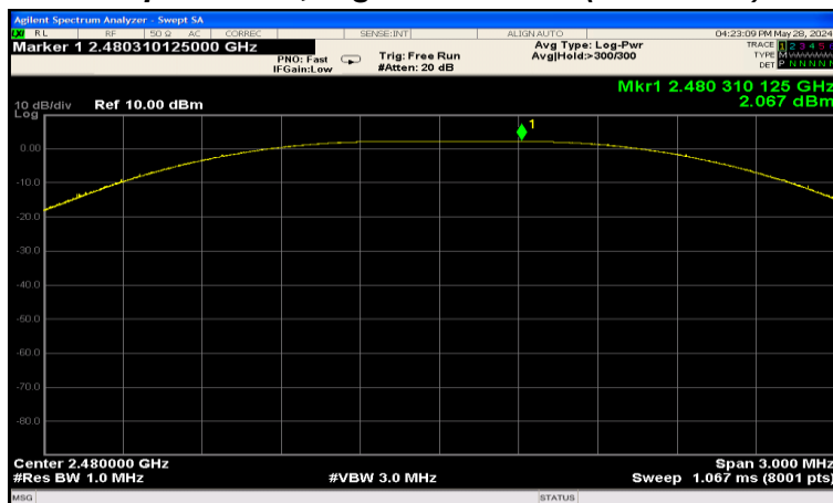
Peak Output Power, Highest Channel (2 480 MHz)
