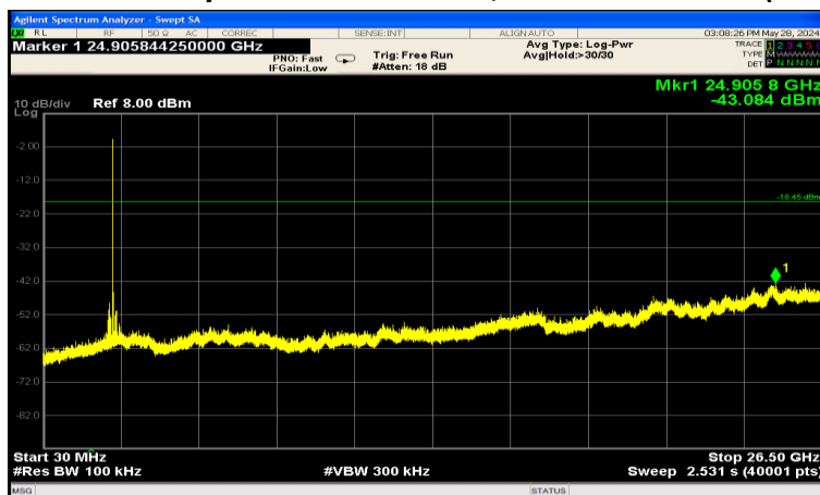
Conducted Spurious Emissions, Lowest Channel (2 402 MHz)
