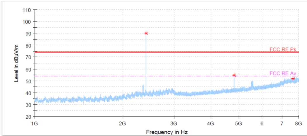
Lowest Channel (2 402 MHz) : 1 GHz to 8 GHz_Peak
