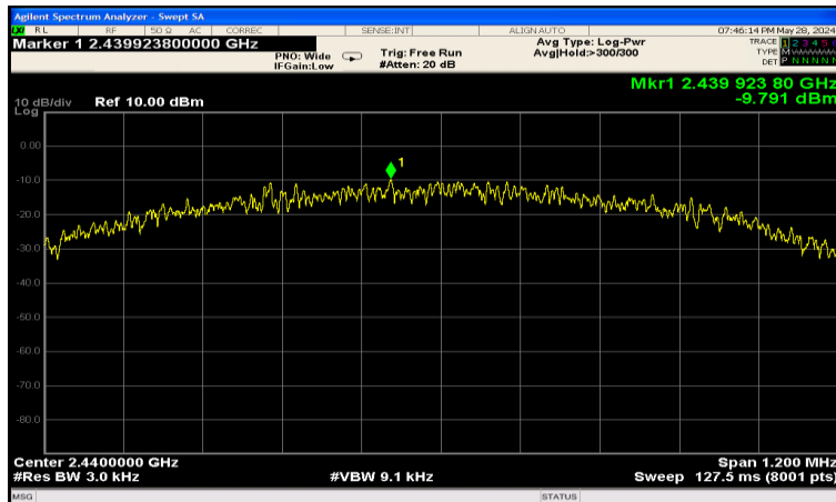
Power Spectral Density, Middle Channel (2 440 MHz)
