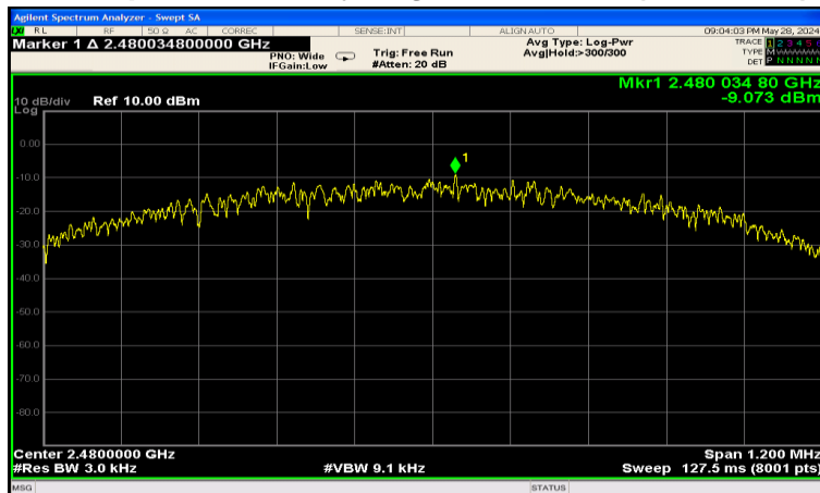
Power Spectral Density, Highest Channel (2 480 MHz)
