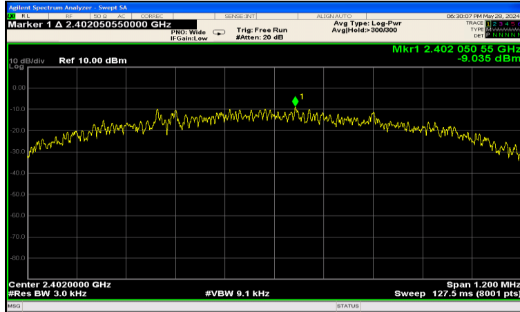
Power Spectral Density, Lowest Channel (2 402 MHz)
