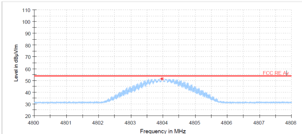
Lowest Channel (2 402 MHz) : 2 nd harmonic_Average
