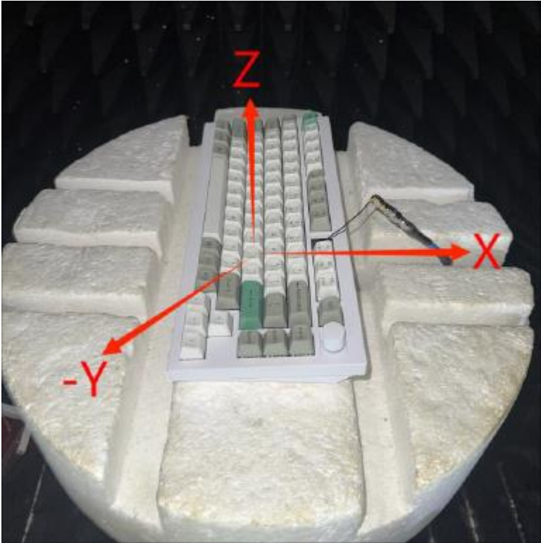
产品规格图(Antenna Specification chart)
