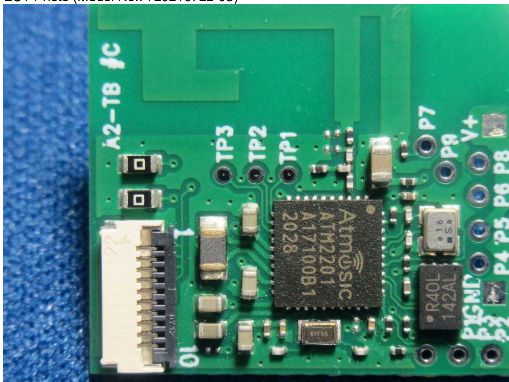
(13) EUT Photo (Model No.: 720210722-03)
