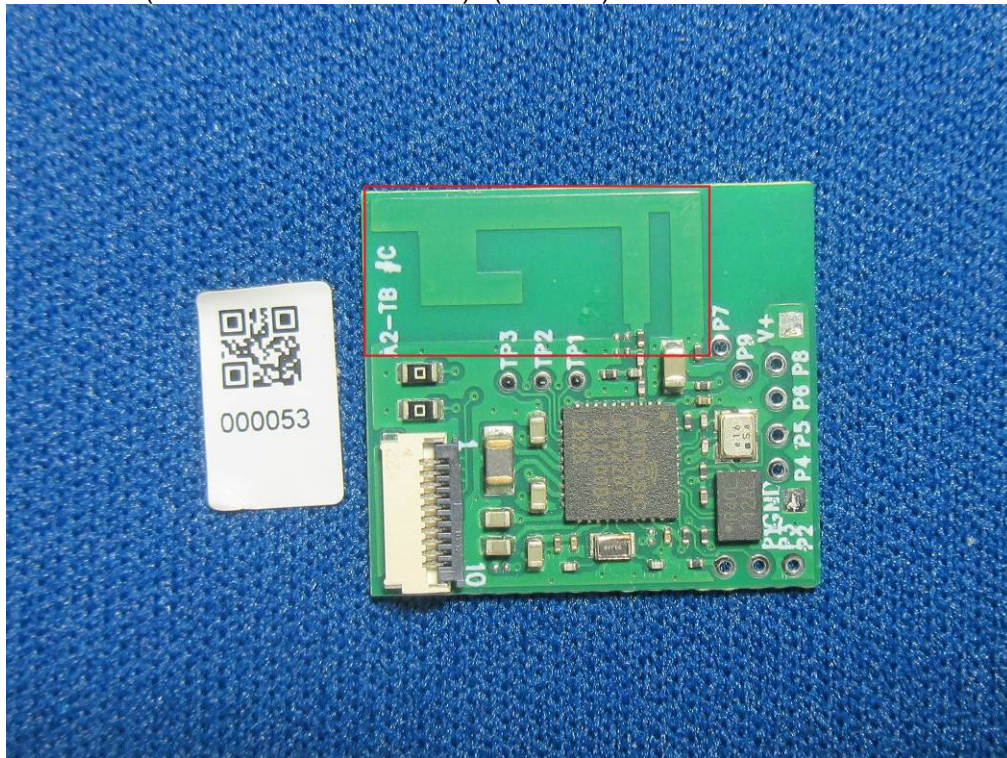
(14) EUT Photo (Model No.: 720210722-03) / (Antenna)
