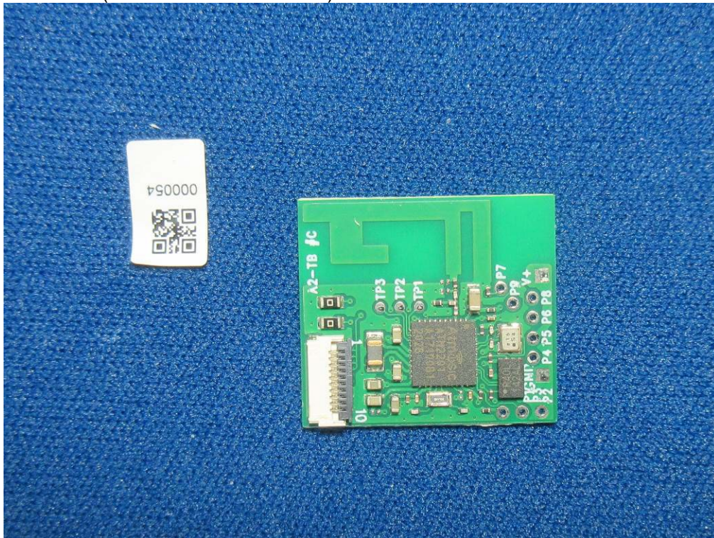
(6) EUT Photo (Model No.: 720210122-03)
