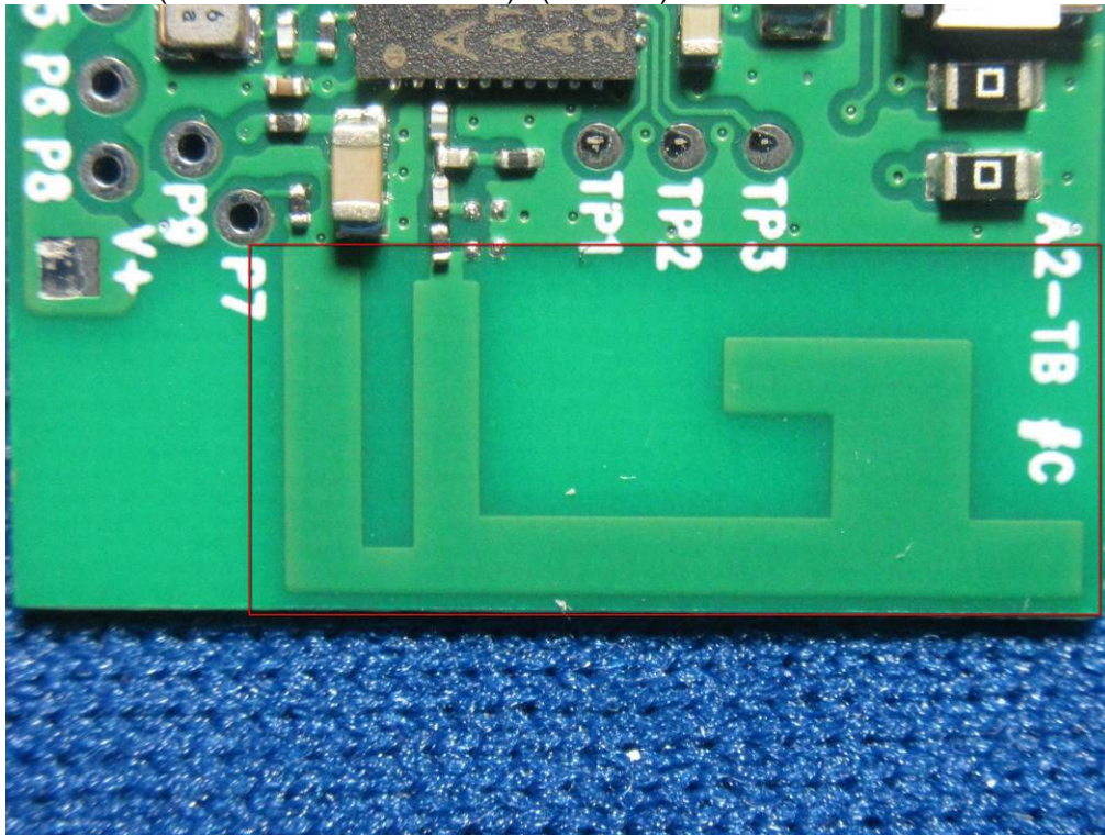
(7) EUT Photo (Model No.: 720210122-03) / (Antenna)
