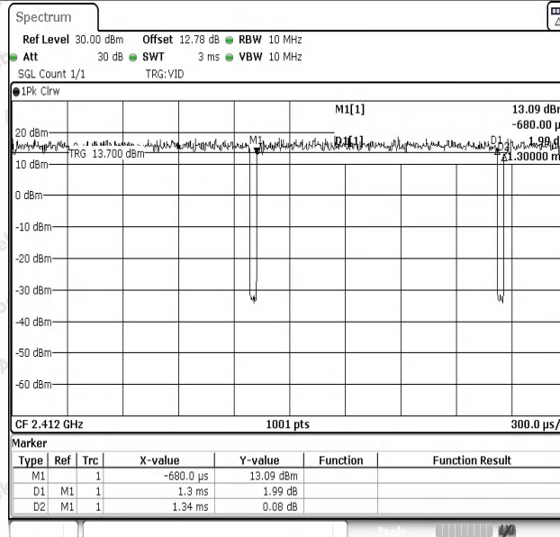
NTNV-11N20SISO-Ant1-2412
