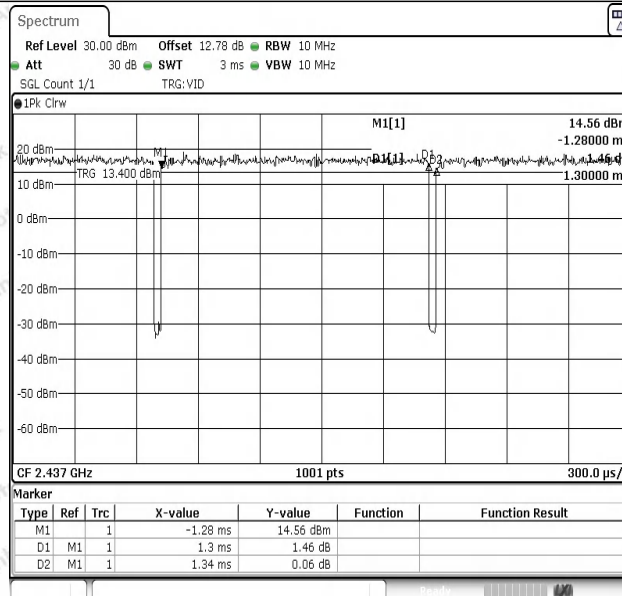
NTNV-11N20SISO-Ant1-2437
