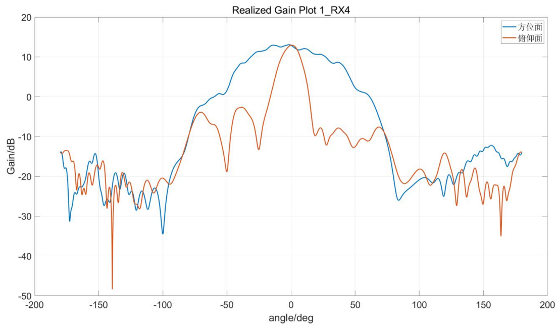
Figure1.4 RX4 directional diagram
