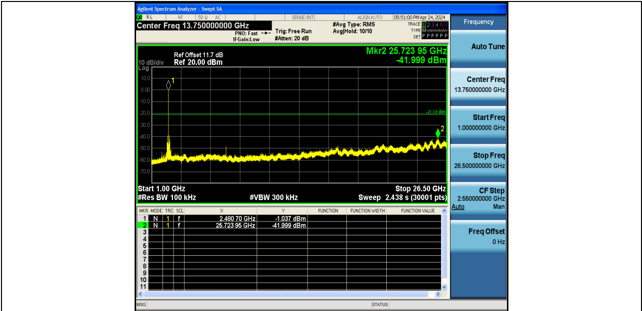
BLE_1M-Ant1-2480-1000~26500-PASS
