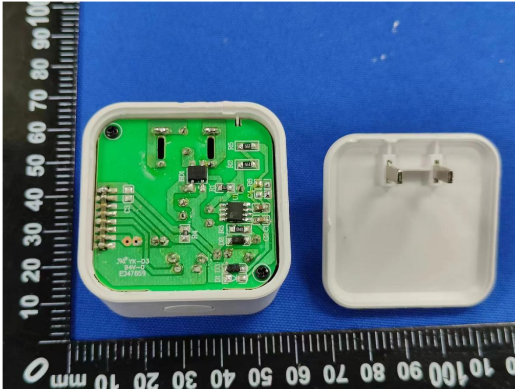
Internal view of unit(Model:AC-DB-CHV1)
