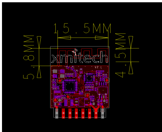
PCB Antenna
