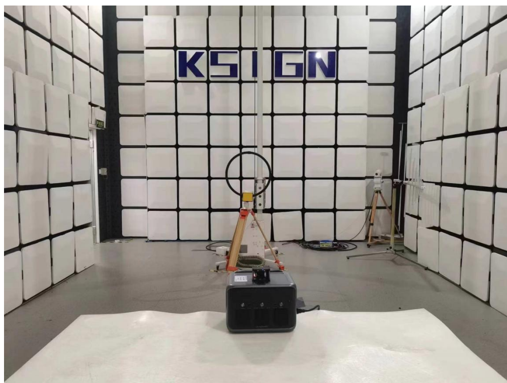
Emissions in frequency bands (30MHz - 1GHz)
