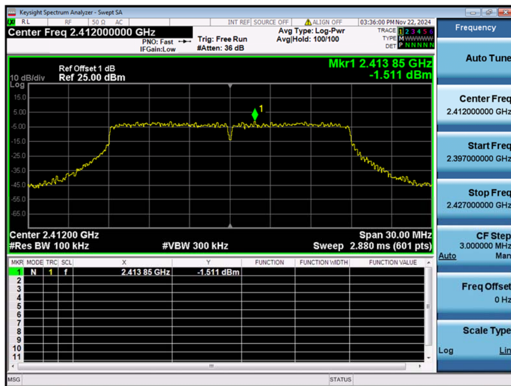
Figure 31: Conducted Spurious Emission & Authorized-band band-edge, 802.11n(HT20), 2412MHz Carrier Level
