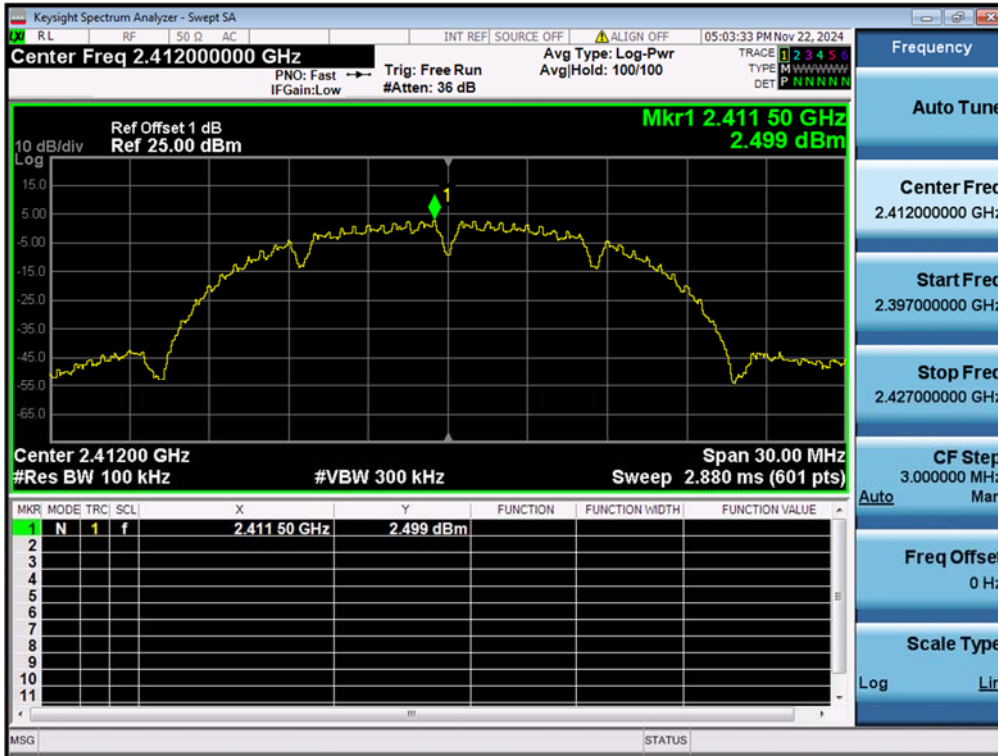
Figure 25: Conducted Spurious Emission & Authorized-band band-edge, 802.11b, 2412MHz Carrier Level
