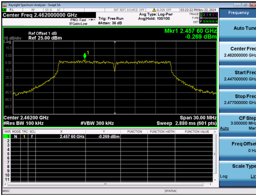
Figure 30: Conducted Spurious Emission & Authorized-band band-edge, 802.11g, 2462MHz Carrier Level
