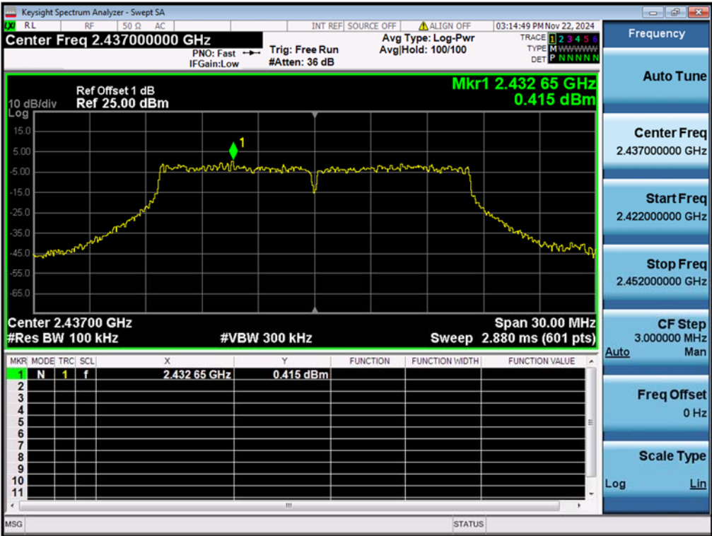
Figure 29: Conducted Spurious Emission & Authorized-band band-edge, 802.11g, 2437MHz Carrier Level
