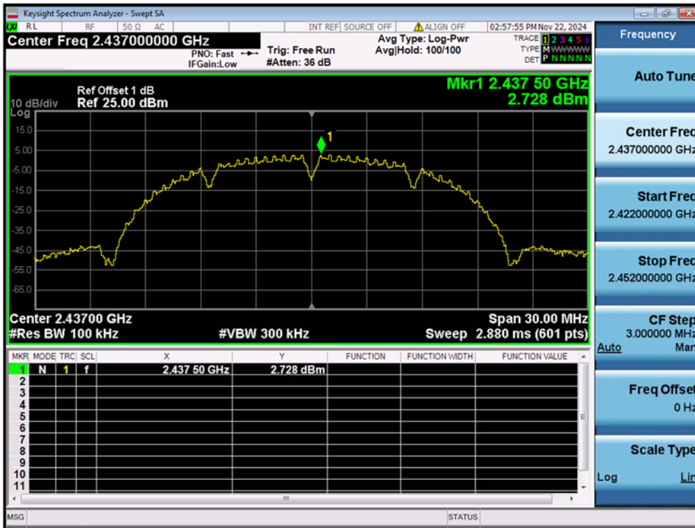
Figure 26: Conducted Spurious Emission & Authorized-band band-edge, 802.11b, 2437MHz Carrier Level
