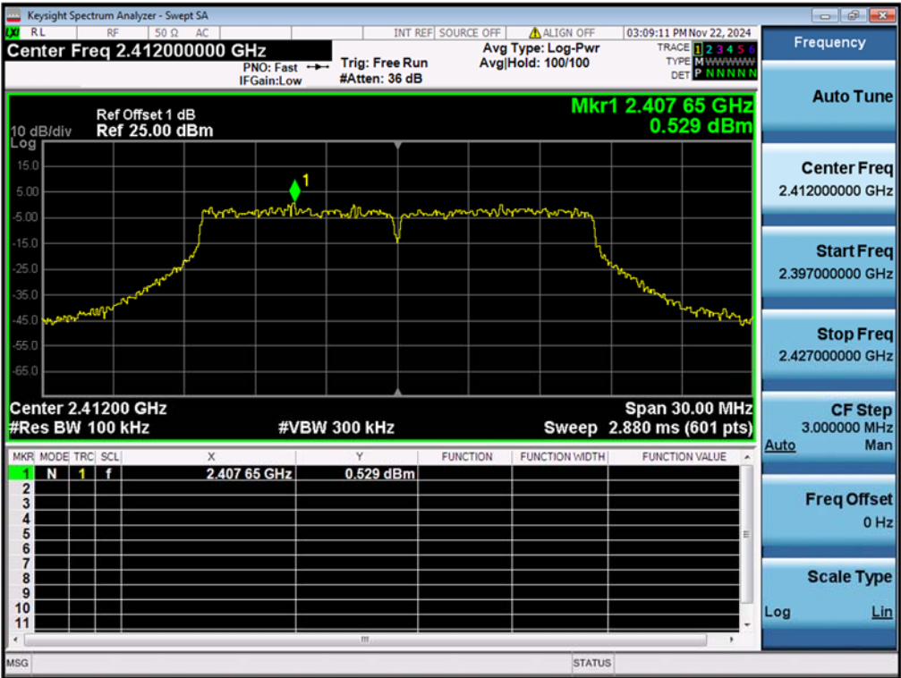
Figure 28: Conducted Spurious Emission & Authorized-band band-edge, 802.11g, 2412MHz Carrier Level
