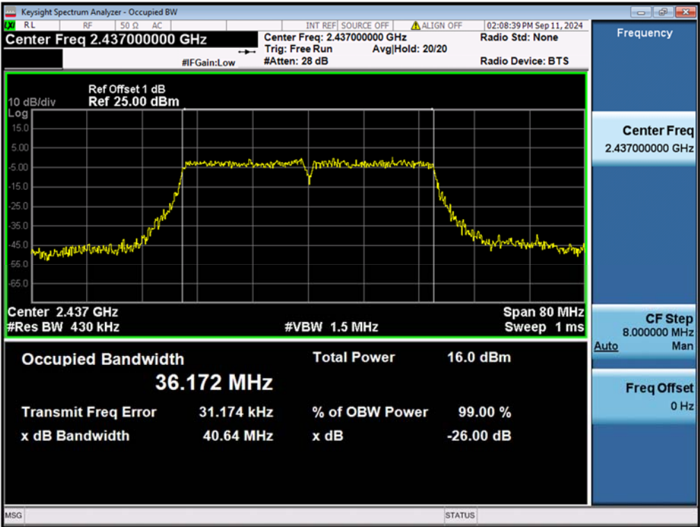
99% Bandwidth, 802.11n(HT40), 2437MHz
