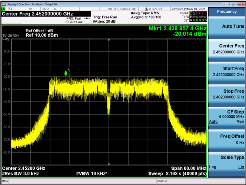
Figure 24: Power Spectral Density, 802.11n(HT40), 2452MHz
