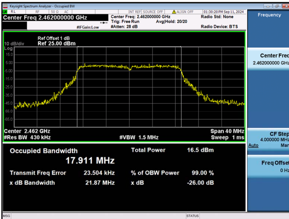
99% Bandwidth, 802.11n(HT20), 2462MHz
