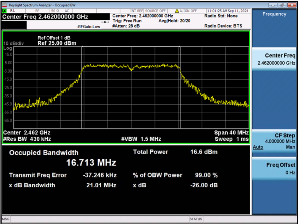
99% Bandwidth, 802.11g, 2462MHz
