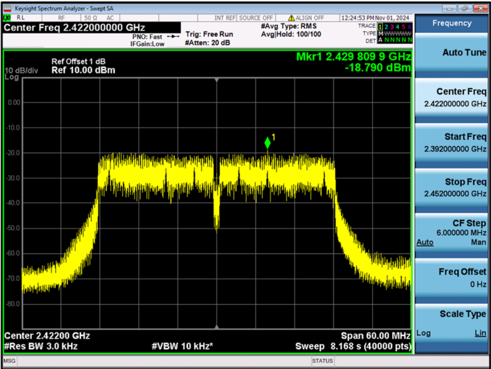
Figure 22: Power Spectral Density, 802.11n(HT40), 2422MHz
