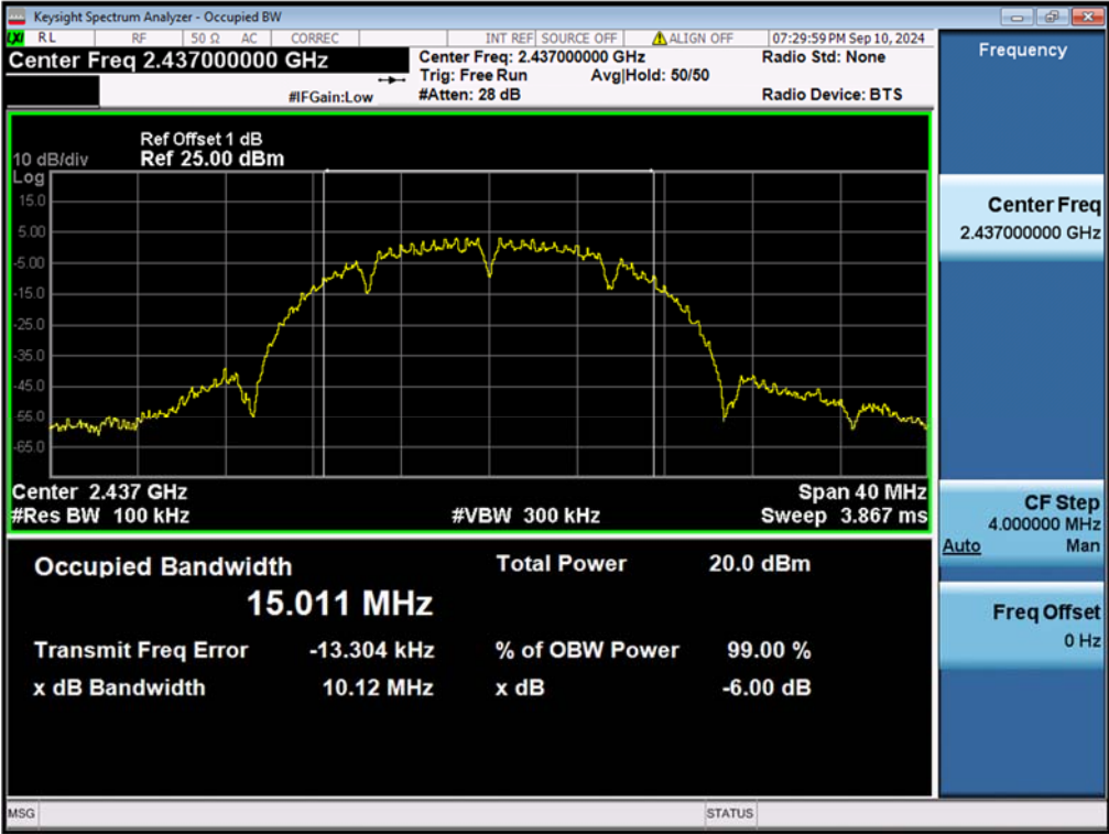
99% Bandwidth, 802.11b, 2437MHz
