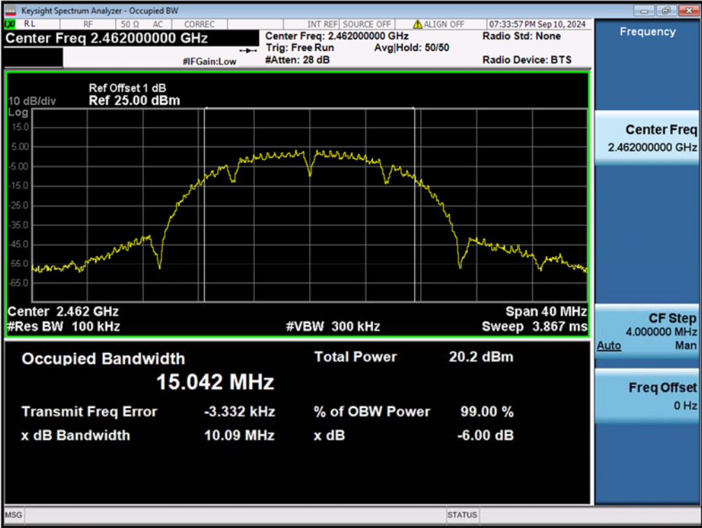
99% Bandwidth, 802.11b, 2462MHz
