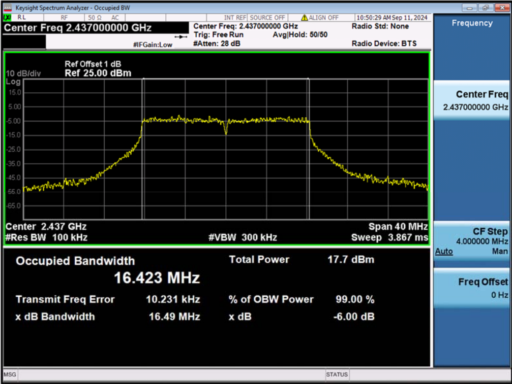
99% Bandwidth, 802.11g, 2437MHz
