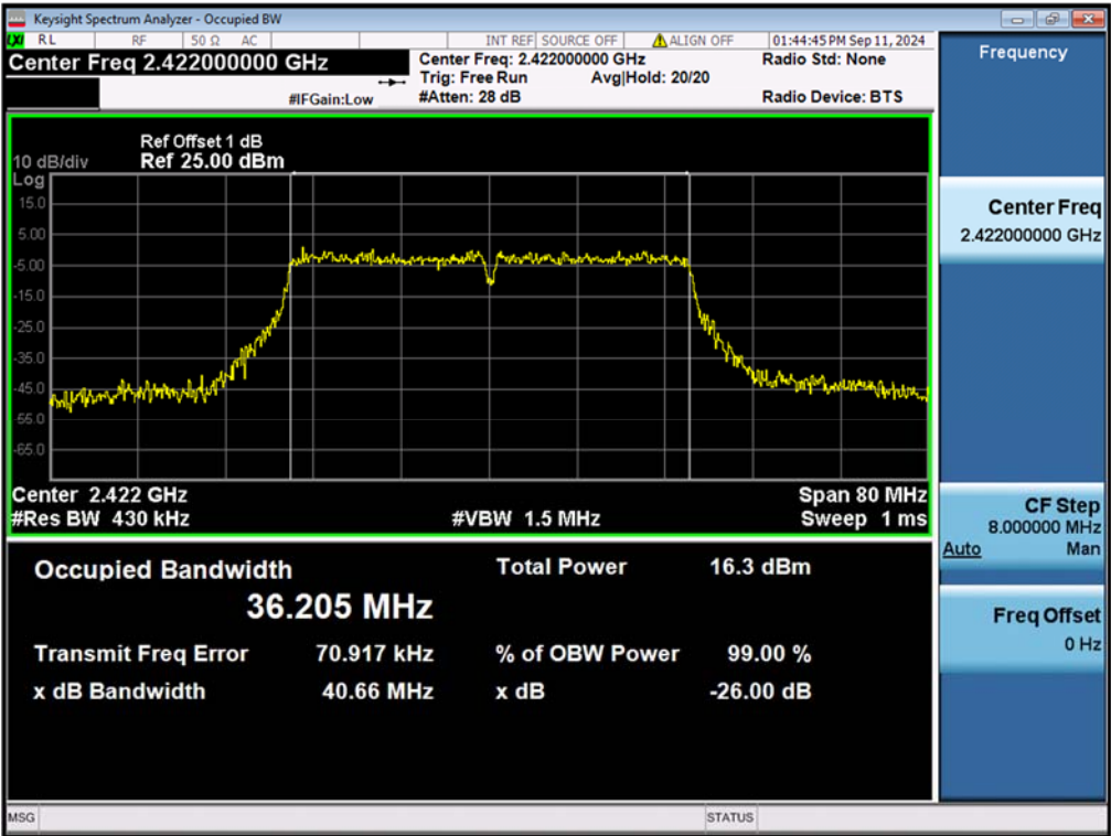
99% Bandwidth, 802.11n(HT40), 2422MHz
