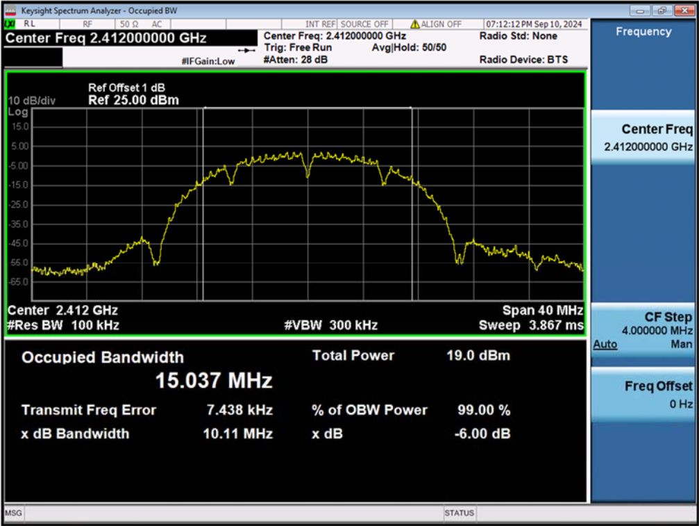
99% Bandwidth, 802.11b, 2412MHz
