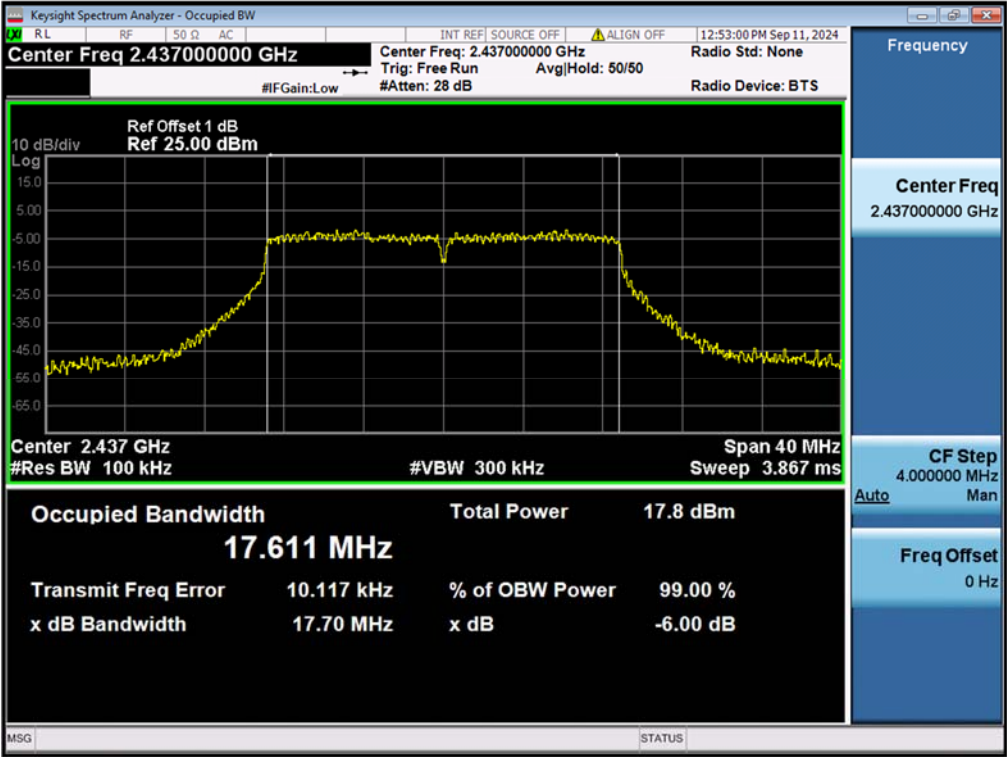
99% Bandwidth, 802.11n(HT20), 2437MHz
