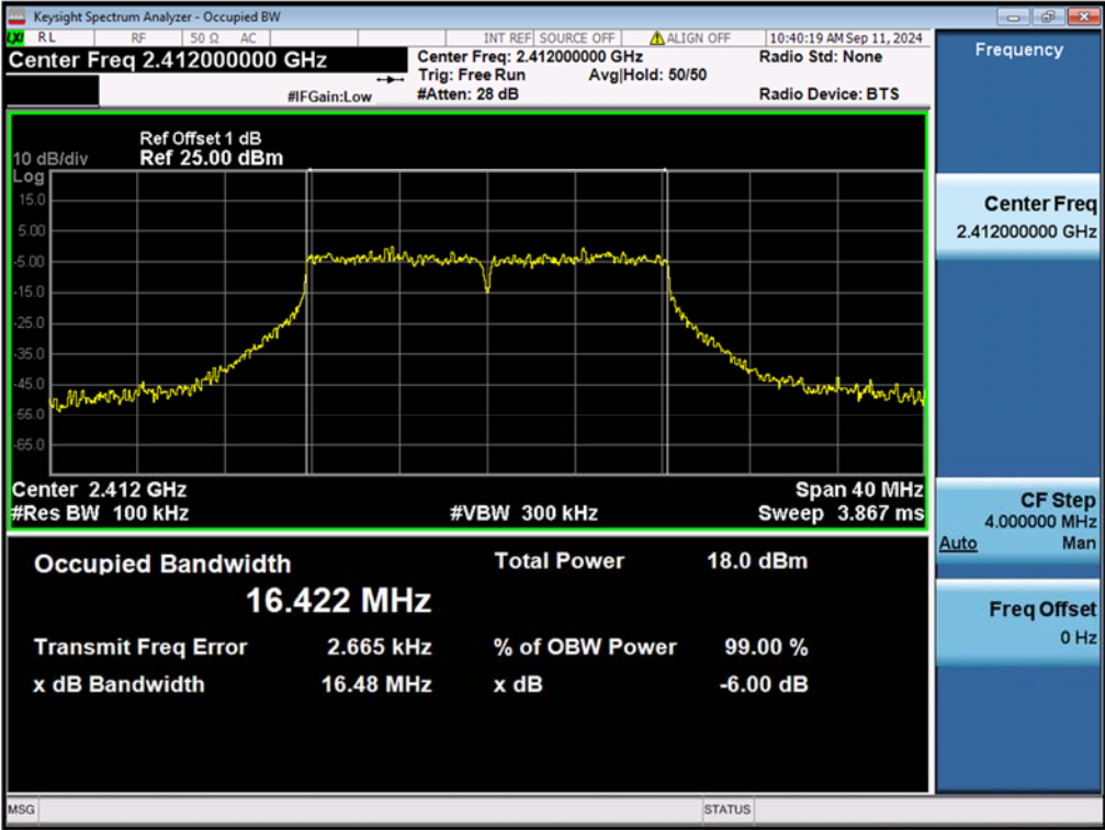
99% Bandwidth, 802.11g, 2412MHz
