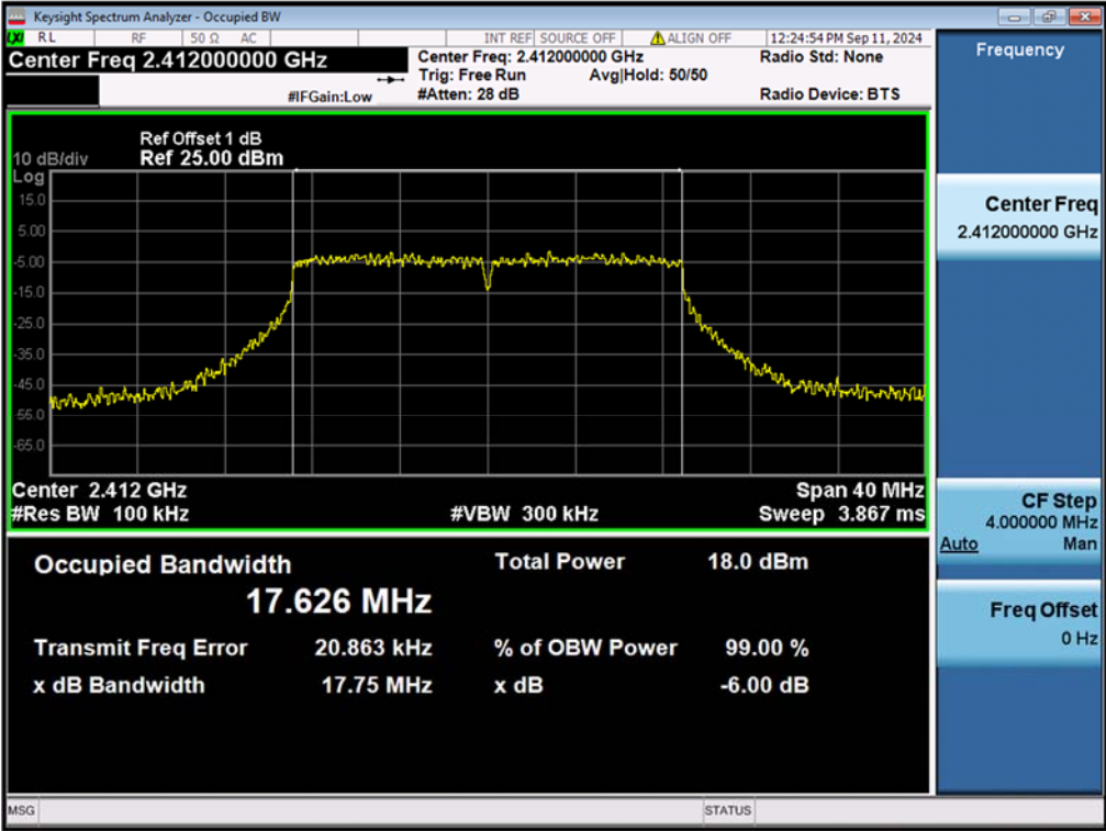
99% Bandwidth, 802.11n(HT20), 2412MHz
