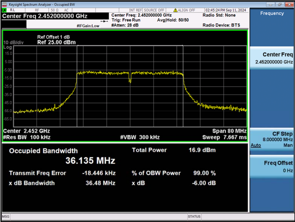
99% Bandwidth, 802.11n(HT40), 2452MHz
