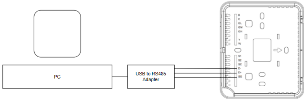
FIGURE 7: RS485 CONNECTION
