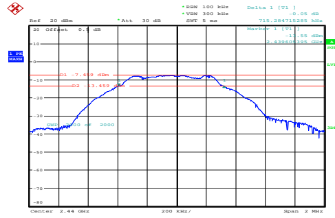
Middle 0.715MHz
