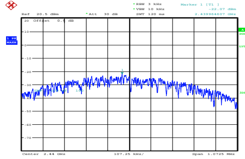
Middle -22.07dBm/3kHz
