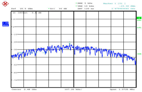
High -23.30dBm/3kHz
