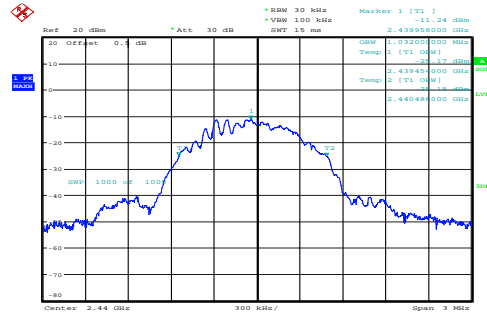
Middle 1.032MHz
