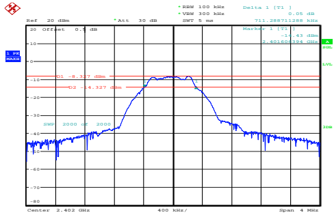
Low 0.711MHz
