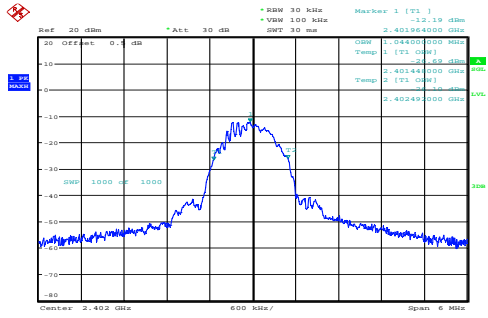
Low 1.044MHz
