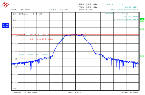
High 0.707MHz
