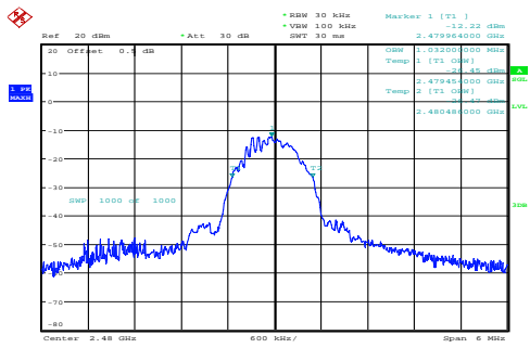
High 1.032MHz
