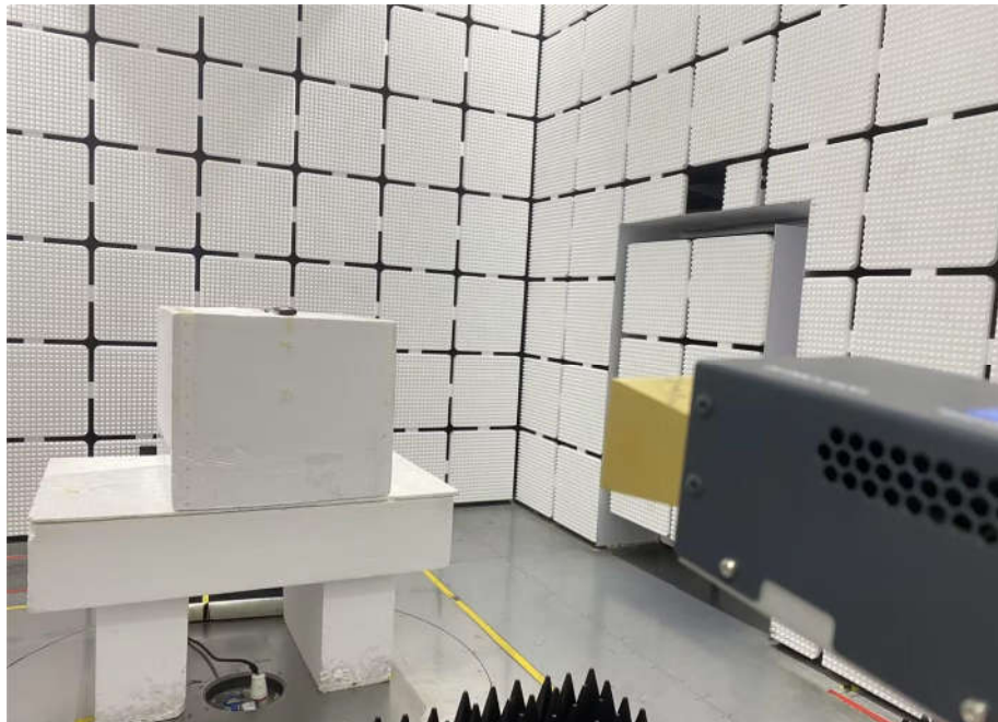
Radiated spurious emission Test Setup-5(Above 41GHz)
