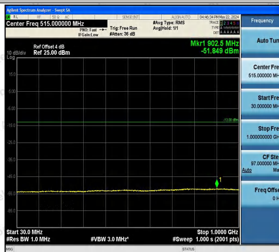
Band2-9262-5-30~1000MHz-PASS
