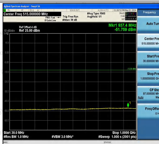
Band2-9262-4-30~1000MHz-PASS
