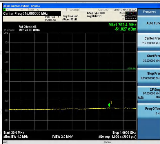
Band2-9262-3-30~1000MHz-PASS
