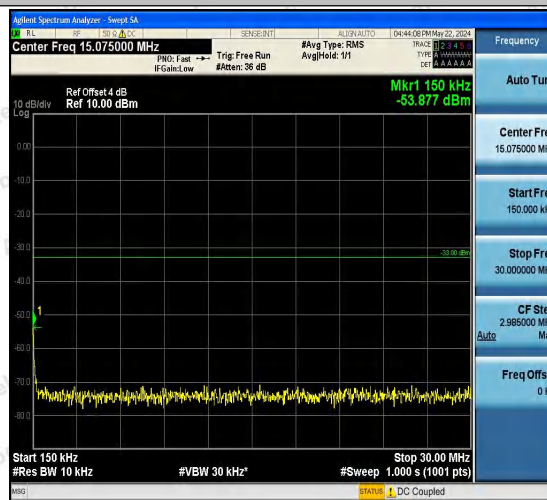
Band2-9400-4-0.15~30MHz-PASS
