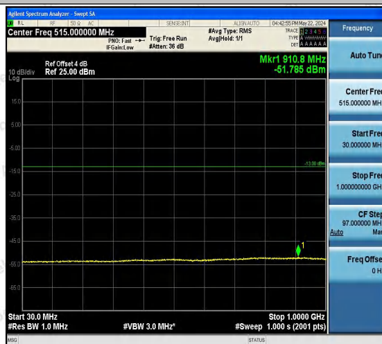
Band2-9262-4-30~1000MHz-PASS
