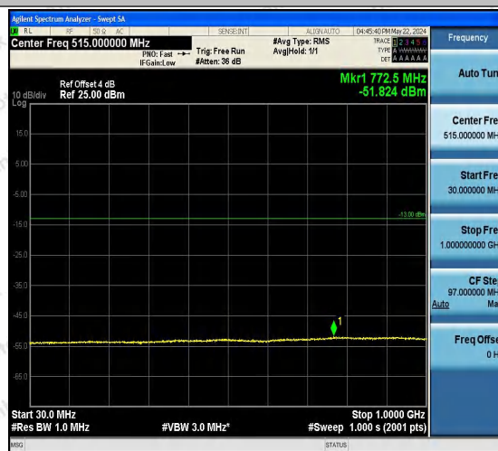
Band2-9538-4-30~1000MHz-PASS
