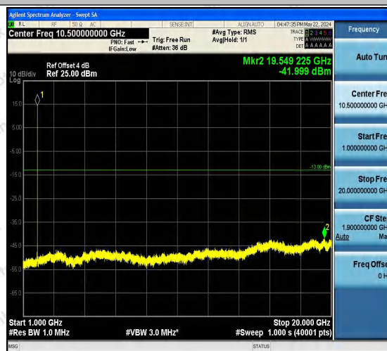
Band2-9400-5-1000~20000MHz-PASS
