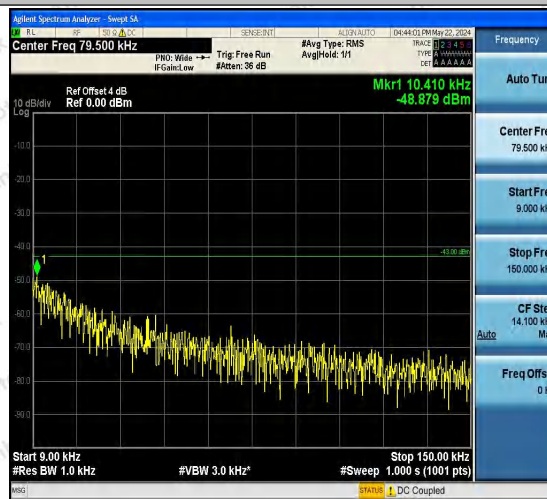
Band2-9400-4-0.009~0.15MHz-PASS
