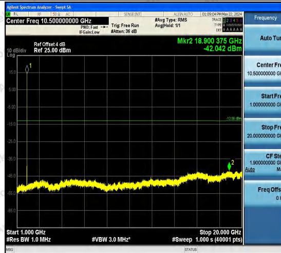
Band2-9262-4-1000~20000MHz-PASS
