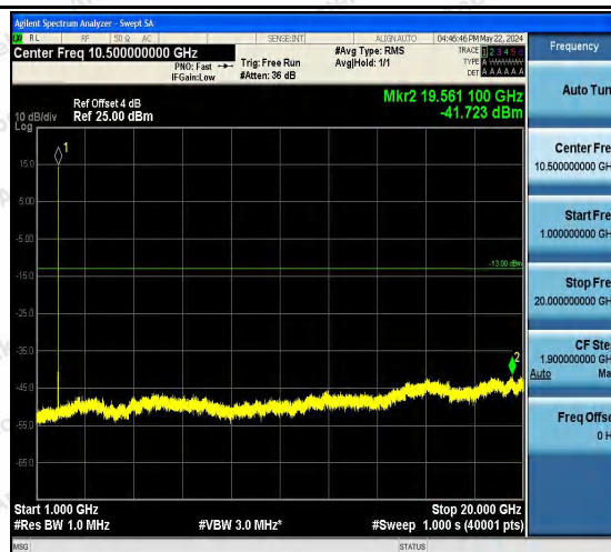
Band2-9262-5-1000~20000MHz-PASS
