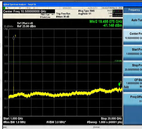
Band2-9262-4-1000~20000MHz-PASS
