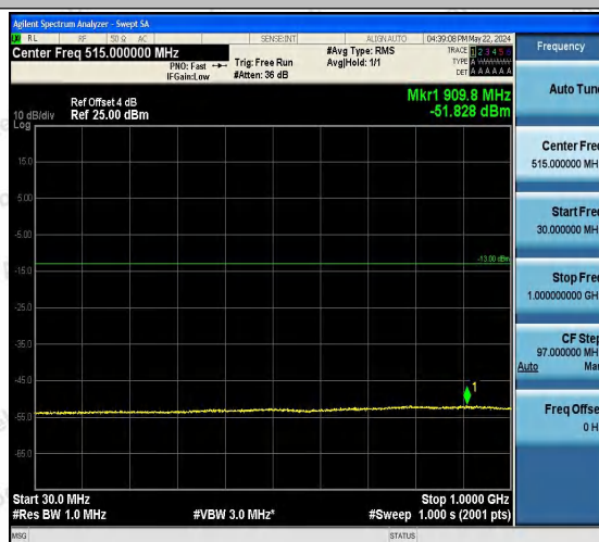
Band2-9262-3-30~1000MHz-PASS
