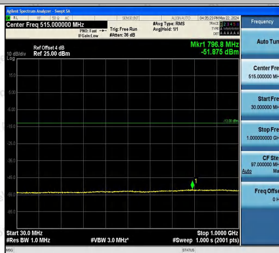
Band2-9262-2-30~1000MHz-PASS
