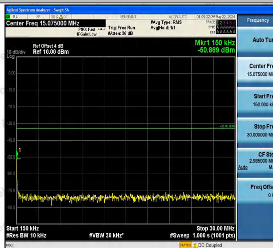
Band2-9400-4-0.15~30MHz-PASS
