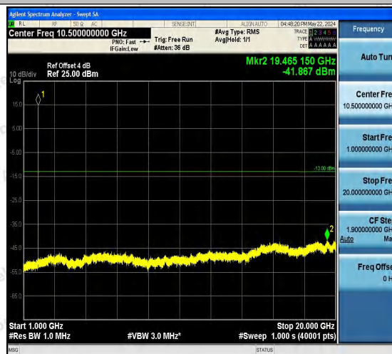
Band2-9538-5-1000~20000MHz-PASS
