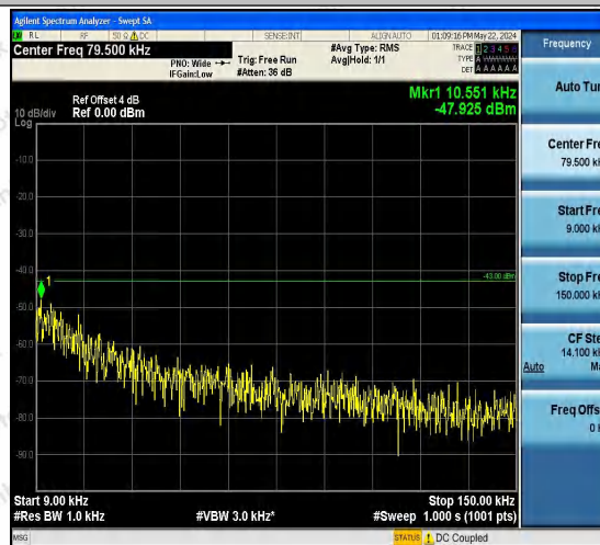
Band2-9400-4-0.009~0.15MHz-PASS
