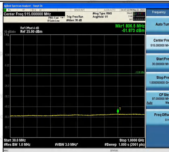
Band2-9400-5-30~1000MHz-PASS
