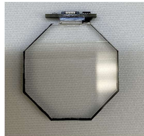
Beamsplitter/display assembly
