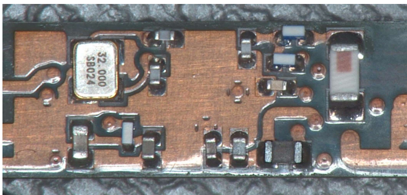
Close up of 2.4GHz ceramic chip antenna
