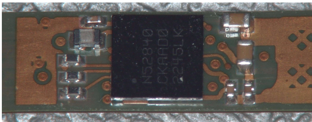
Close up of processor with integrated Bluetooth circuitry
