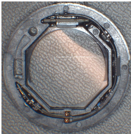
Flex board – display side
