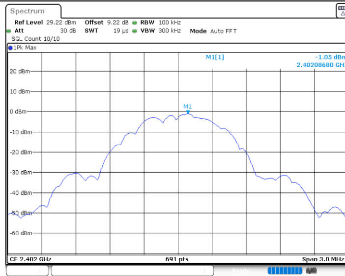
BLE_1M_Ant1_2402_0~Reference
