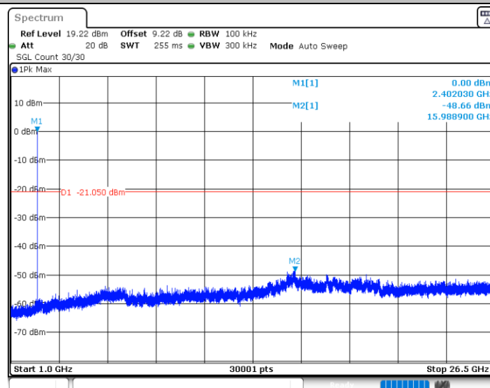
BLE_1M_Ant1_2402_1000~26500
