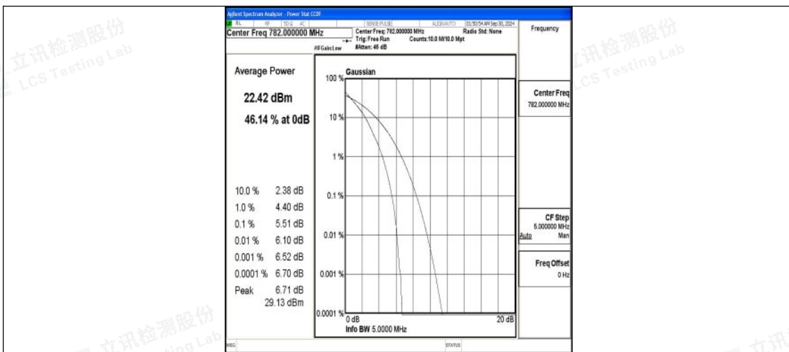
Band13-5MHz-QPSK-23230-25RB#0-PASS
