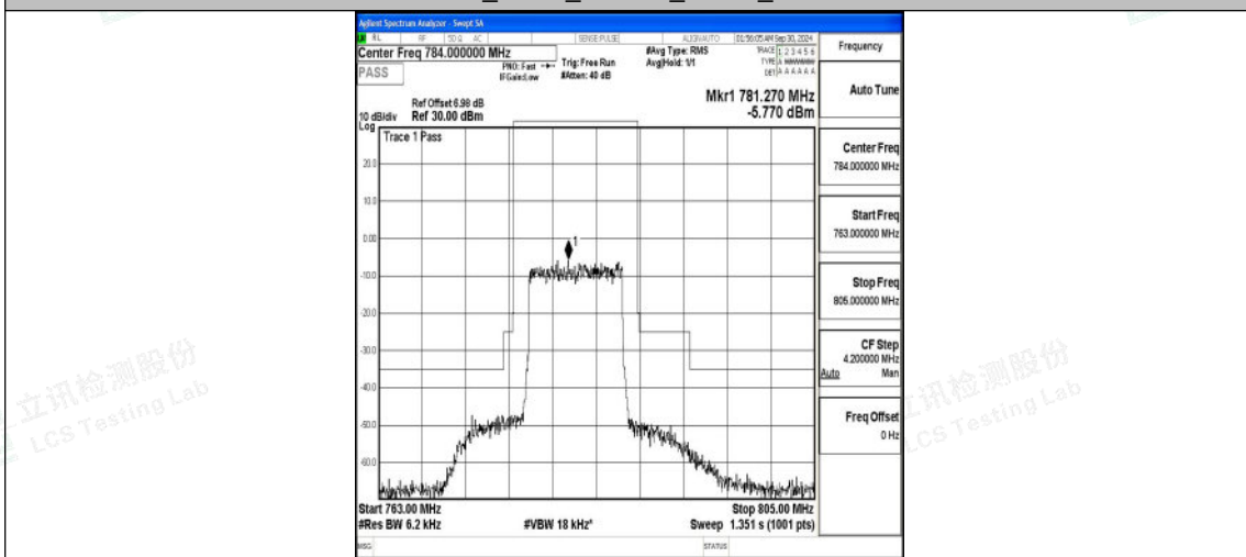
Band13_10MHz_QPSK_23230_50RB#0
