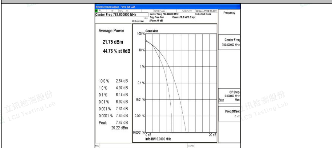
Band13-5MHz-16QAM-23230-25RB#0-PASS
