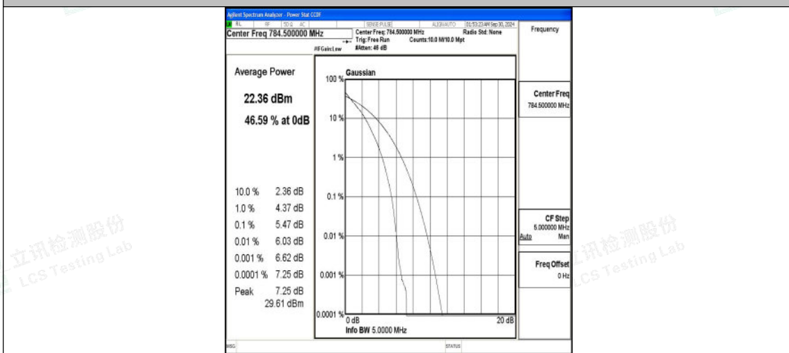
Band13-5MHz-QPSK-23255-25RB#0-PASS
