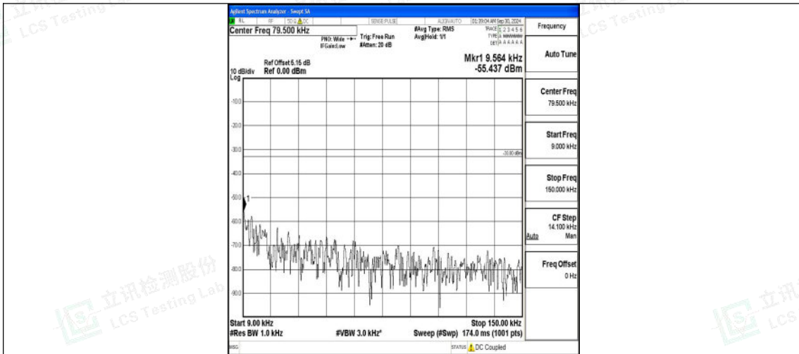
Band13_5MHz_QPSK_23205_1RB#0_0.009~0.15_0.009~0.15
