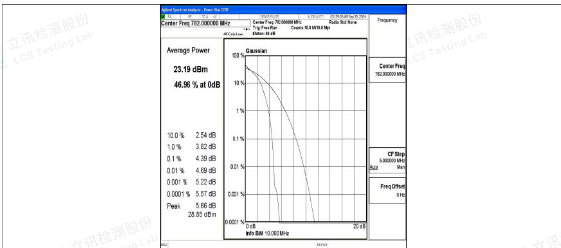
Band13-10MHz-QPSK-23230-1RB#0-PASS
