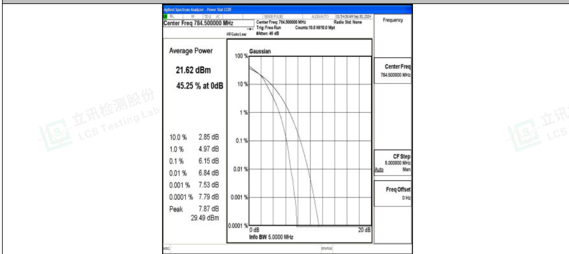
Band13-5MHz-16QAM-23255-25RB#0-PASS
