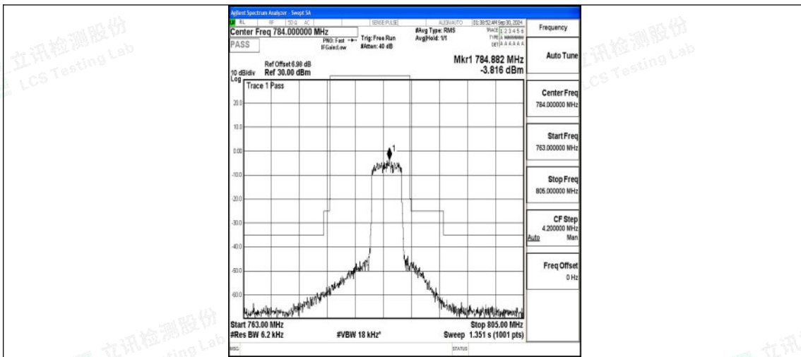
Band13_5MHz_16QAM_23255_25RB#0
