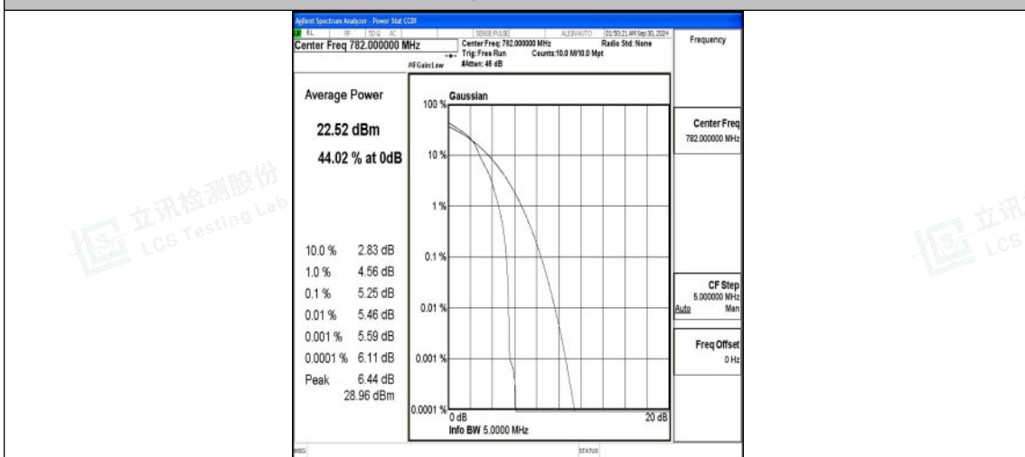
Band13-5MHz-16QAM-23230-1RB#0-PASS
