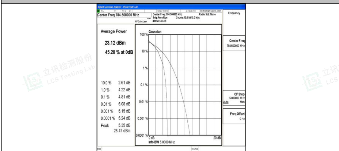
Band13-5MHz-QPSK-23255-1RB#0-PASS
